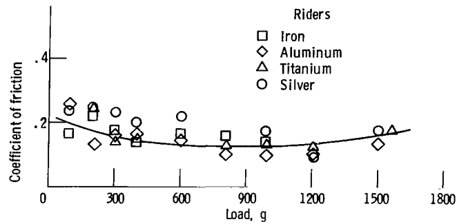
Figure 2. - Coefficient of friction for various riders sliding on iron disk containing thin film of zinc dialkyldithiophosphate. Sliding velocity, 30 centimeters per minute; temperature, 23° C.
