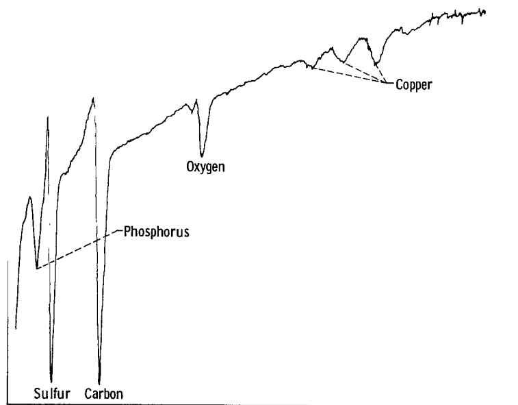
Figure 11. - Auger emission spectrum for copper surface containing thin film of 10 percent zinc dialkyldithiophosphate in hexane.
