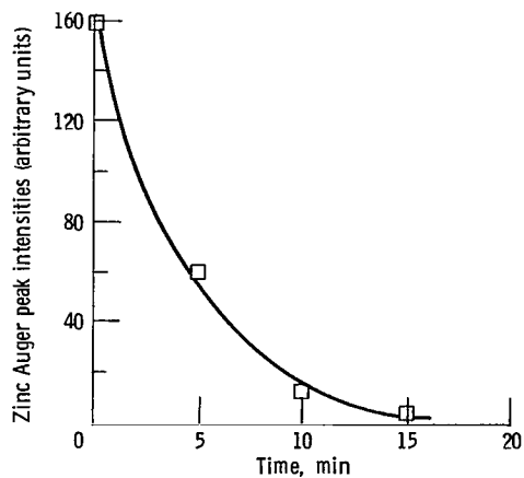
Figure 8. - Electron beam induced desorption of zinc from tungsten disk wear track. Rider, aluminum; load, 300 grams; temperature, 23 o C; Auger electron beam, 10 microamperes and 1360 volts; lubricant, thin film of 10 percent zinc dialkyldithiophosphate in hexane.
