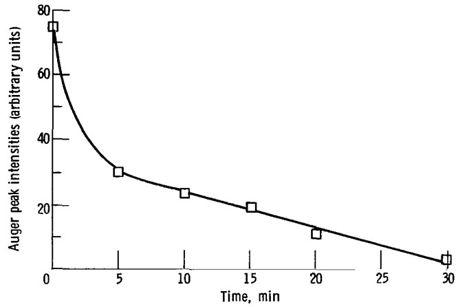
Figure 9. - Auger electron beam induced desorption of zinc from wear track on molybdenum disk. Source of zinc, 10 percent dialkyldithiophosphate thin film on disk surface. Rider, aluminum; load, 1600 grams; sliding velocity, 30 centimeters per minute; temperature, 23 o C.
