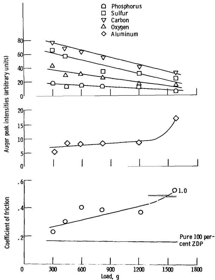
Figure 4. - Friction and Auger spectroscopy data for aluminum sliding on iron with thin film of 10 percent zinc dialkyldithiophosphate (ZDP) in hexane. Sliding velocity, 30 centimeters per minute; temperature, 23° C.
