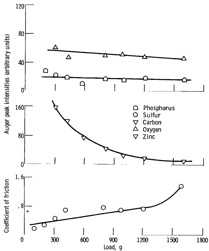
Figure 7. - Friction and Auger spectroscopy data for aluminum sliding on tungsten with thin film of 10 percent zinc dialkyldithiophosphate in hexane. Sliding velocity, 30 centimeters per minute, temperature, 23 o C.
