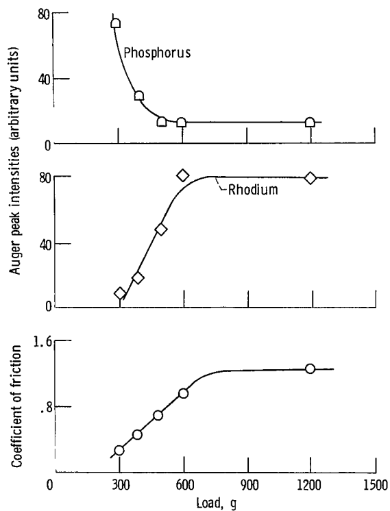
Figure 5. - Friction and Auger spectroscopy data for aluminum sliding on rhodium with thin film of 10 percent zinc dialkyldithiophosphate in hexane. Sliding velocity, 30 centimeters per minute, temperature, 23 o C.
