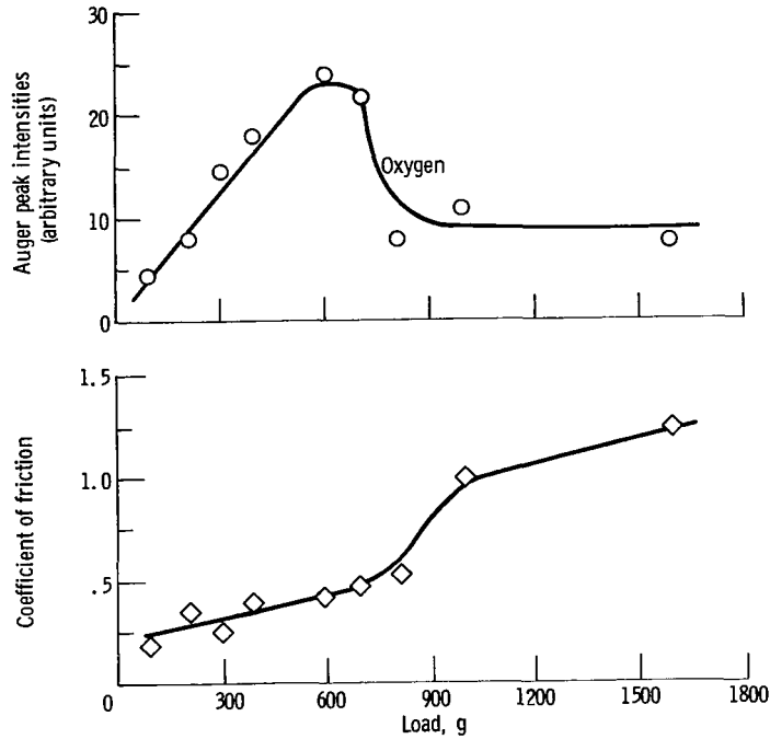
Figure 10. - Coefficient of friction and oxygen Auger peak intensity for aluminum rider sliding on molybdenum disk containing thin film of zinc dialkyldithiophosphate. Sliding velocity, 30 centimeters per minute; temperature, 23 o C.
