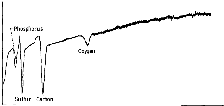
Figure 3. - Auger emission spectrum for iron disk surface containing thin film of 10 percent zinc dialkyldithiophosphate in hexane.
