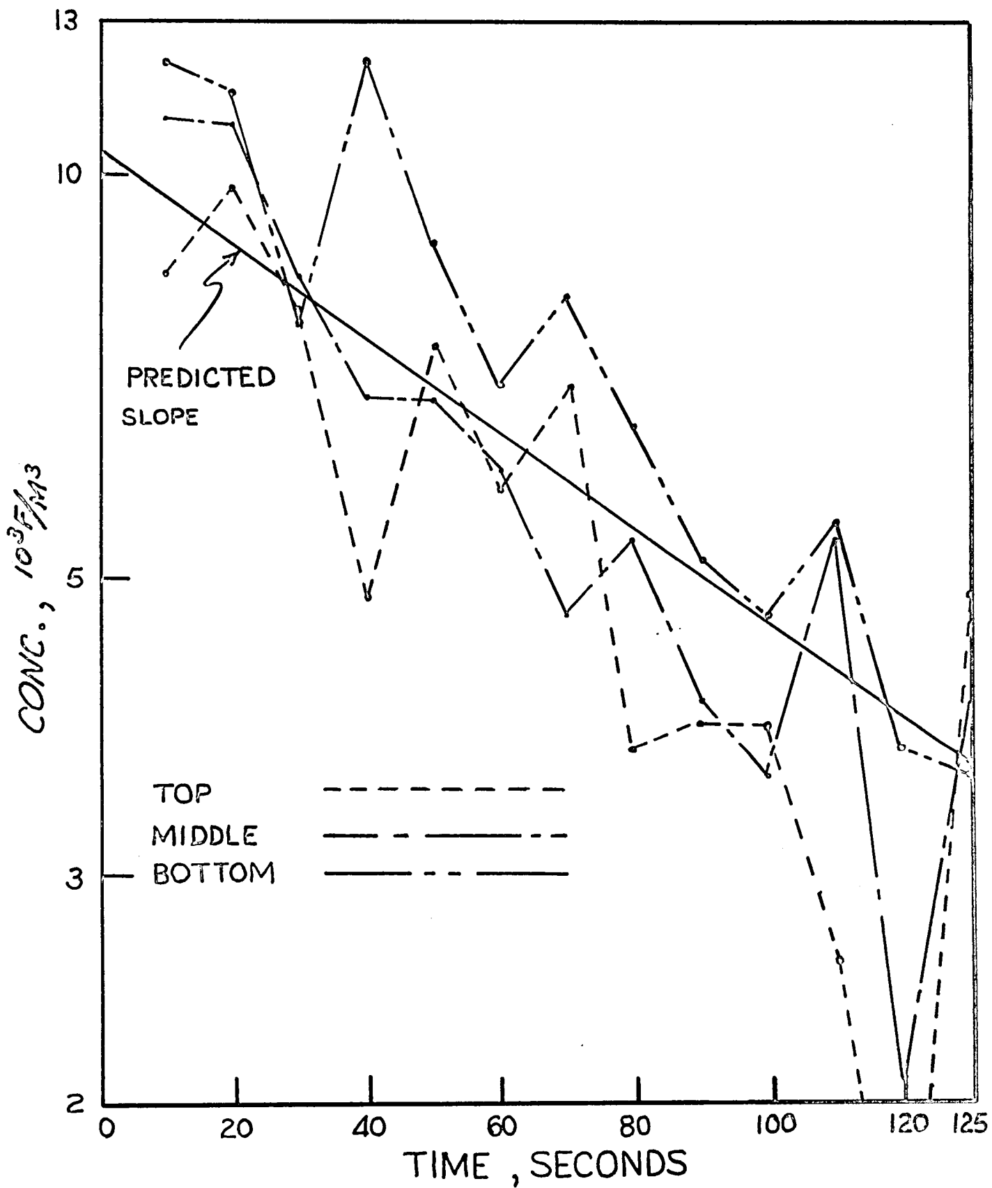
FIGURE 2 Initial Decay for 0.12 m/s Turbulence
