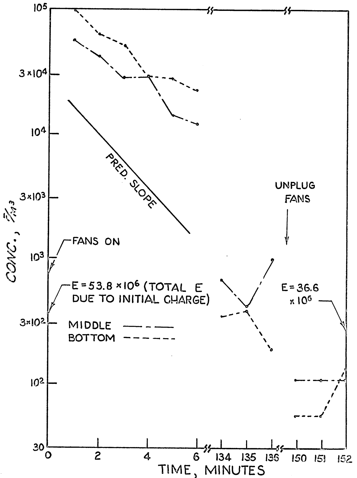
FIGURE B-1 Effects of First Fan-Induced Redissemination
