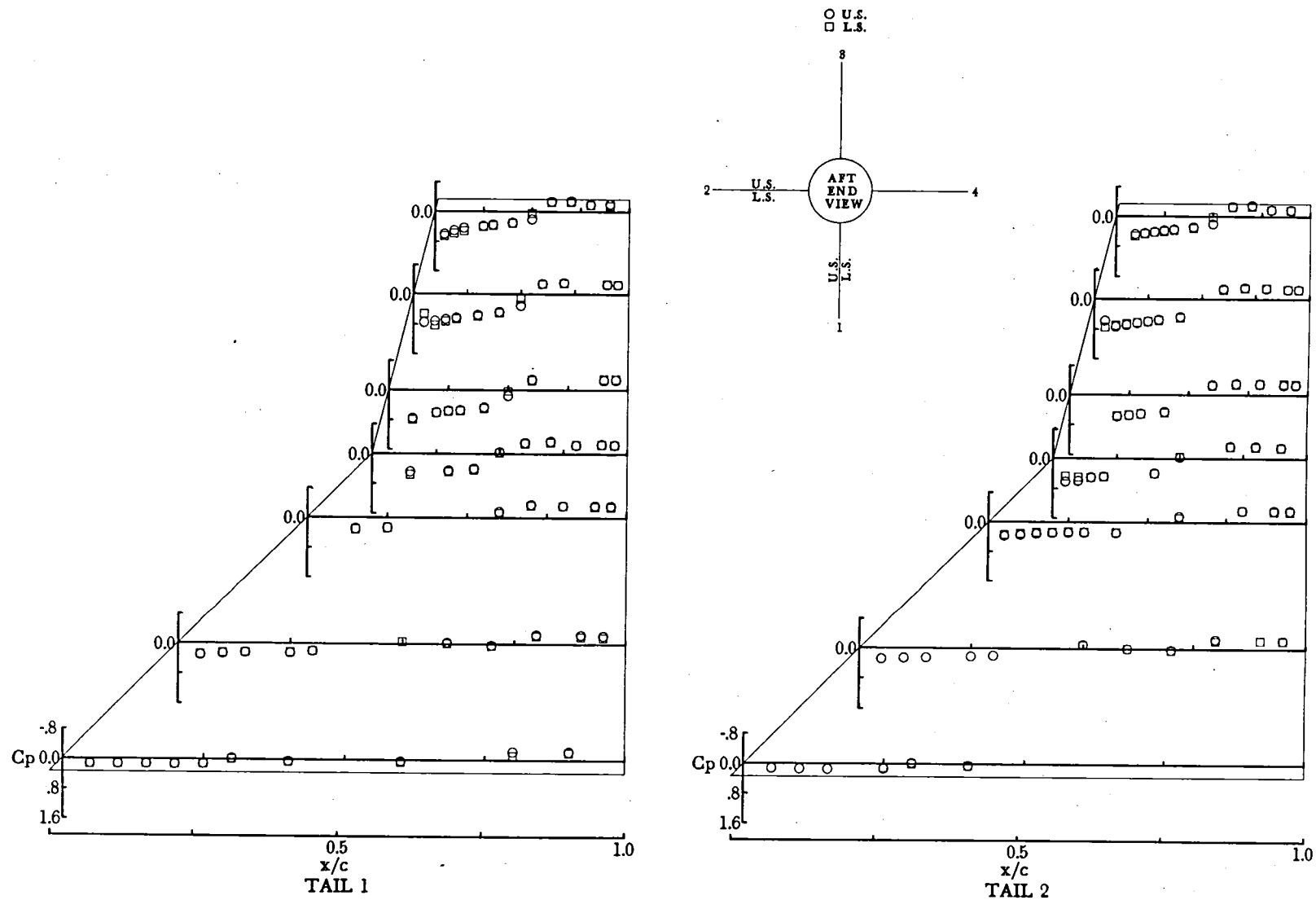
Figure 3.- Pressure coefficients for tail planform C at M = 1.60 , \phi = 0^\circ , and \delta = 0^\circ .
