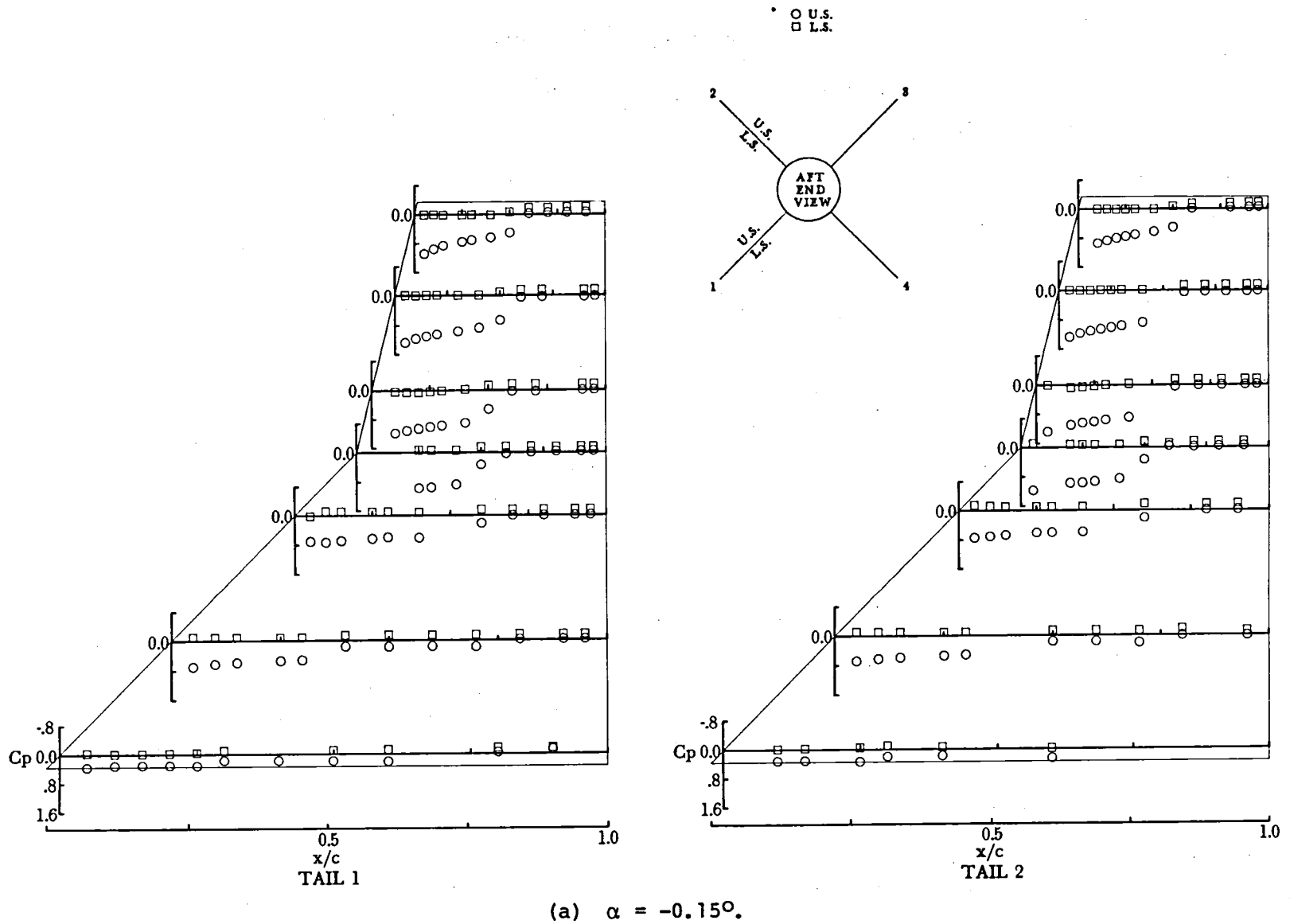
Figure 22.- Pressure coefficients for tail planform C at M = 2.36 , \phi = 45^\circ , and \delta = -15^\circ .
