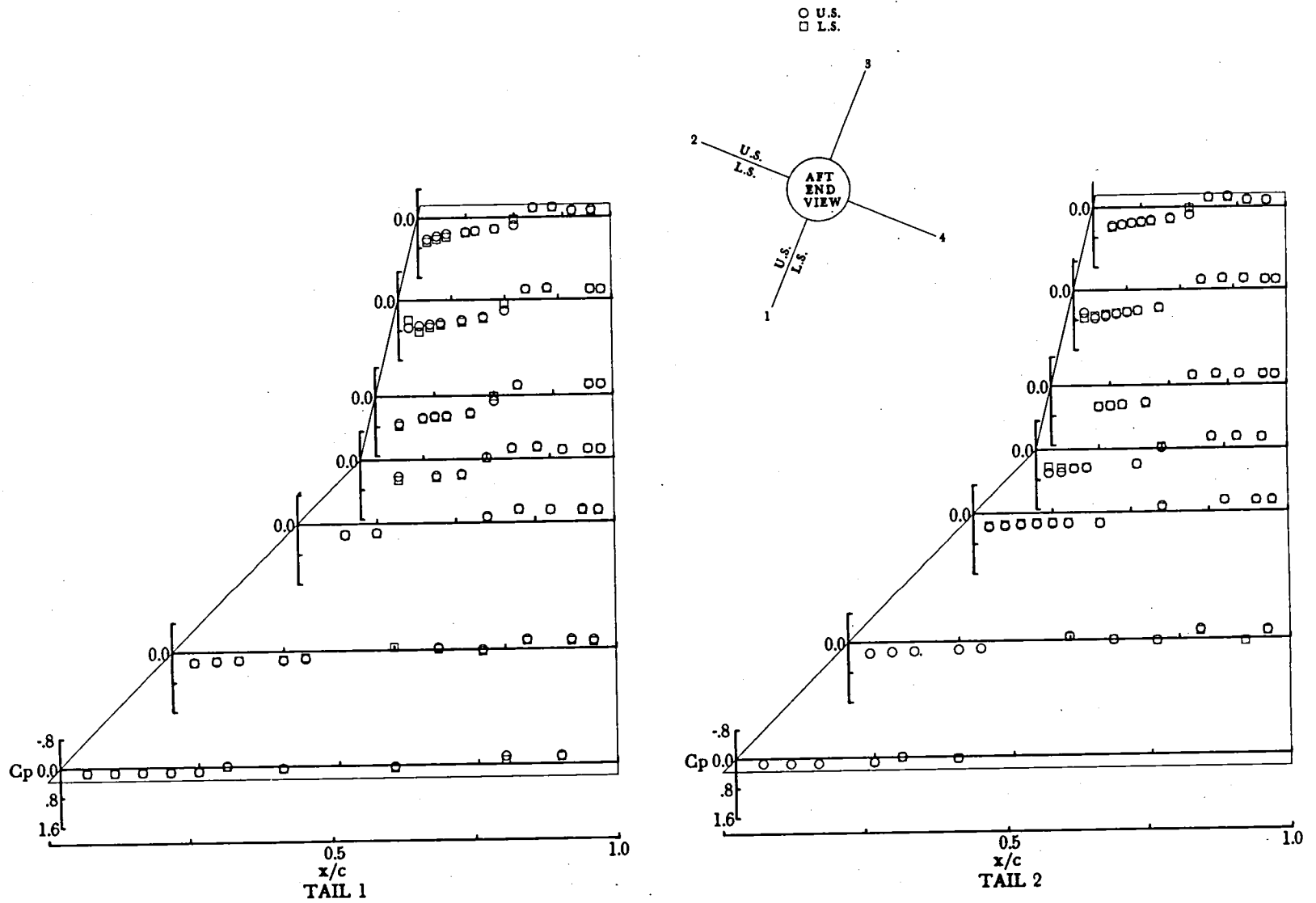
Figure 6.- Pressure coefficients for tail planform C at M = 1.60 , \phi = 22.5^\circ , and \delta = 0^\circ .
