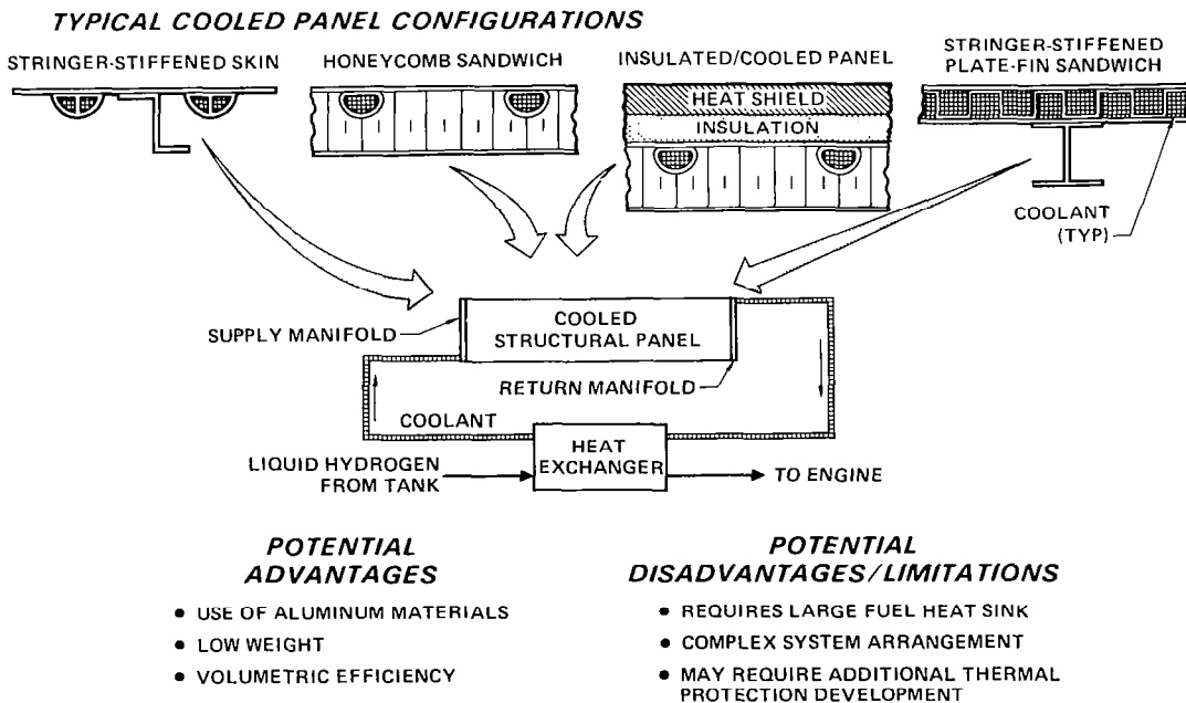
FIGURE 6 ACTIVELY COOLED STRUCTURE
