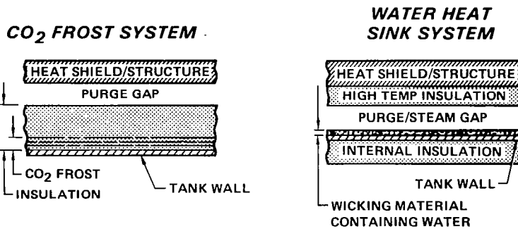
FIGURE 13 LH 2 . LAYERED EXTERNAL INSULATION, TPS CONCEPT
