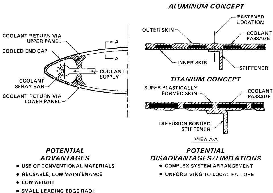
FIGURE 10 ACTIVELY COOLED STRUCTURE - LEADING EDGE
