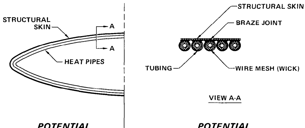
FIGURE 8 EXTERNALLY INSULATED STRUCTURE - LEADING EDGE
