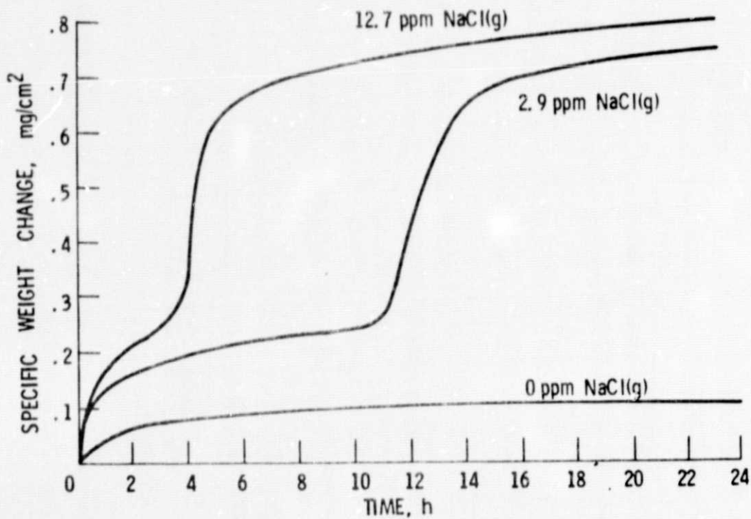
Figure 13. Oxidation of Ni-25Cr at 900°C in air and in air with NaCl(g) added. (From Refs. 33 and 34).
