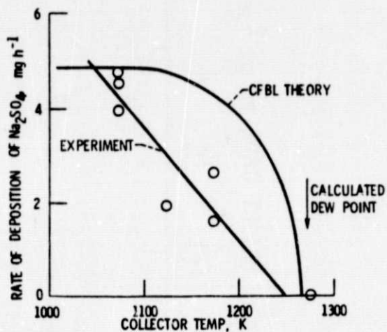
Figure 7. Comparison of experimental and calculated theoretical deposition rates of \text{Na}_2\text{SO}_4 from burner rig flame seeded with 8.0 wppm NaCl in the air and 0.25 wt. % sulfur in the fuel.
