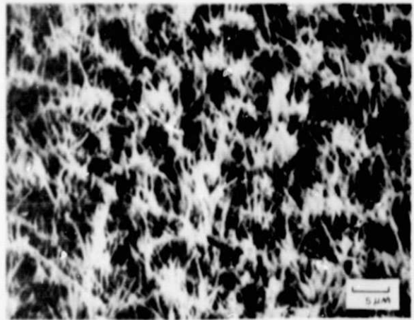
NiAl OXIDIZED WITH 10 ppm NaCl VAPOR PRESENT
