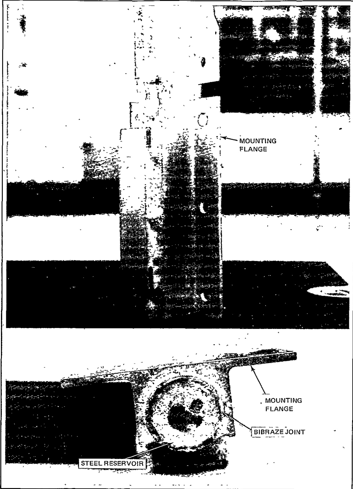
Fig. 3-7 Reservoir Assembly
