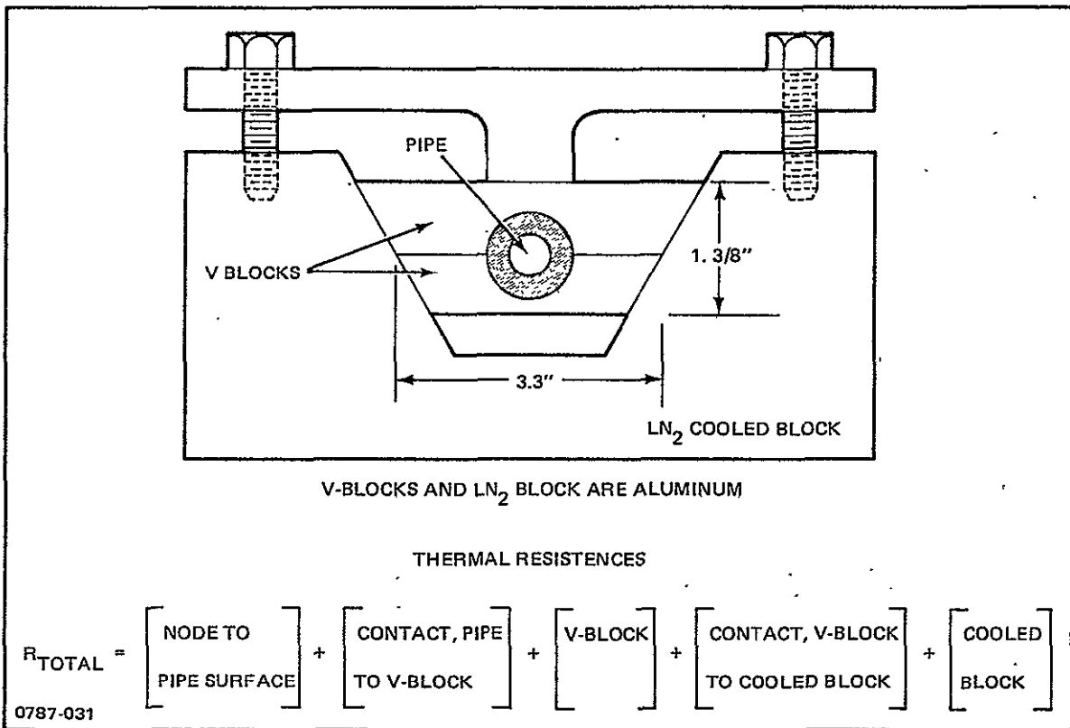
Fig. 6-5 Condenser Cooling Block Schematic
