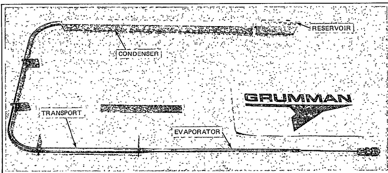
Fig. 3-6 Spiral Artery Liquid Blockage Cryogenic Thermal Diode for HEPP
