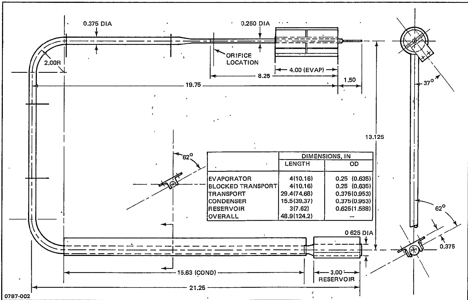
Fig. 3-2 Overall Design Layout for HEPP Liquid Blockage Cryodiode Heat Pipe
