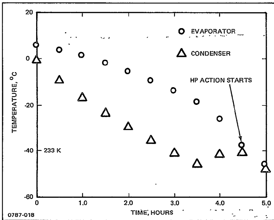
Fig. 3-18 Diode Start-up Behavior During Post-Vibration Testing (1 W on Evaporator)
