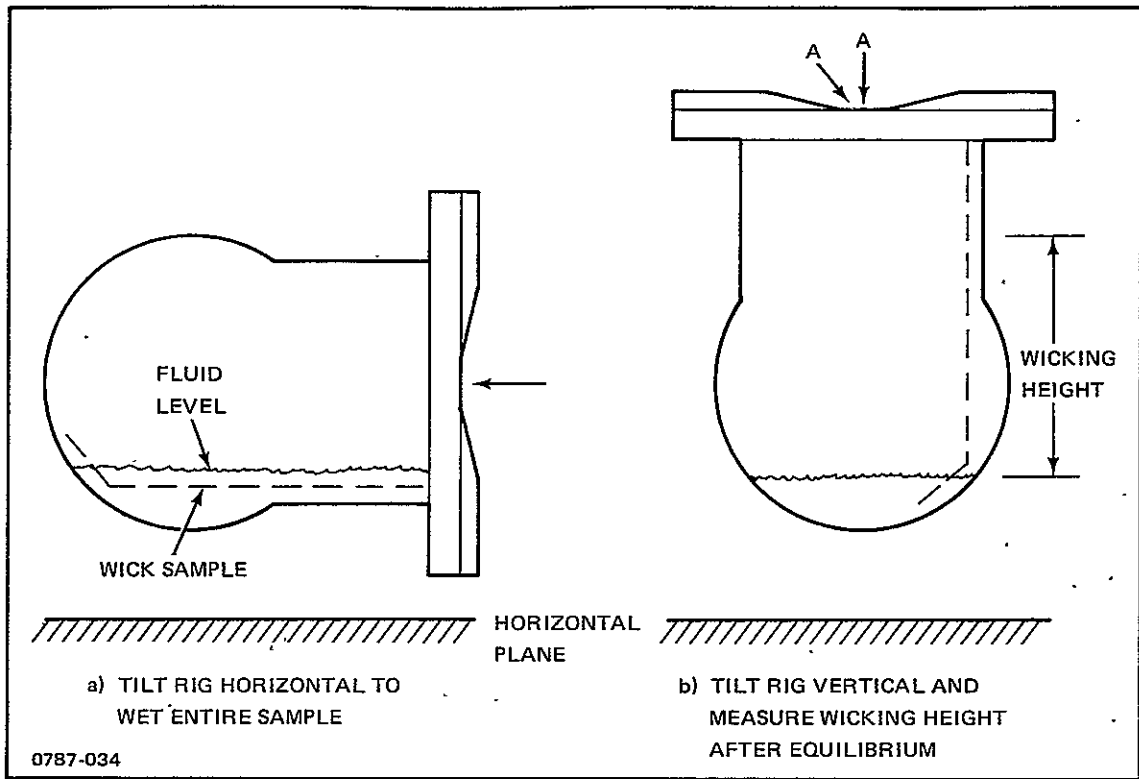
Fig. 6-8 Test Procedure
