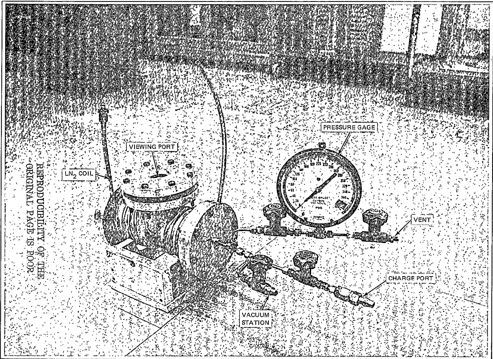
Fig. 6-7 Wettability Apparatus
