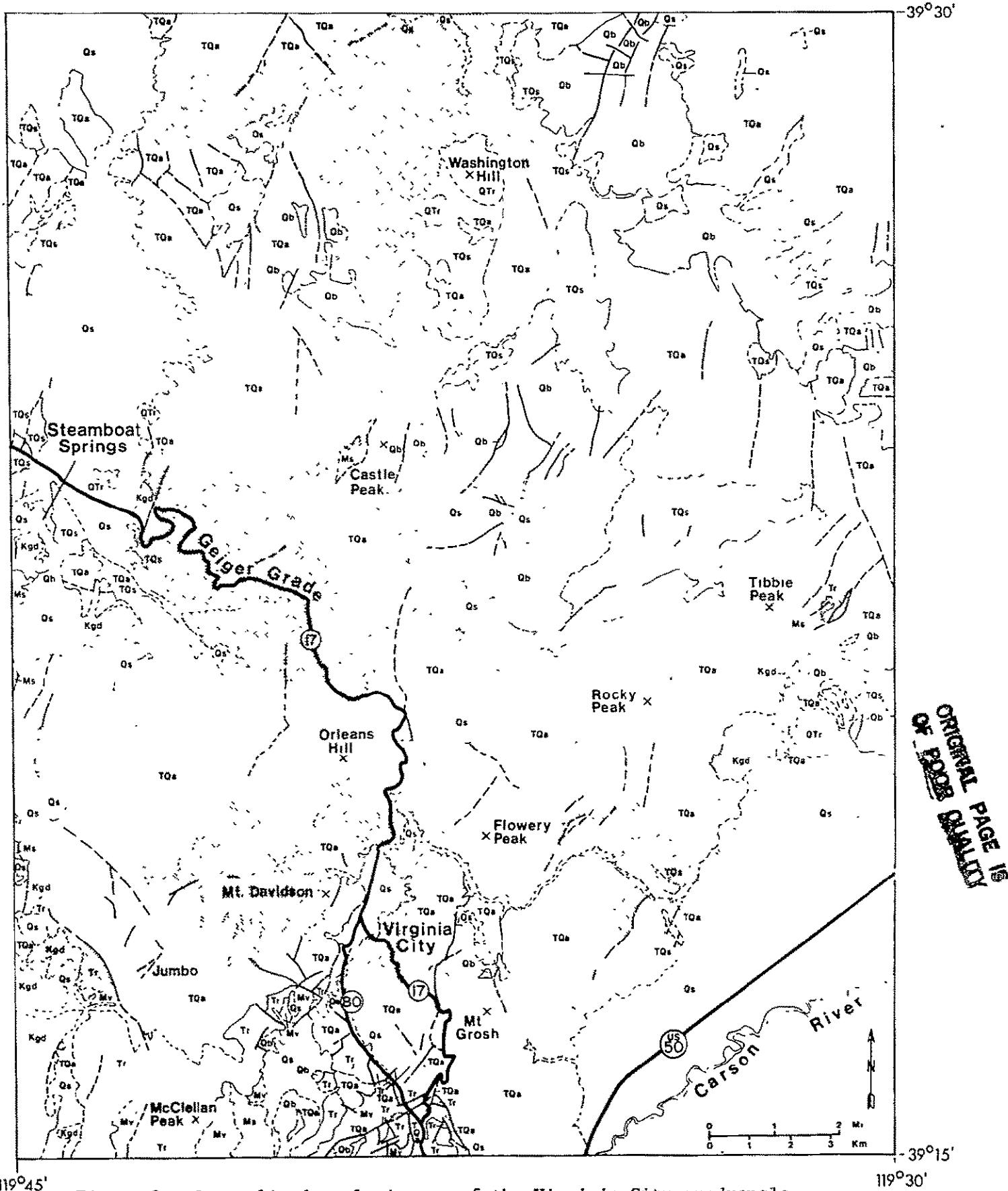
Figure 2. Generalized geologic map of the Virginia City quadrangle, Nevada, modified from Thompson (1956). Mapped hydrothermally altered areas are pattered.
