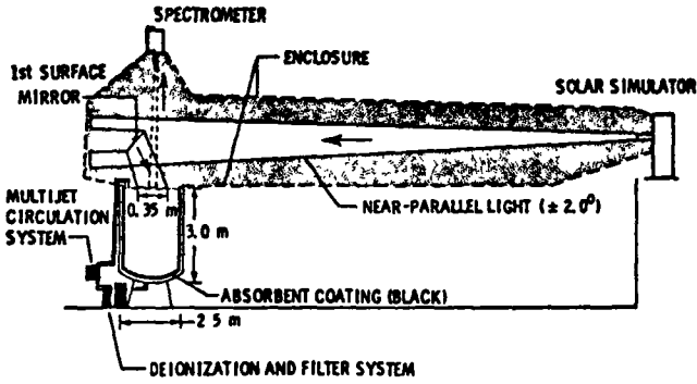
Figure 1. - Laboratory setup.
