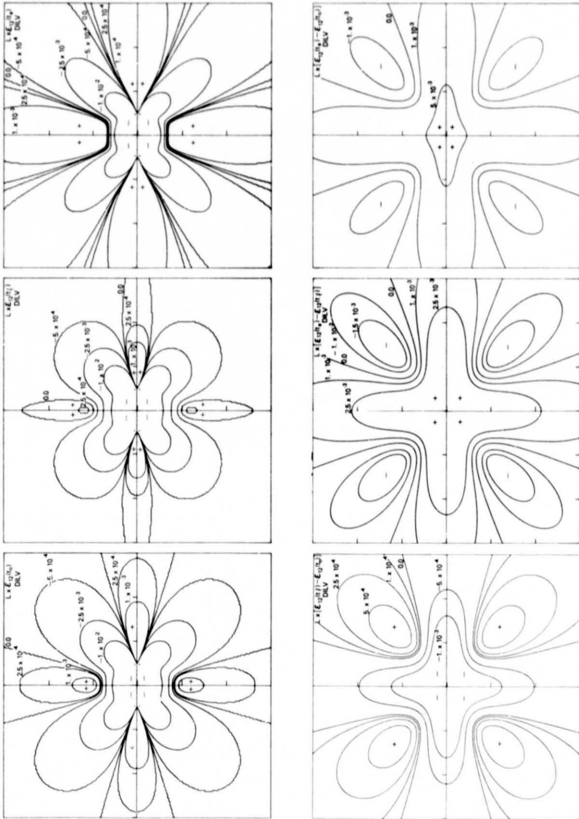
Figure 11. Shear Strain, \epsilon_{12}(t) , for Model DILV; u_0 = 1 m.
