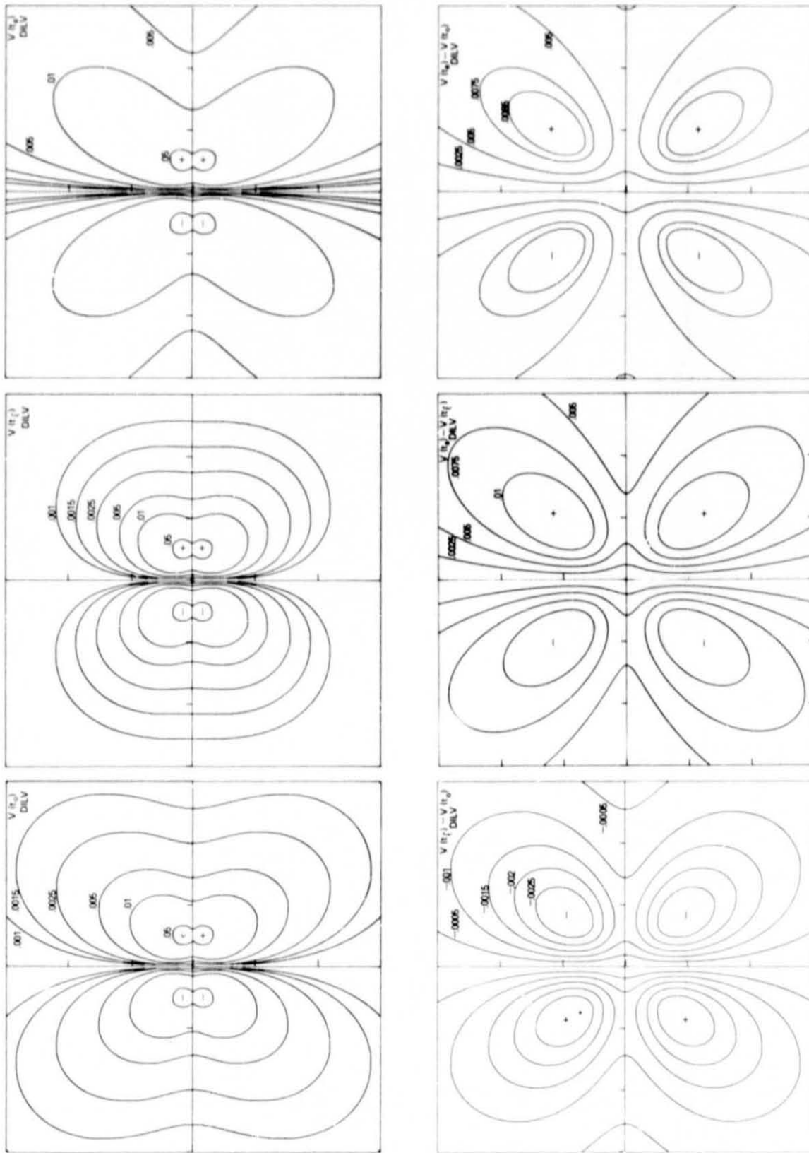
Figure 10. Displacements Perpendicular to the Fault, v(t) , for Model DILV; u_0 = 1 m.
