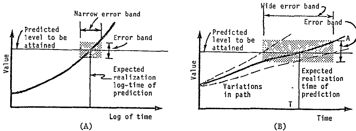
Figure 1.1 - Prediction Band
