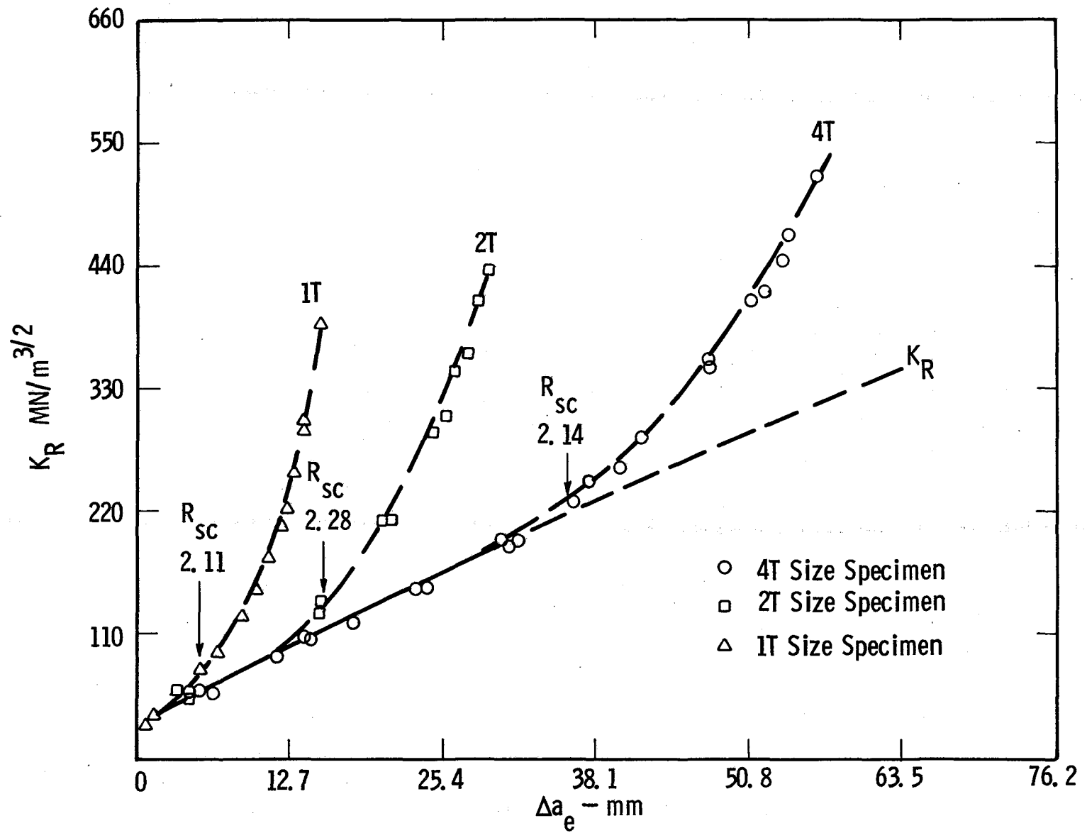
Fig. 6 - 304 Stainless
