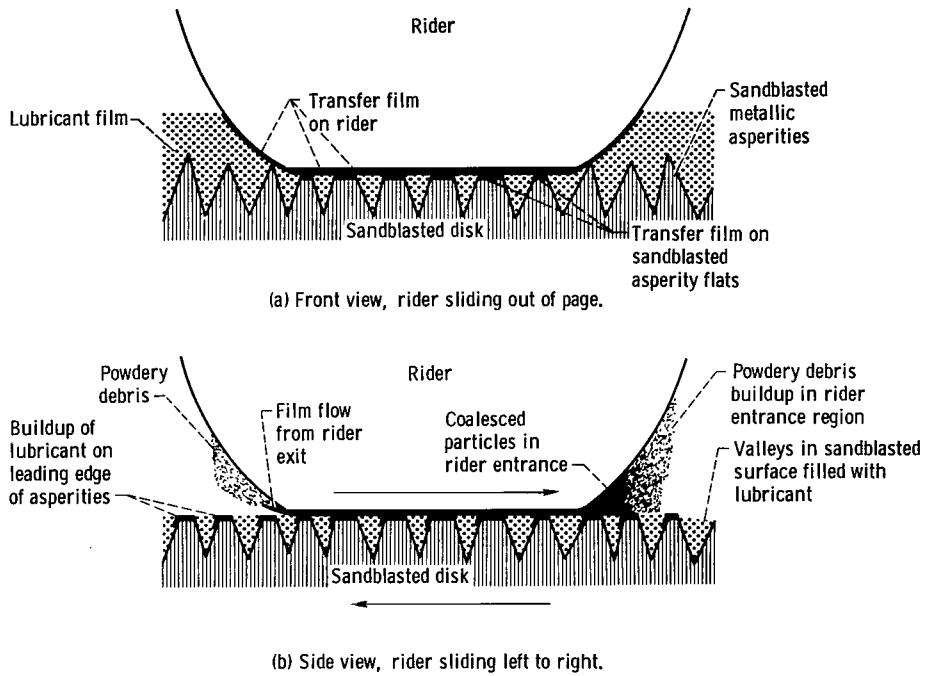
Figure 15. - Idealized schematic drawing of sliding surfaces, illustrating lubricating mechanism in the second lubrication regime.
