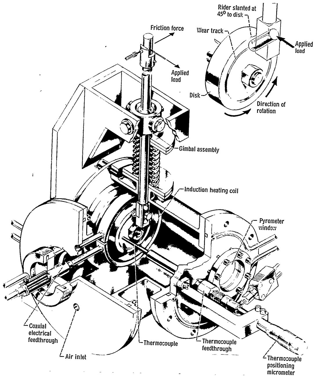
Figure 1. - Friction and wear testing device.
