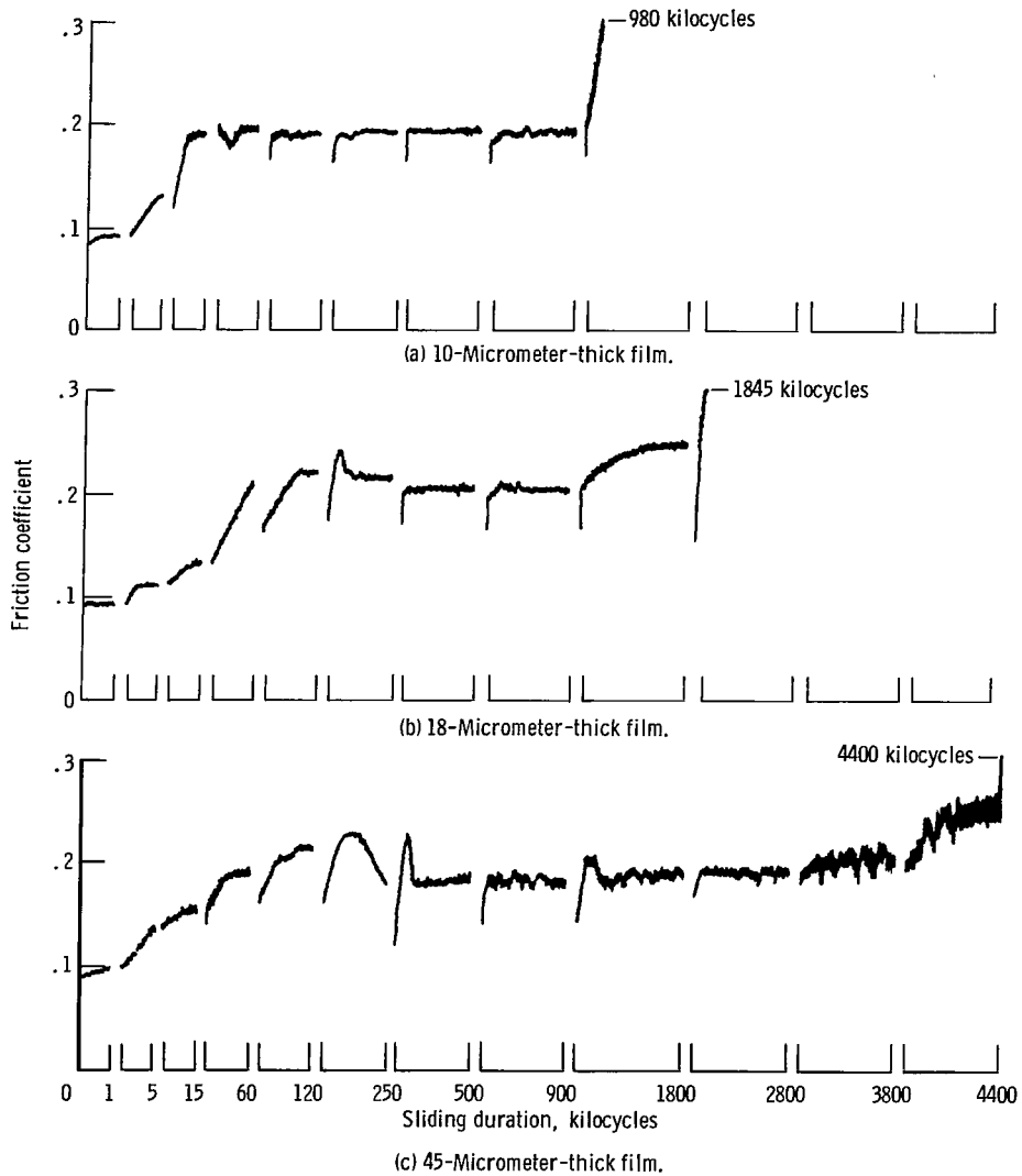
Figure 2. - Friction traces for 440C HT stainless-steel riders sliding on polyimide-bonded graphite fluoride films 10, 18, and 45 micrometers thick. Load, 1 kilogram; sliding speed, 2.6 meters per second (1000 rpm); temperature, 25° C; atmosphere, moist air (10 000 ppm H 2 O).
