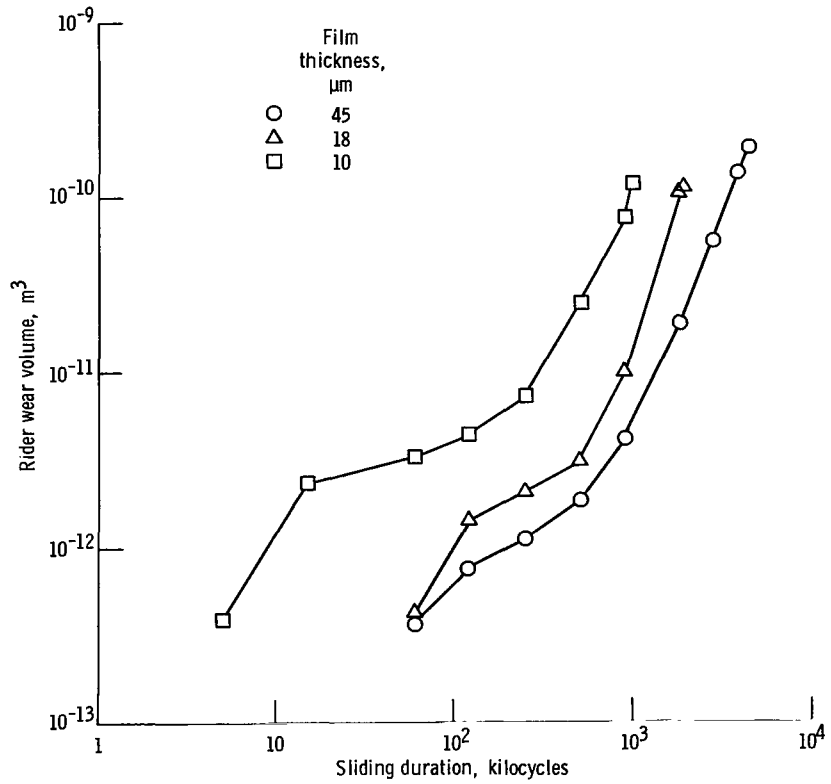
Figure 12. - Rider wear as function of sliding duration for riders sliding on polyimide-bonded graphite fluoride films of three thicknesses. Rider and disk substrate material, 440C HF stainless steel; rider radius, 0.476 centimeter (hemispherically tipped); load, 1 kilogram; sliding speed, 2.6 meters per second (1000 rpm); temperature, 25 o C; atmosphere, moist air (10 000 ppm H 2 O).
