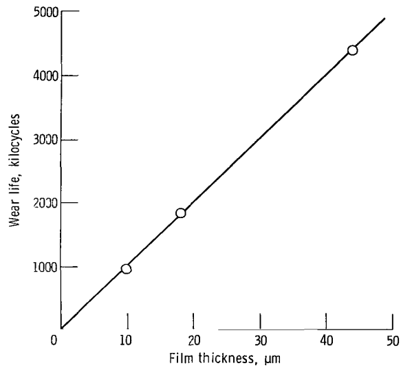
Figure 3. - Wear life as function of polyimide-bonded graphite fluoride film thickness. Rider and disk substrate material, 440C HT stainless steel; rider radius, 0.476 centimeter (hemispherically tipped); load, 1 kilogram; sliding speed, 2.6 meters per second (1000 rpm); temperature, 25 o C; atmosphere, moist air (10 000 ppm H 2 O).
