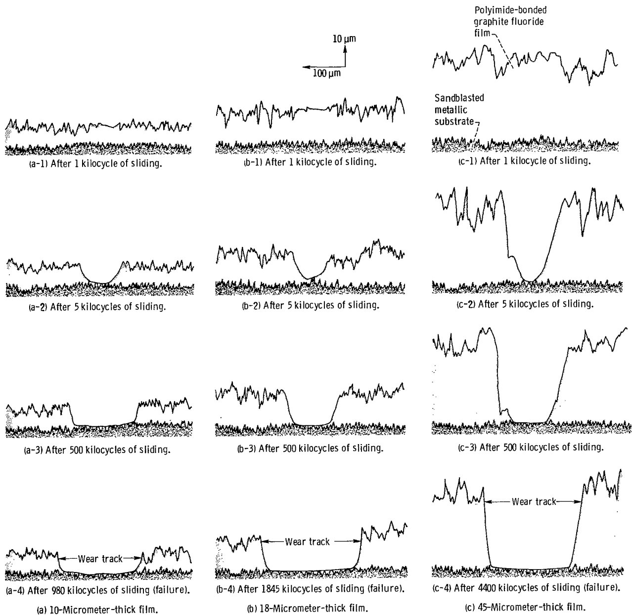
Figure 4. - Surface profiles of the wear tracks on polyimide-bonded graphite fluoride films of three thicknesses after various sliding intervals. Rider and disk substrate material, 440C HT stainless steel; rider radius, 0.476 centimeter (hemispherically tipped); load, 1 kilogram; sliding speed, 2.6 meters per second (1000 rpm); temperature, 25° C; atmosphere, moist air (10 000 ppm H 2 O).
