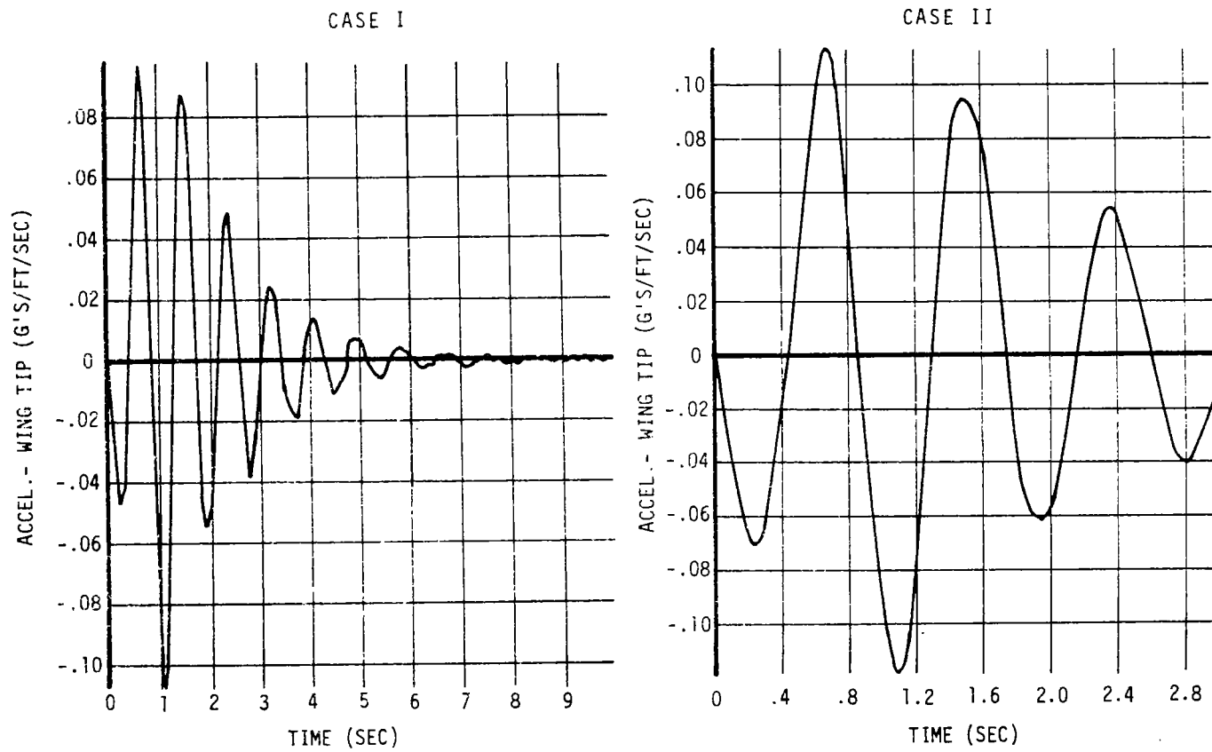
Figure 9.—Interval Spacing Effect on Acceleration Response
