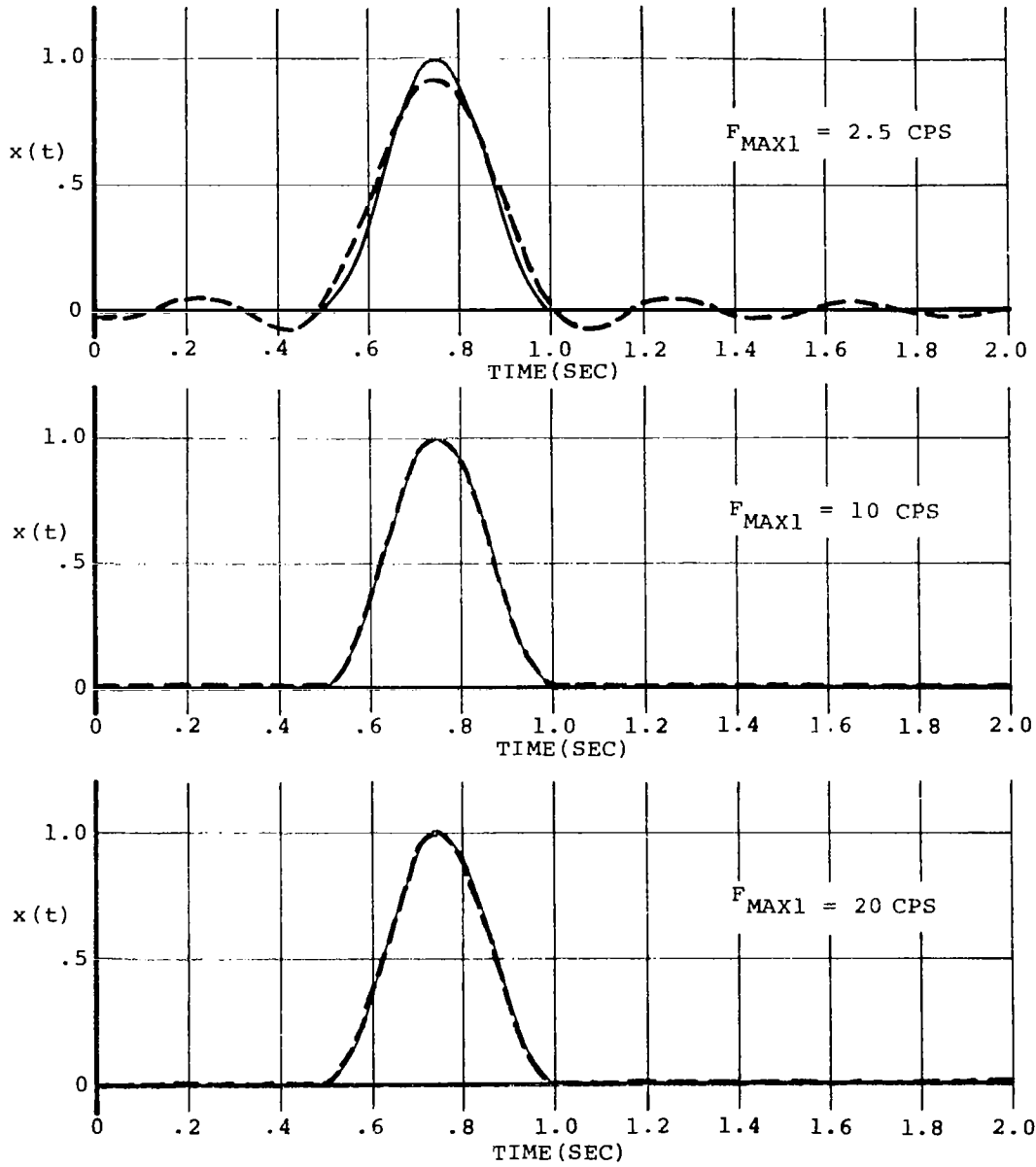
Figure 6. -Cutoff Frequency Effect on a One-Half (1 - \cos) Wave
