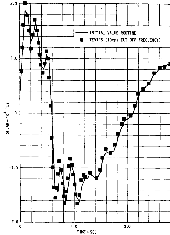
Figure 13.—Comparison of an Airplane Response to a 25-Chord Rectangular Wave in the Time Domain
