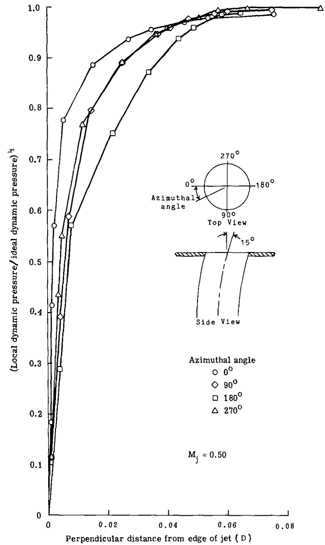
(b) 15° deflection nozzle.
