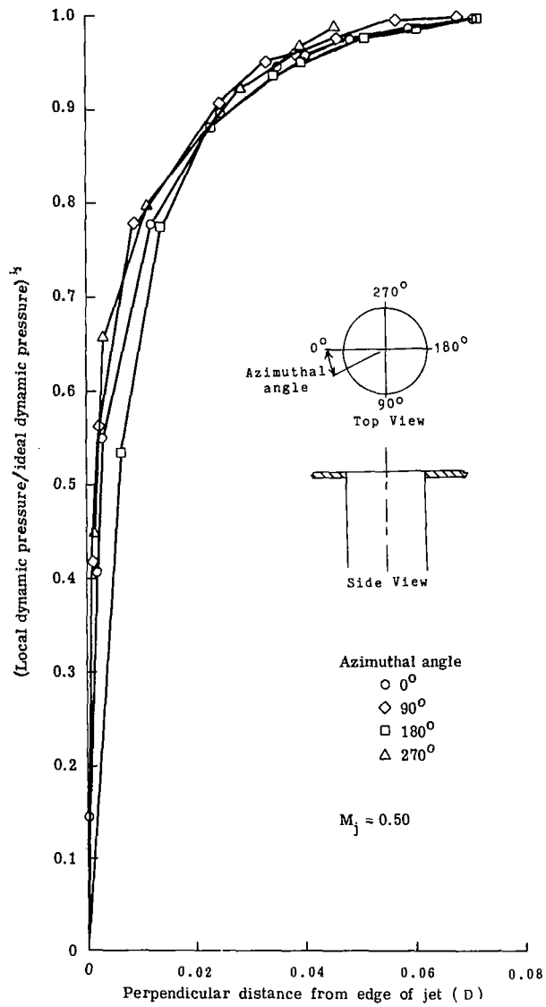
(a) 0° deflection nozzle.
