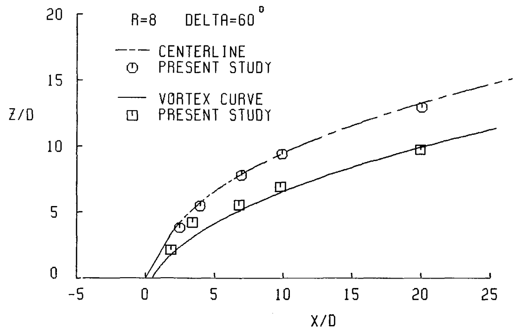
(b) Effective velocity ratio of 8.
