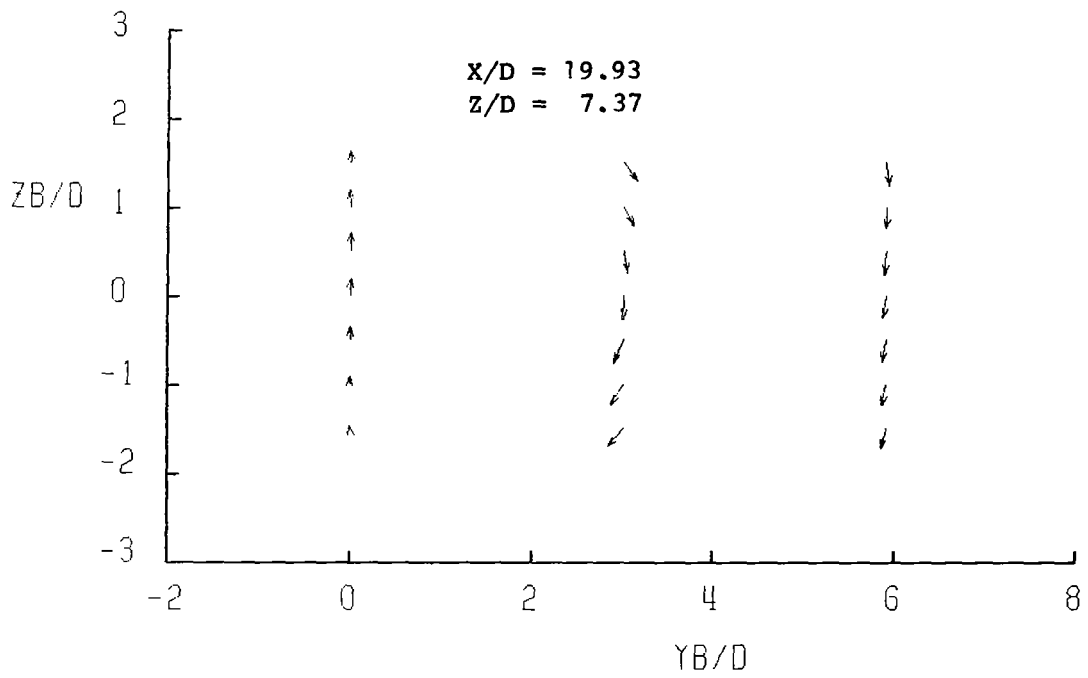
Figure B9.- Concluded.
