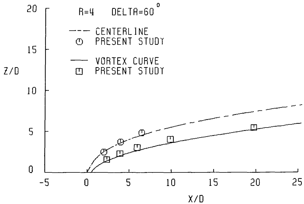
(a) Effective velocity ratio of 4.
