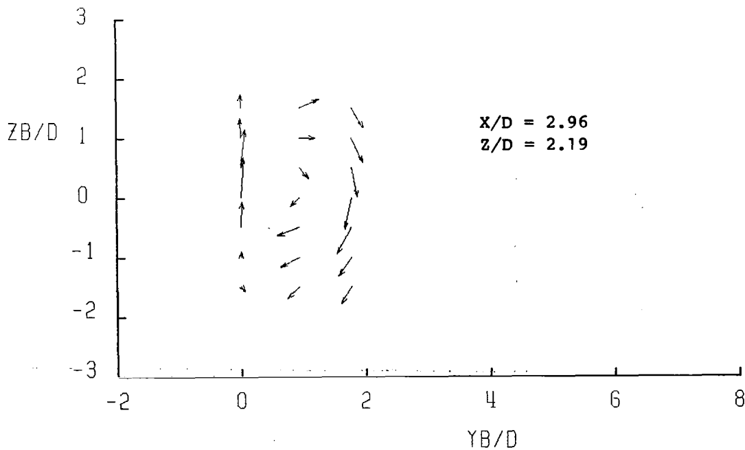
(b) Cross-section velocity plots.
