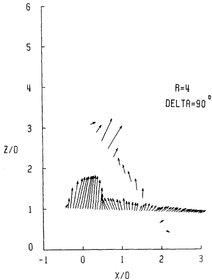
(a) Effective velocity ratio of 4.
