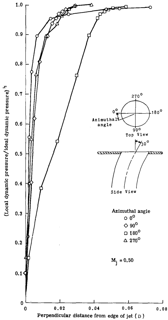
(c) 30° deflection nozzle.
