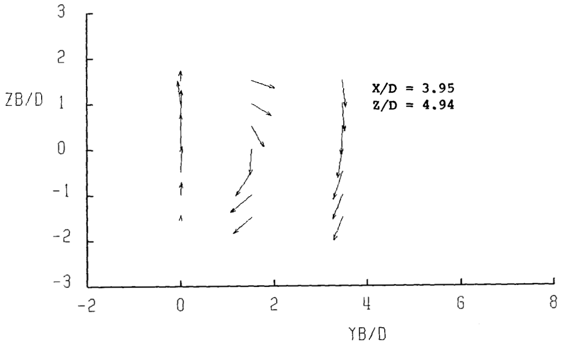
(b) Cross-section velocity plots.
