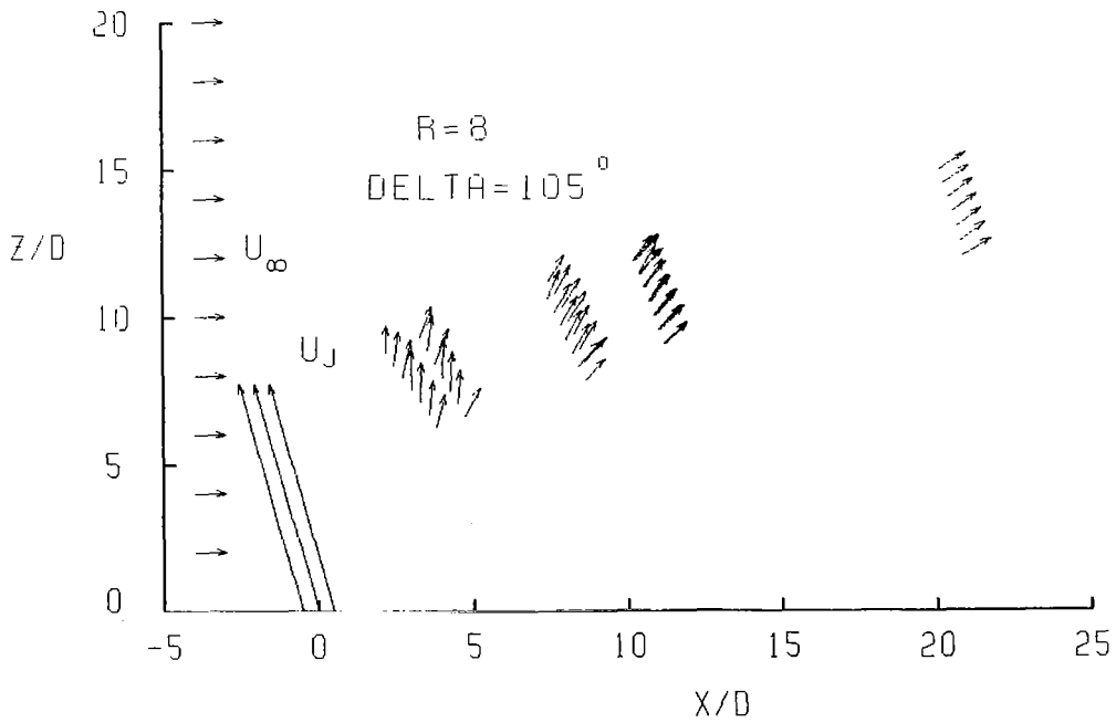
Figure B2.- Concluded.
