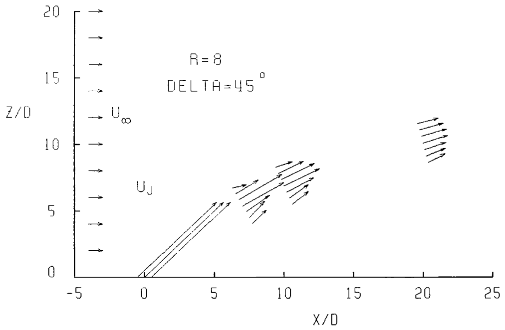
Figure B1.- Continued.
