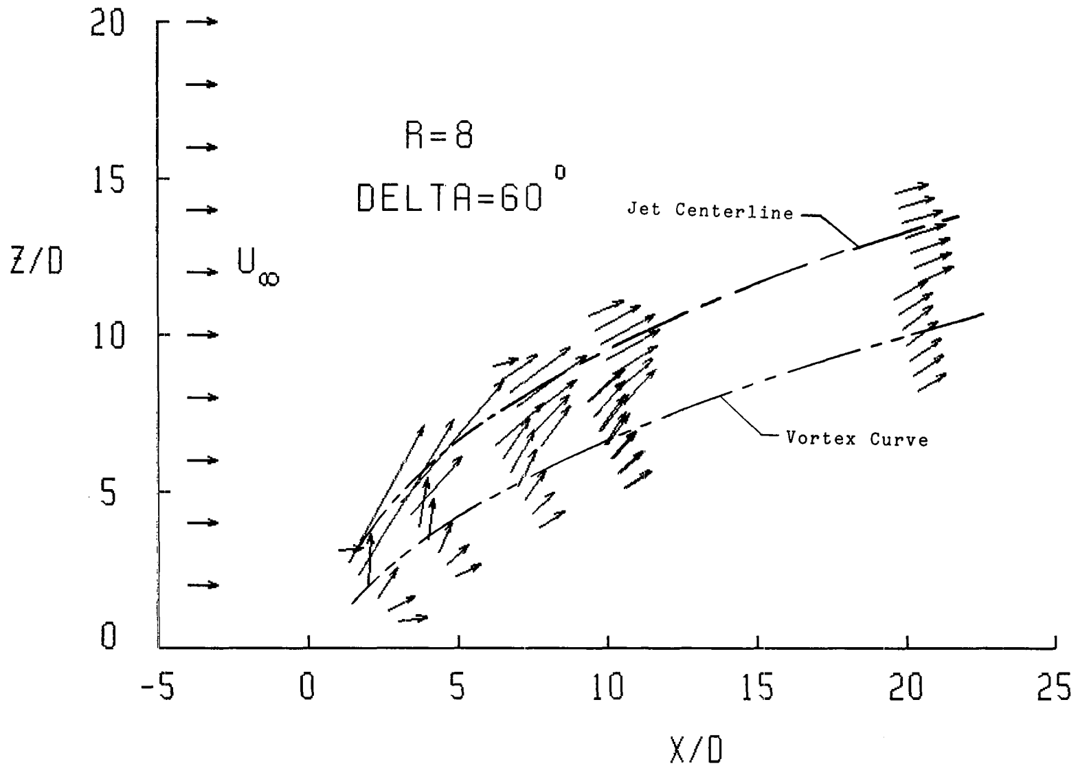
Figure 6.- Symmetry plane velocities.
