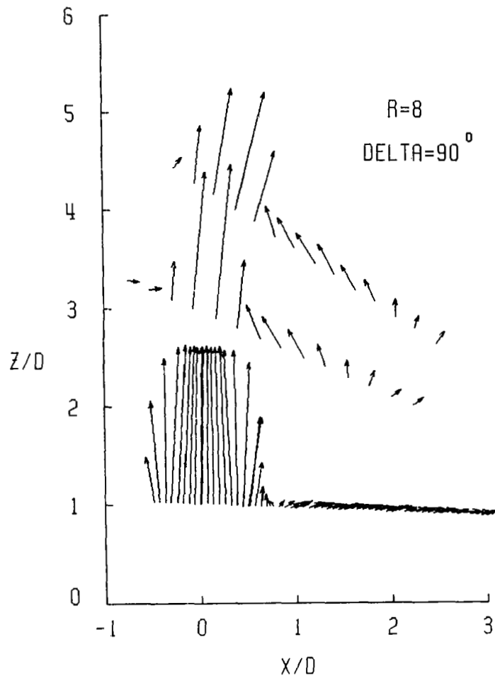
(b) Effective velocity ratio of 8.
