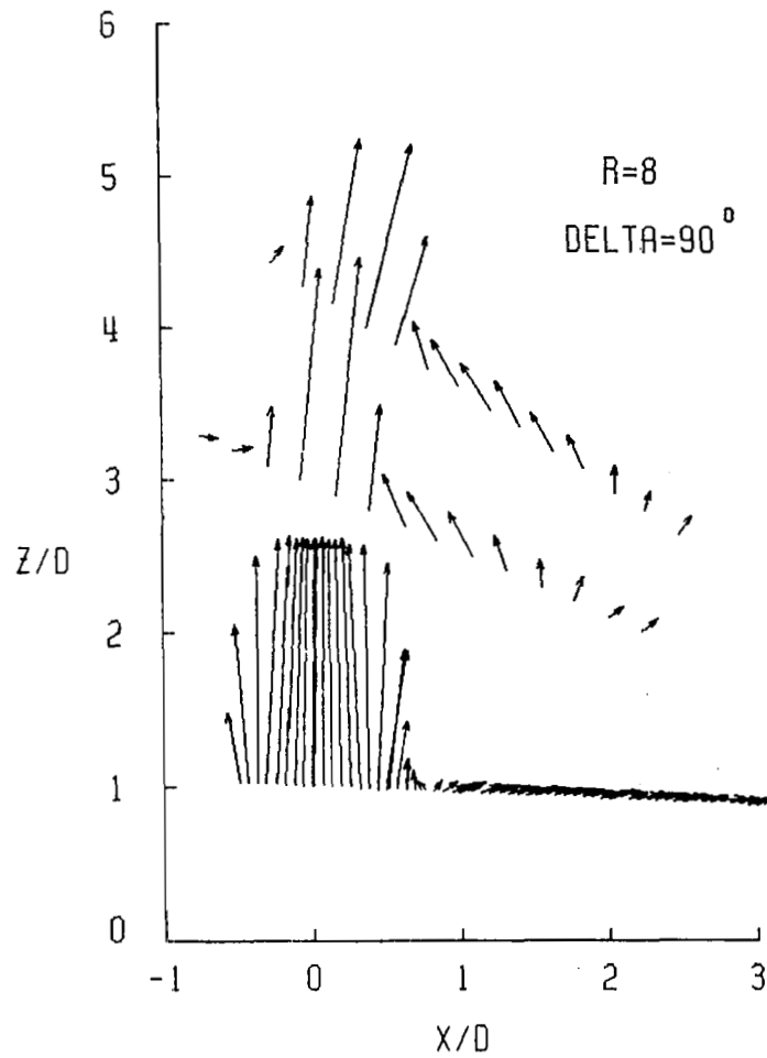
Figure B3.- Symmetry plane velocities near jet orifice.
