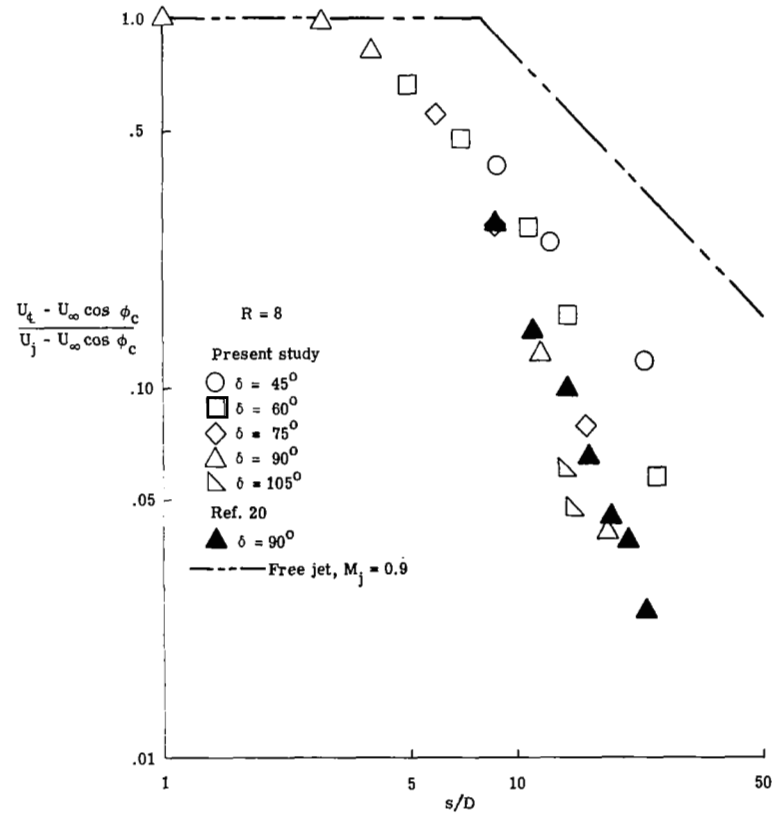
(b) Effective velocity ratio of 8.
