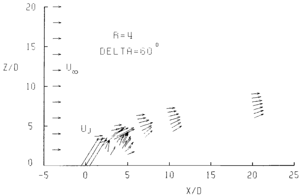
Figure B1.- Symmetry plane velocities in jet centerline vicinity.
