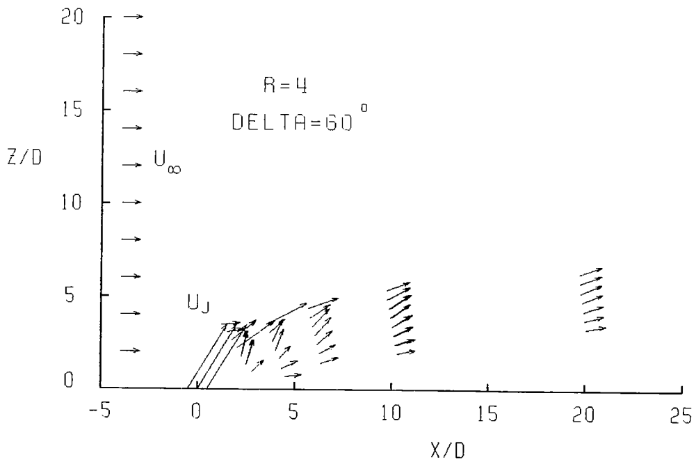
Figure B2.- Symmetry plane velocities in vortex-curve vicinity.
