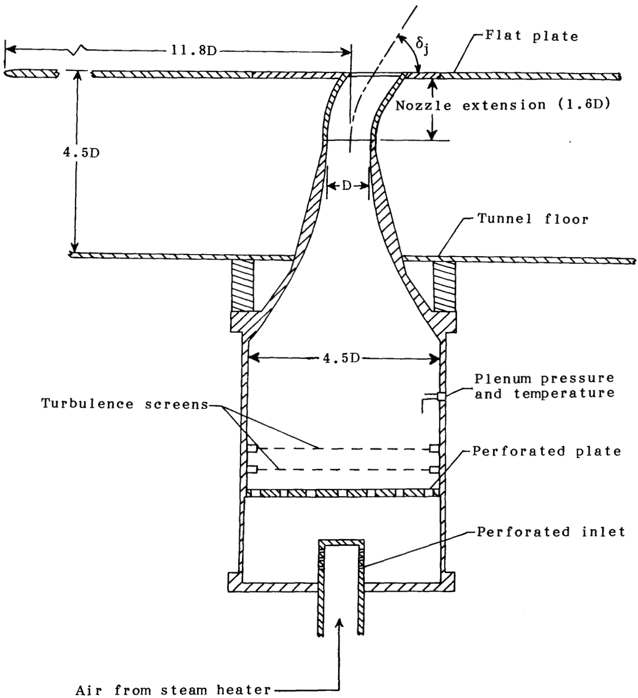
Figure 3.- Jet plenum and nozzle.
