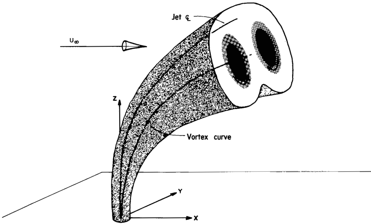
Figure 1.- Sketch of the jet plume.
