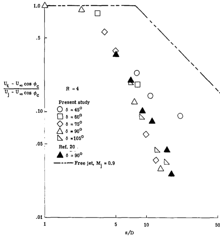
(a) Effective velocity ratio of 4.
