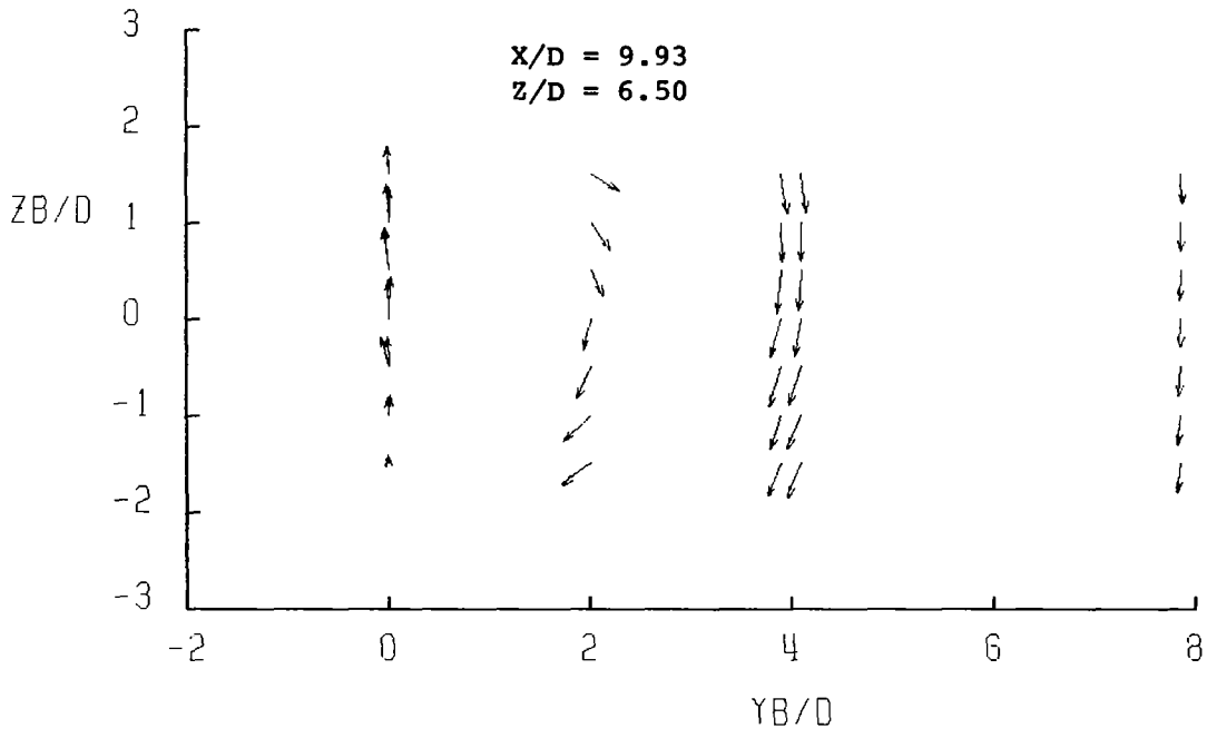
Figure B10.- Concluded.
