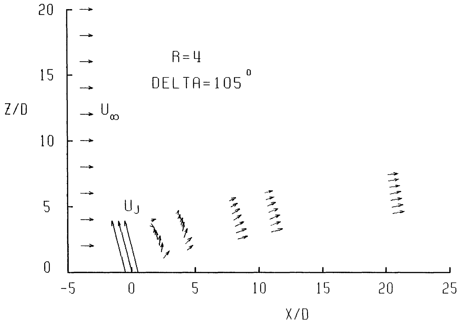
(a) Symmetry plane velocity plot locating cross sections of measurement.
