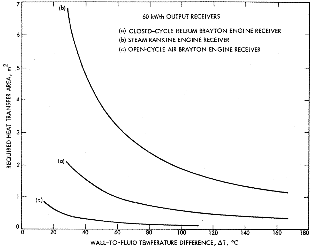
Figure B-6. Heat Transfer Area and Temperature Difference Relationship for Typical Receivers
