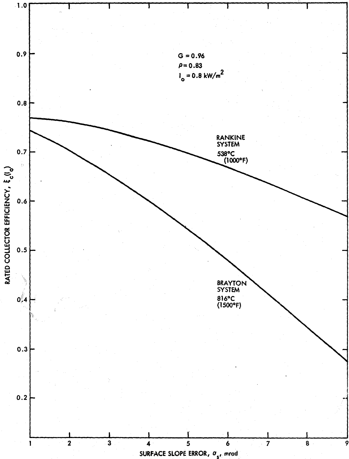
Figure 2-15. Collector Efficiency versus Surface Slope Error at Design Point Insolation
