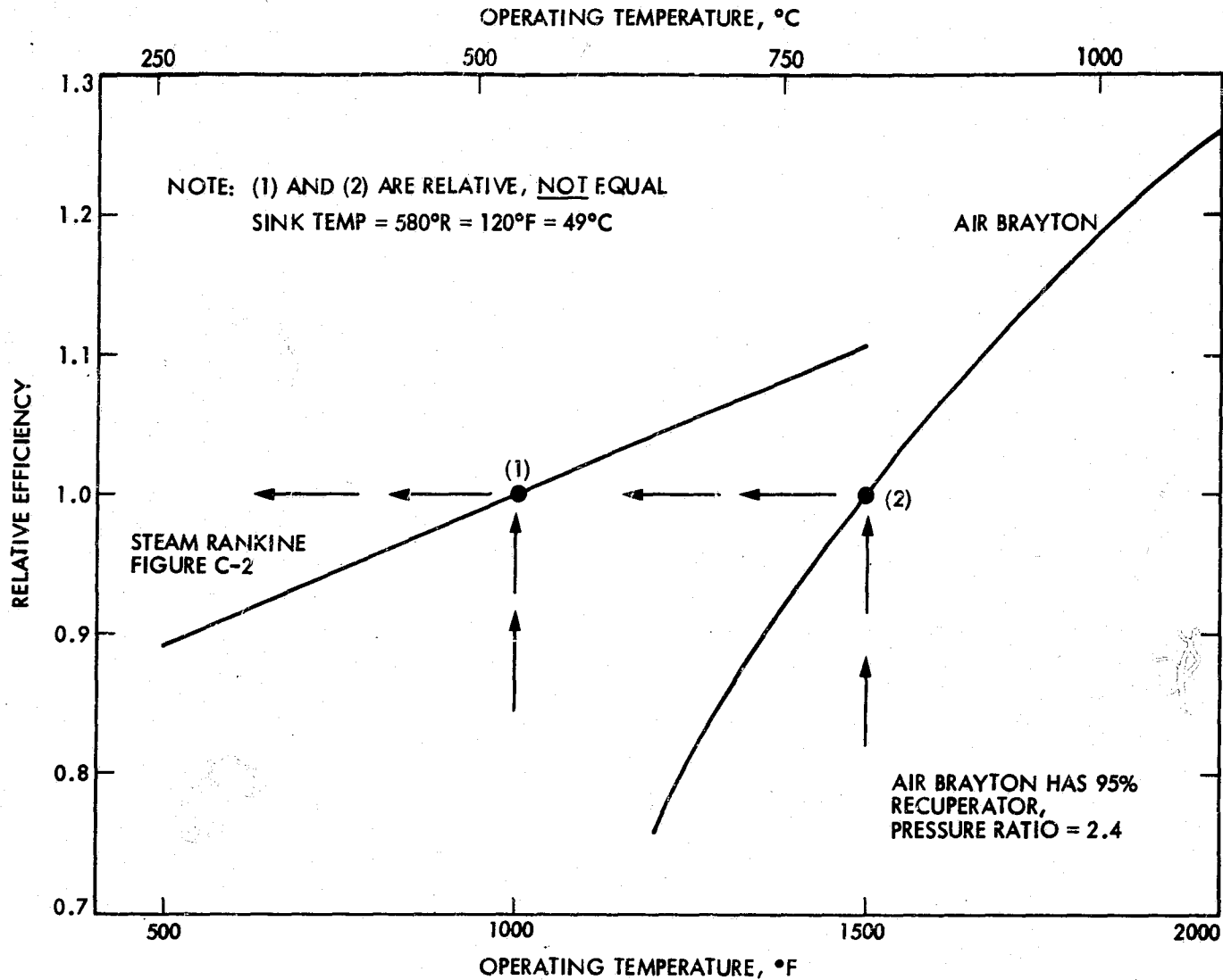
Figure C-4. Brayton Cycle Efficiency versus Operating Temperature
