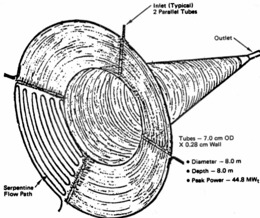
Figure 4-11. Partial Cavity Receiver 10 MW e
