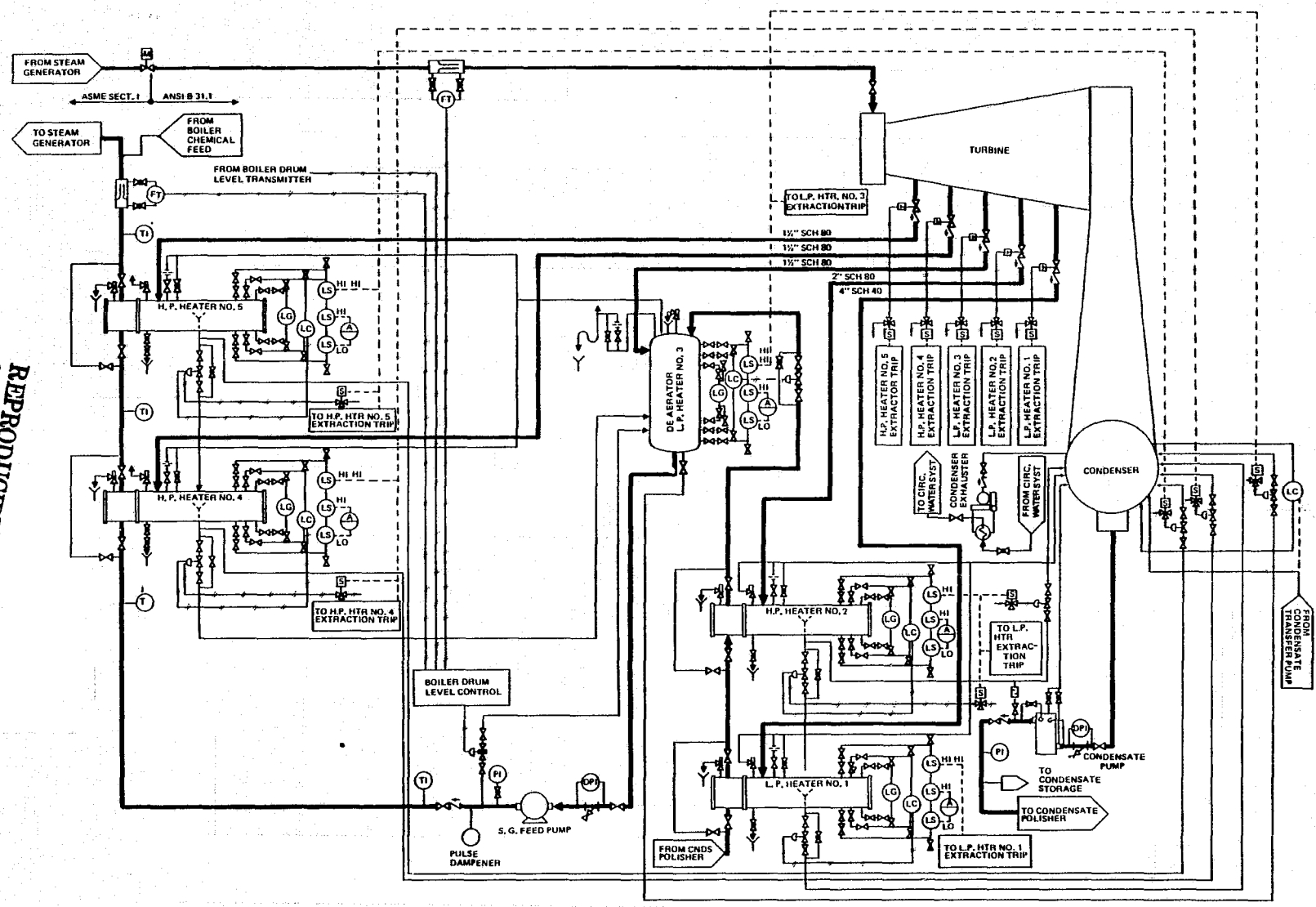
Figure 3-10. Steam, Condensate, Feedwater, Extraction Steam, Heater Vents, and Drains Flow Diagram for Commercial Program
