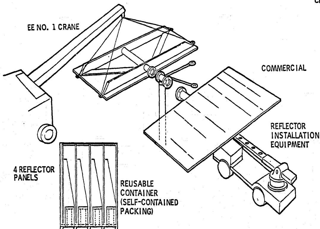
Figure 3-15. Heliostat Installation
