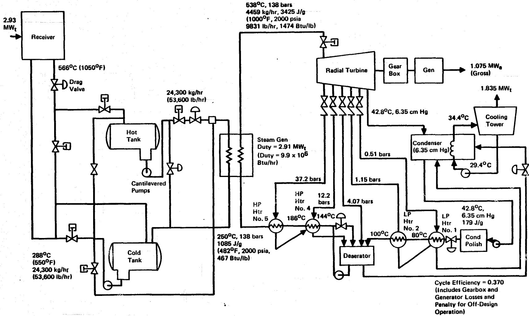
Figure 5-2. System Schematic ( 1 \text{ Mw}_e , \text{CF} = 0.275 )
