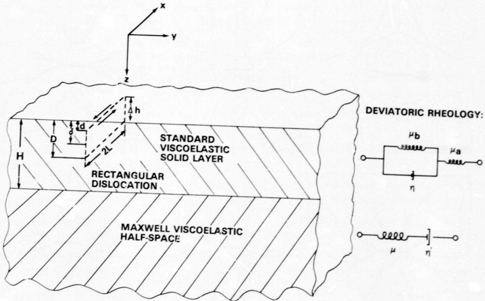
Figure 1. Viscoelastic Model for Deformation and Stress Due to an Earthquake Along a Strike-Slip Fault
