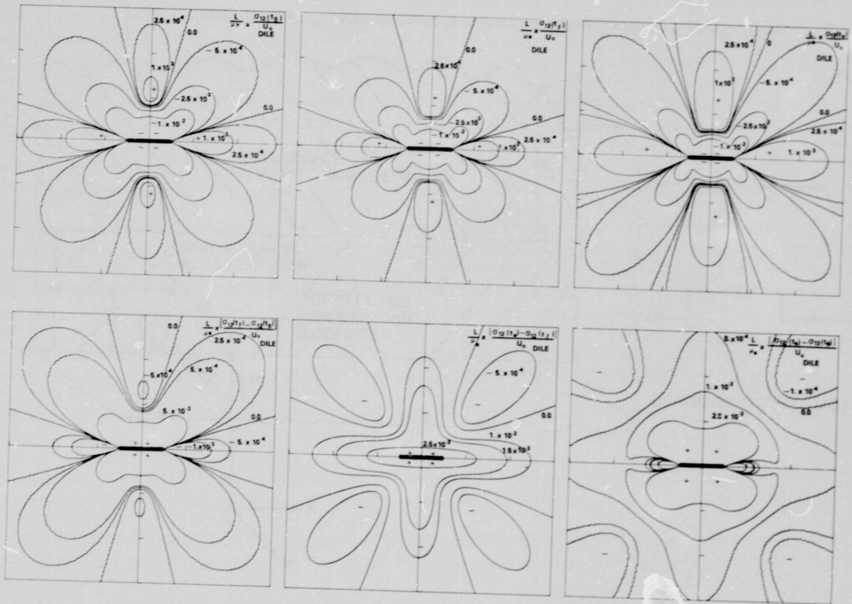
Figure 2. Shear Stress, \sigma_{12}(t) . Fault extends along x axis from -L to +L . Tick mark \dots = 2L .
