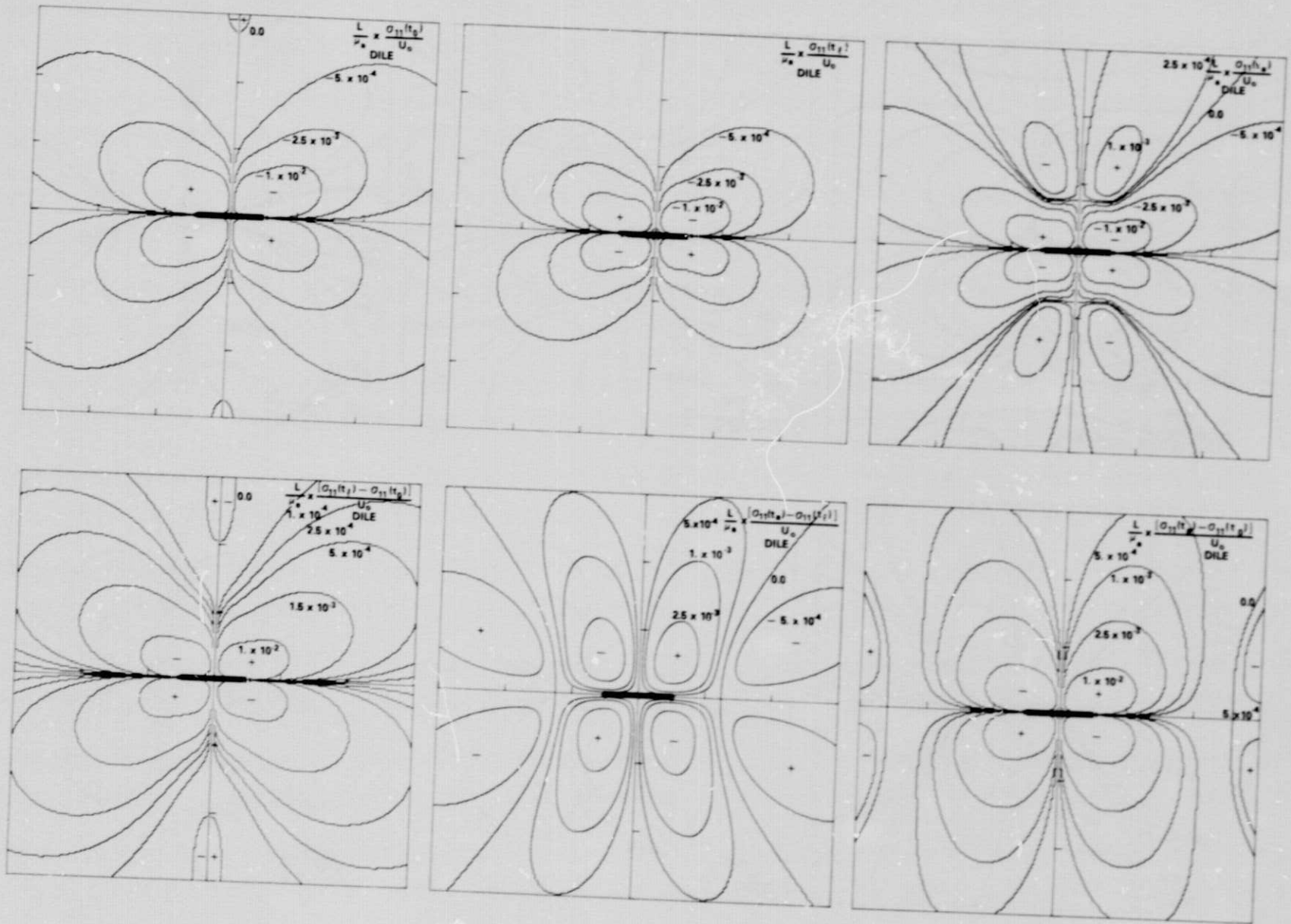
Figure 3. Normal Stress, \sigma_{11}(t)
