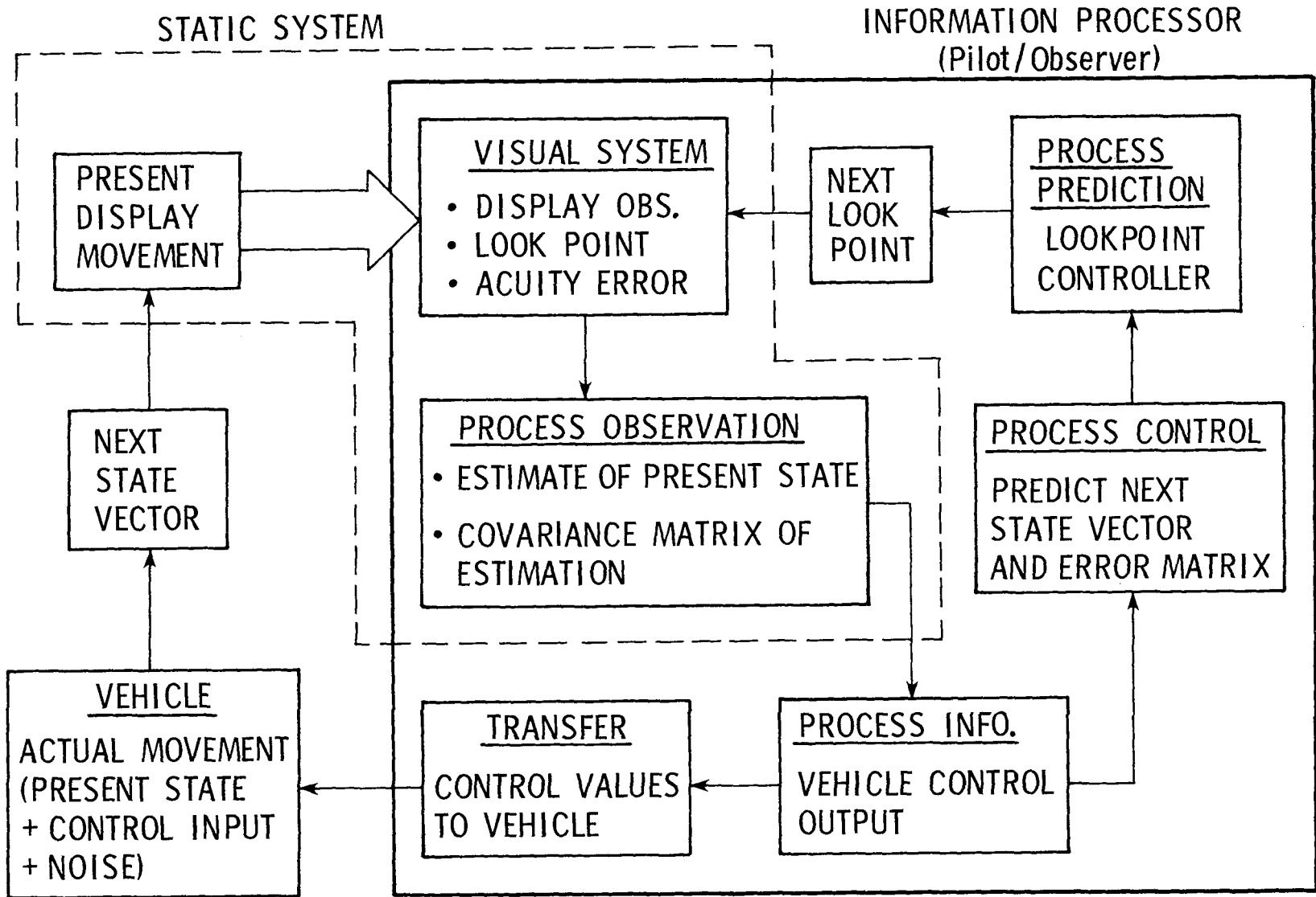
Figure 6.- Information flow for dynamic system.
