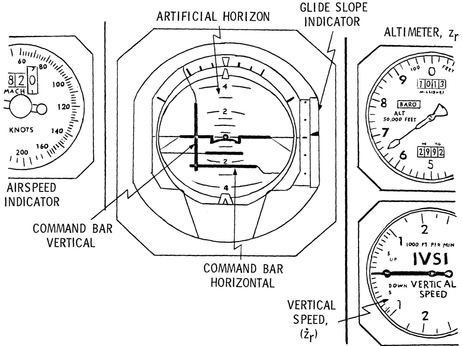
Figure 7.- Display setup.
