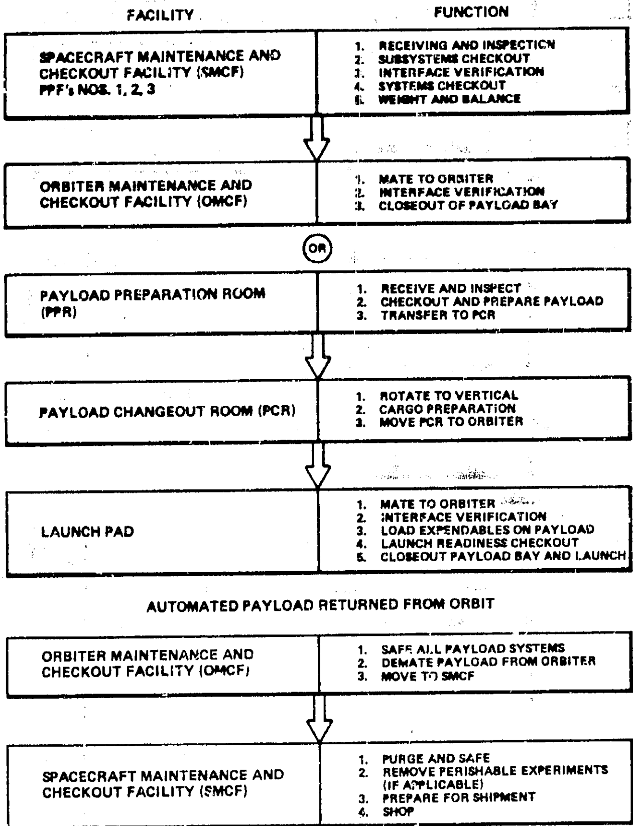
Figure 8-5. Typical Automated Payload Flow at WTR
