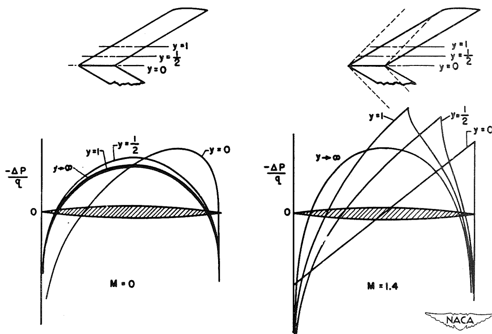
Figure 7.- Pressure distributions at several sections of a symmetrical biconvex wing at 0° angle of attack.
