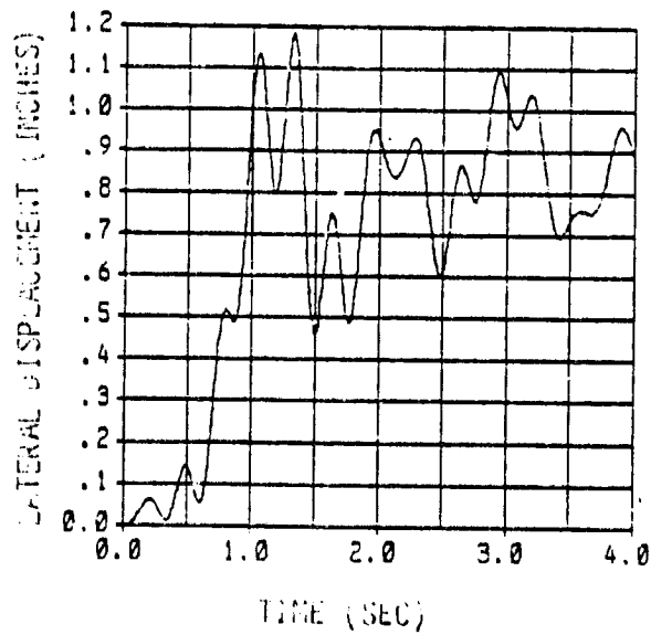
Figure 17 Wing Lateral Displacement History for Typical Revenue Service Landing
