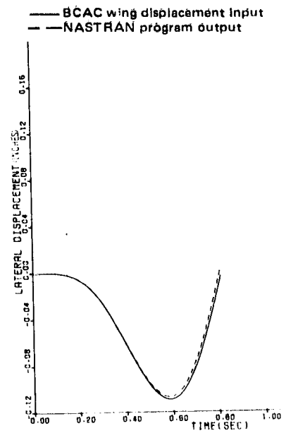
Figure 30 Wing Lateral Displacement Evaluation for Vertical Gust
