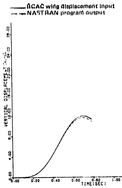
Figure 29 Wing Vertical Displacement Evaluation for Vertical Gust
