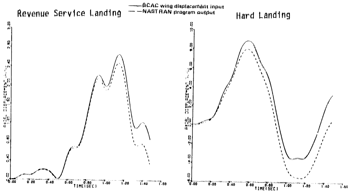
Figure 37 Wing Axial Displacement Evaluation for Landing Events
