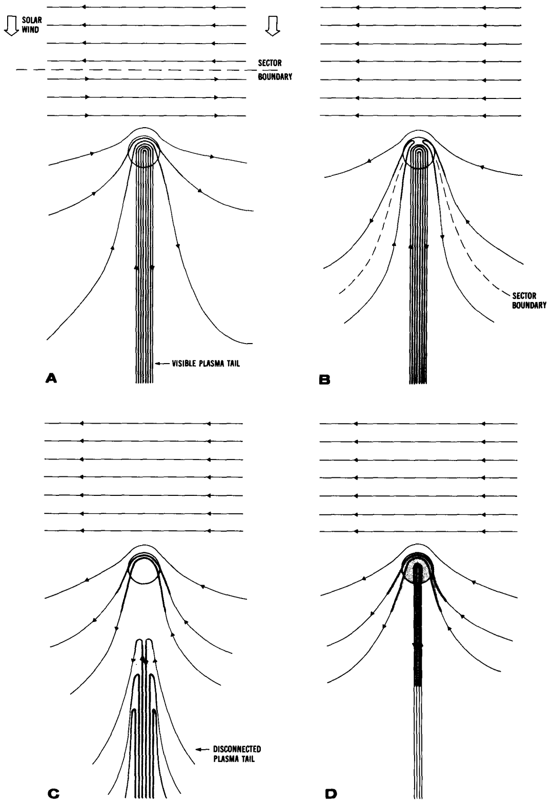
Fig. 12. Process of disconnection of a comet tail in response to the passage of an interplanetary sector boundary. (From Niedner and Brandt, 1978)
