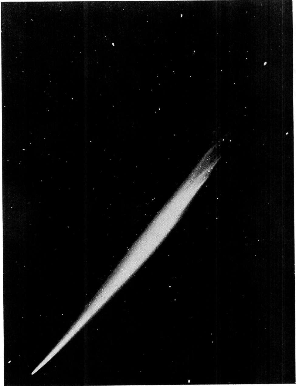
Fig. 2. Comet Ikeya-Seki, 1965 VIII.
