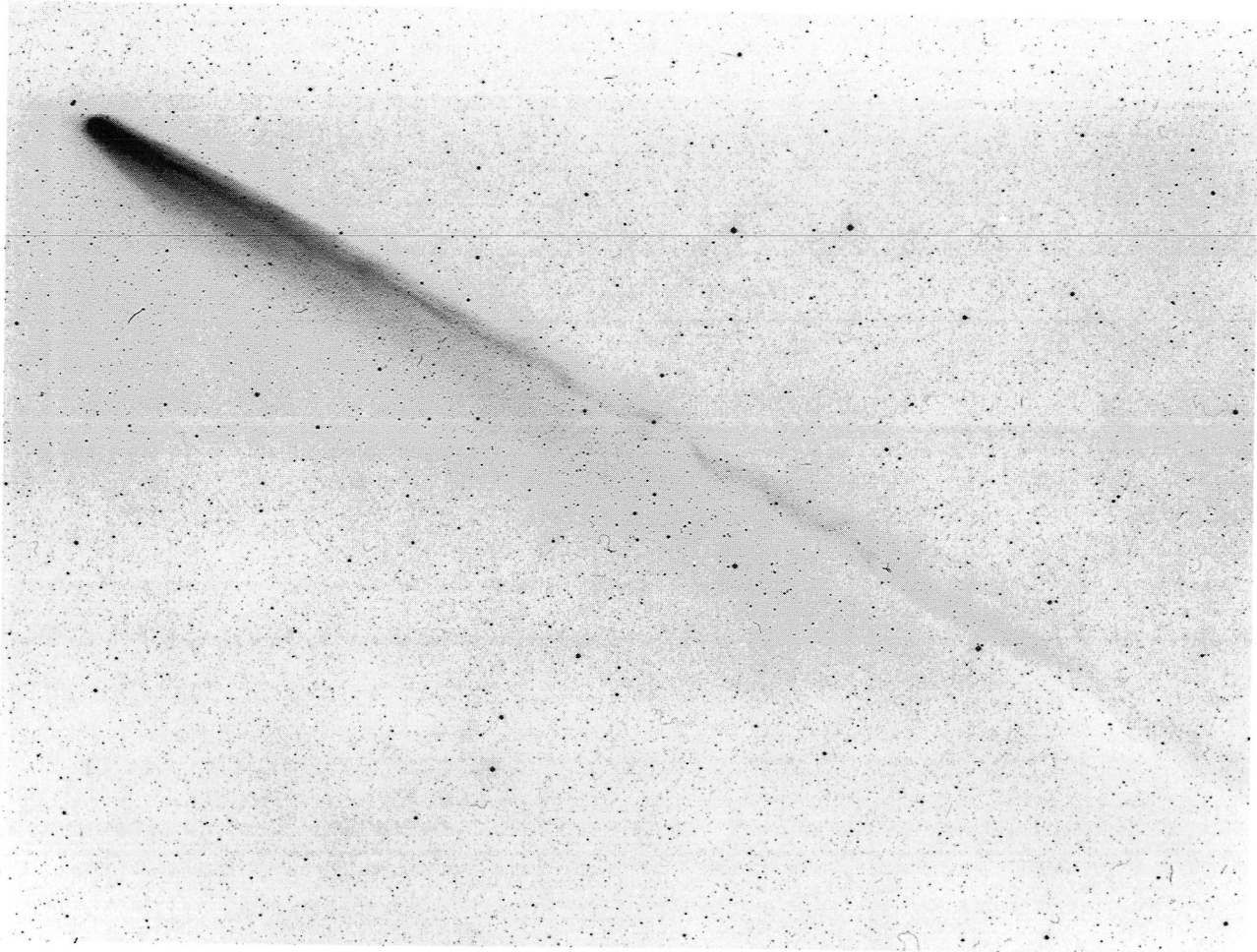
Fig. 7. Comet Kohoutek, 1973 XII. (Joint Observatory for Cometary Research photograph)
