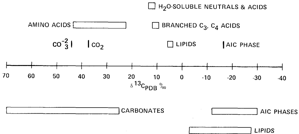
Fig. 4. Isotopic composition of carbon phases in Murchison (above the scale line) and in other carbonaceous meteorites. AIC phase corresponds to a cid i nsoluble c arbonaceous phase. Data are taken from references given in the caption of Fig. 3. The data from lipids in Murchison are judged to be least influenced by exposure to terrestrial contamination.
