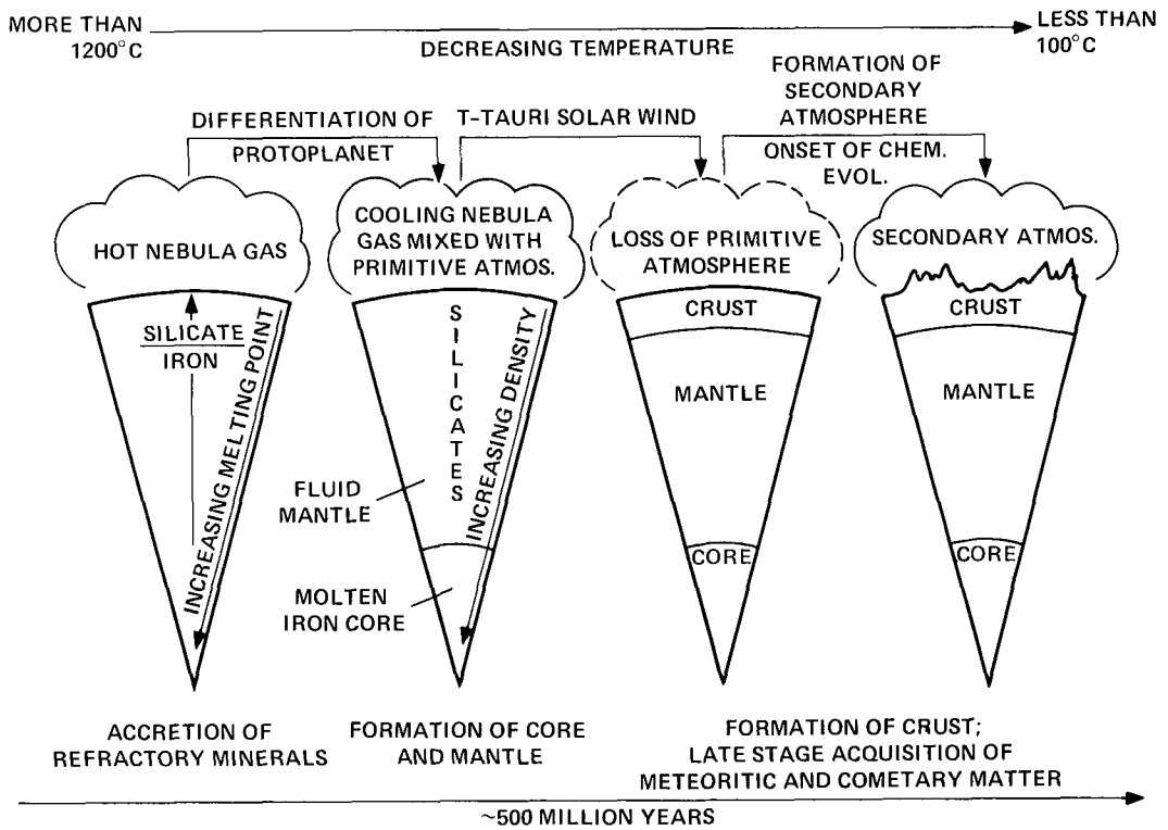
Fig. 5. Stages in the Earth's early evolution.
