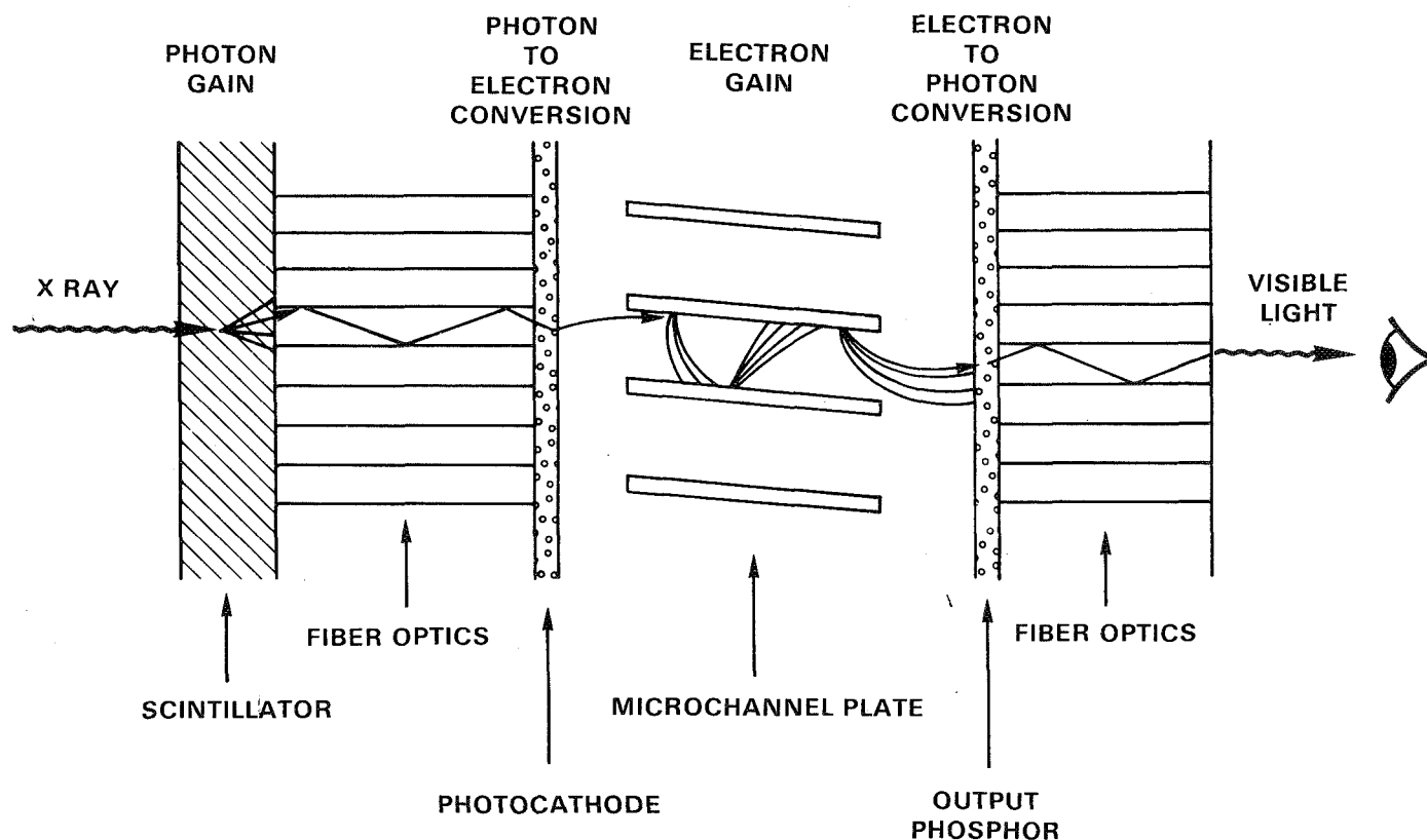
Figure 1. Principle of the Lixiscope
