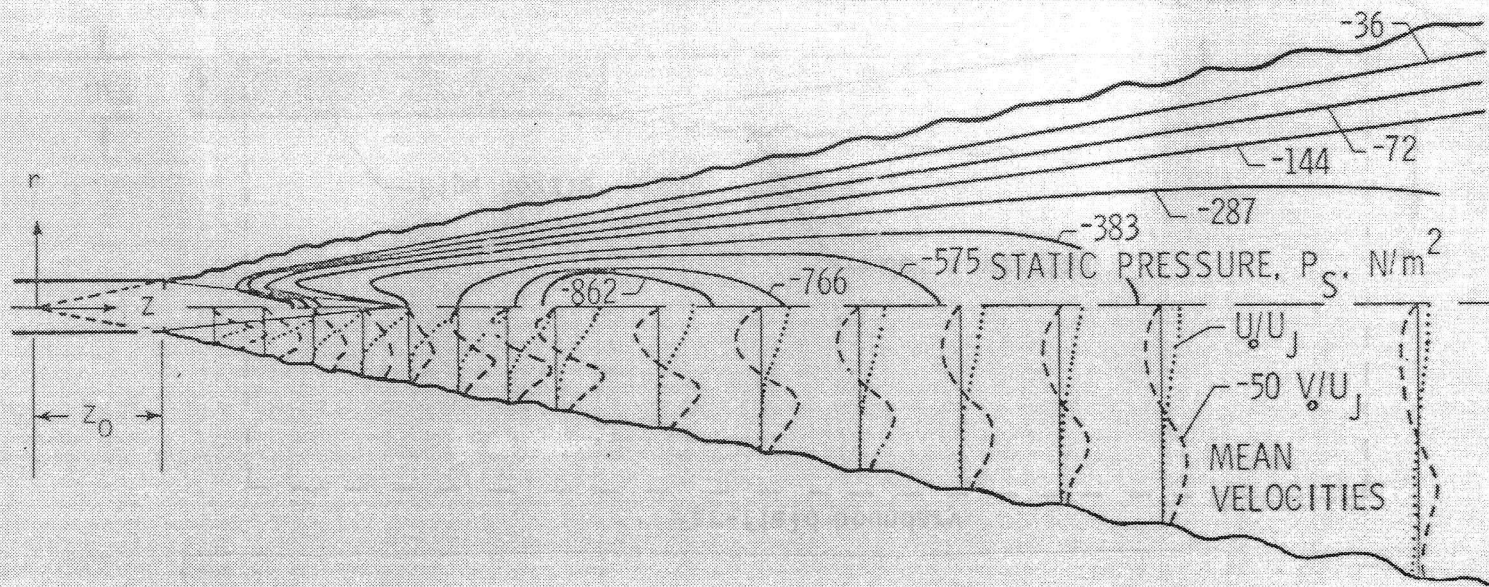
Figure 2. Experimental configuration and mean flow field.
