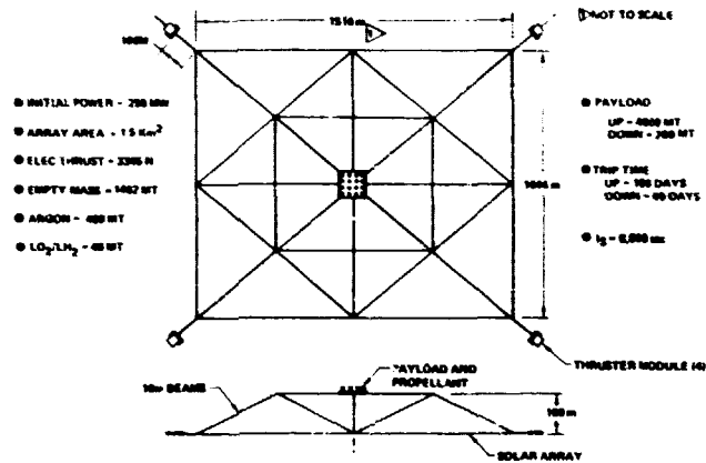
Figure 22. Electric OTV Configuration
