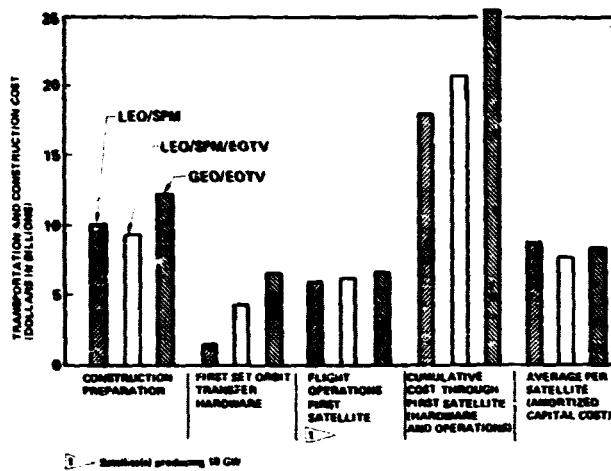
Figure 23. Construction/Transportation Cost Comparison
