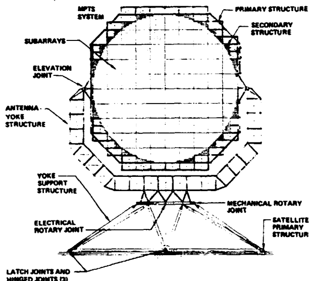
Figure 28. Reference MPTS Structural Approach
