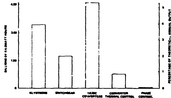
Figure 16. Annual Power Loss due to Failures
