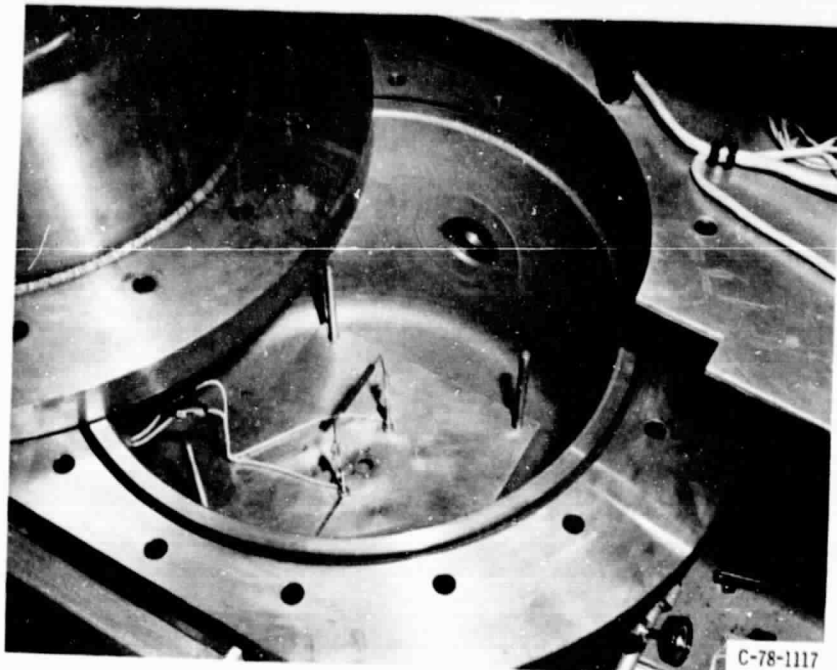
Figure 8. - Carbon rod in burning chamber.
