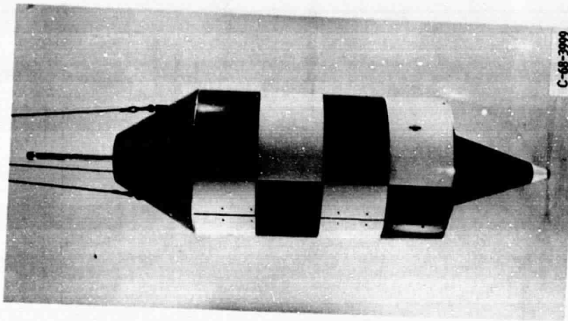
Figure 5. - Experiment vehicle.
