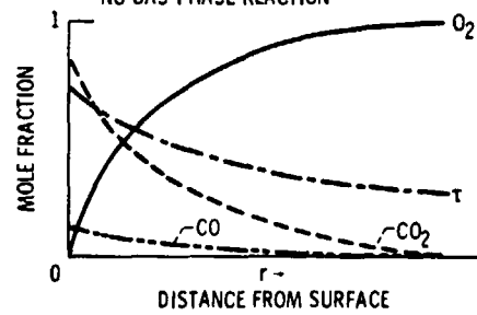
Figure 2. - Mid temperature model.
