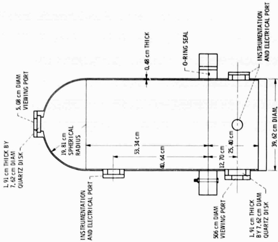
Figure 7. - Cross-sectional schematic of combustion chamber.
