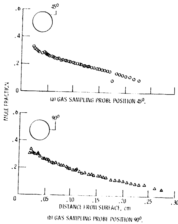
Figure 25. - CO concentration as a function of distance from surface.
