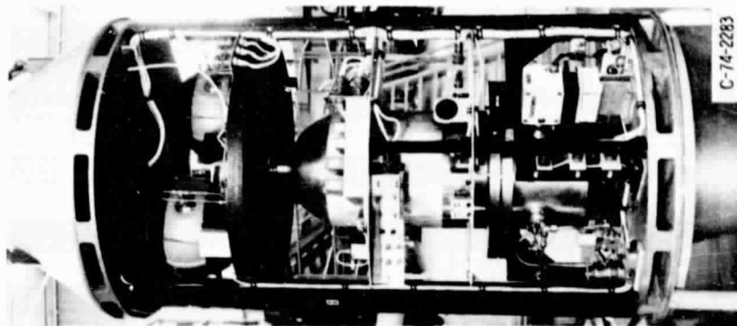
Figure 6. - Test rig.
