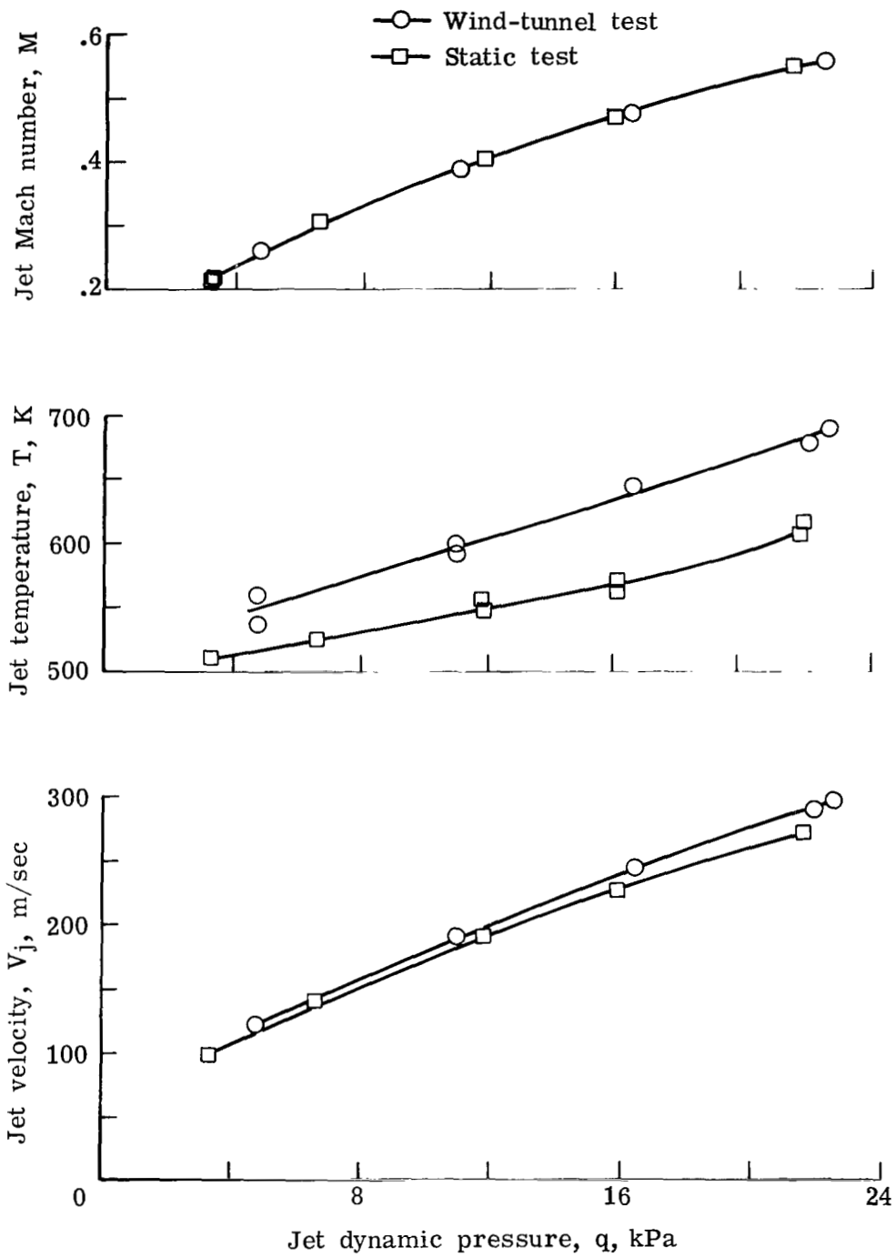
Figure 7.- Condition of efflux at jet exit.
