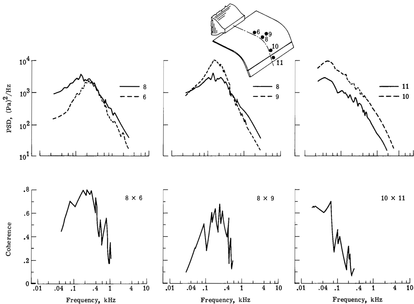
Figure 25.- Coherence function and PSD for three sets of measurement locations for q = 22 \text{ kPa} .
