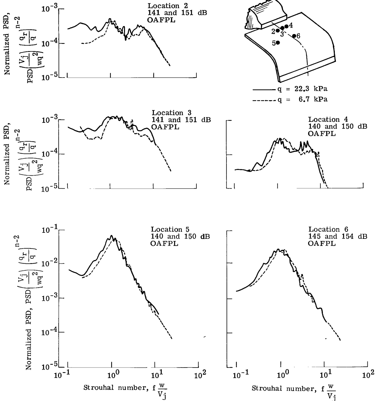
Figure 23.- Comparison of normalized flap loads spectra for q = 6.7 \text{ kPa} and 22.3 \text{ kPa} .
