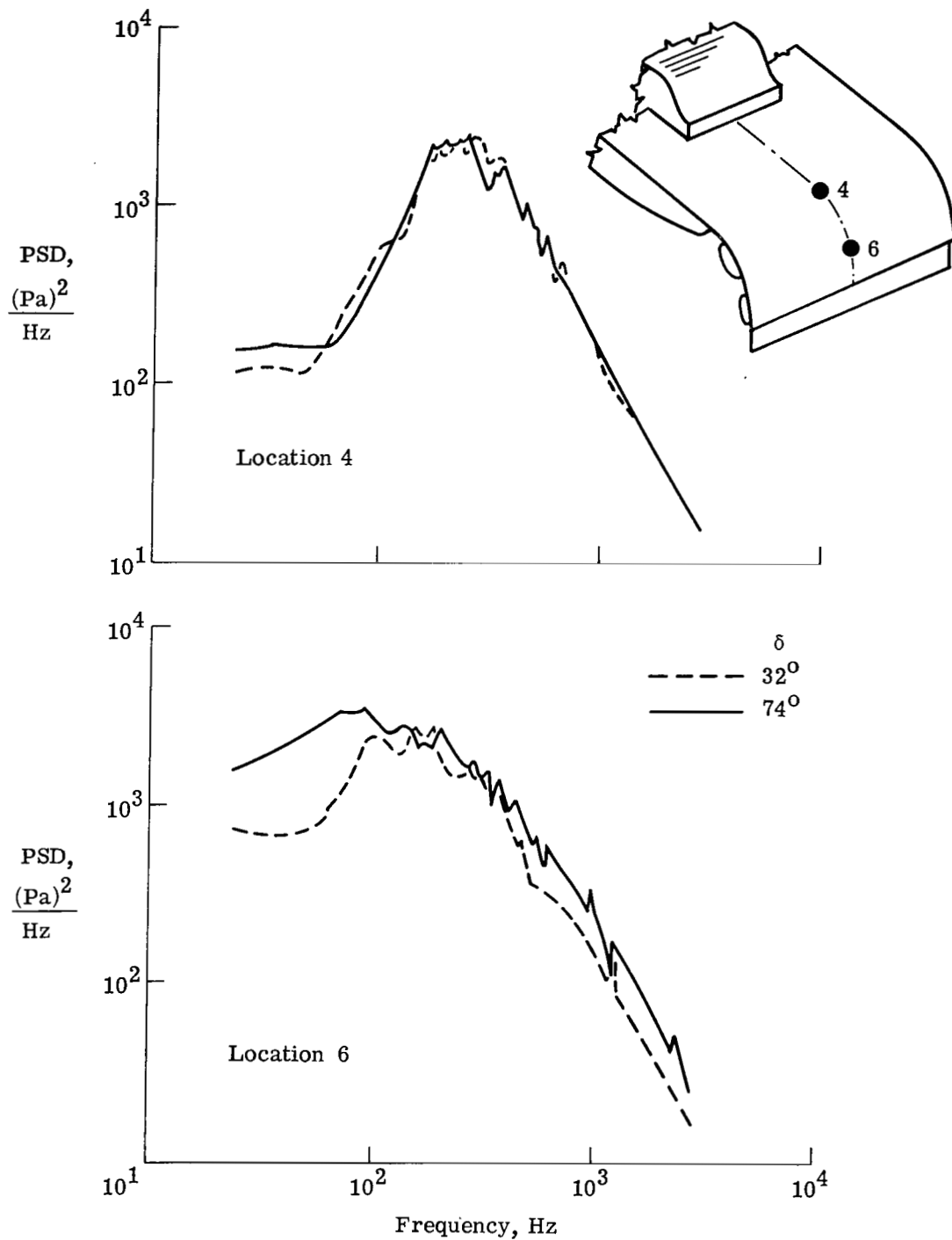
Figure 22.- Comparison of PSD for 32^\circ and 74^\circ flaps.
