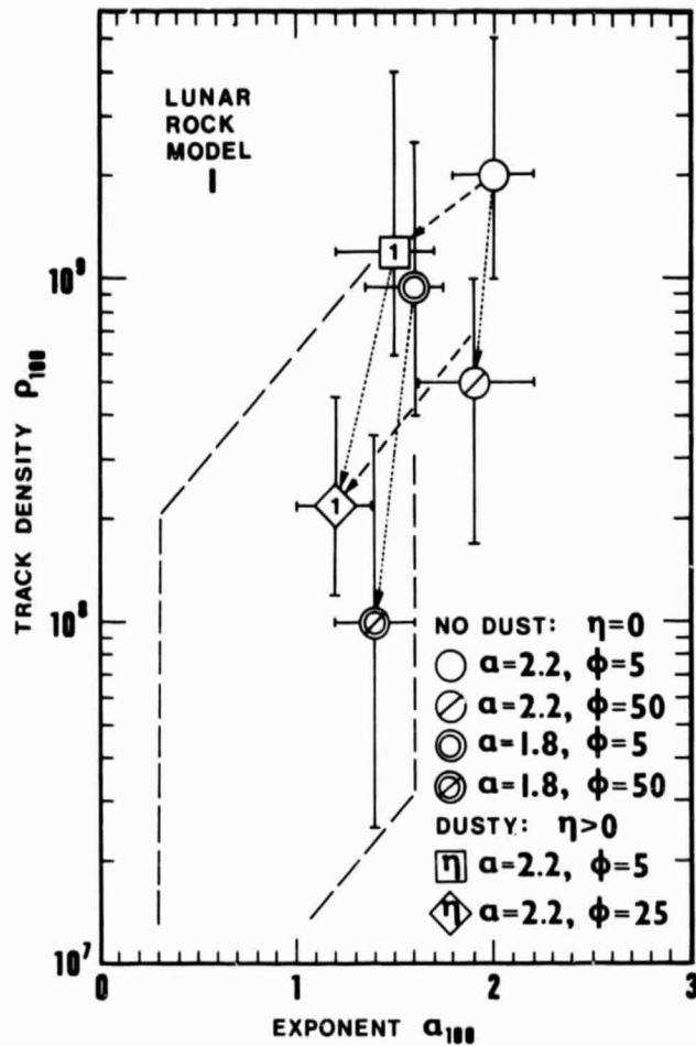
Fig. 6. Calculated track density at 100 \mu\text{m} plotted against the negative exponent of the depth profile at 100 \mu\text{m} for models of impact-saturated rock surfaces which are assumed to be continuously clean (no dust), along with two dusty rock models. \eta is a dust accumulation rate parameter defined in the text. \alpha is the track production profile exponent. \phi is the number of impact pits per \text{cm}^2 \cdot 10^6 years with pit diameter > 500 \mu\text{m} . The parallelogram encloses the normal rock data in Fig. 5. Dashed arrows show the effect of adding dust accumulation and dotted arrows show the effect of increasing the meteoroid flux level.
