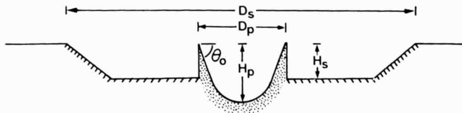
Fig. 1. Idealized cross-sectional shape of microcraters used in rock surface model. Stippled area is glassy pit, shaded area is spall zone which tends to be absent for D_p less than \sim 10 \mu\text{m} .
