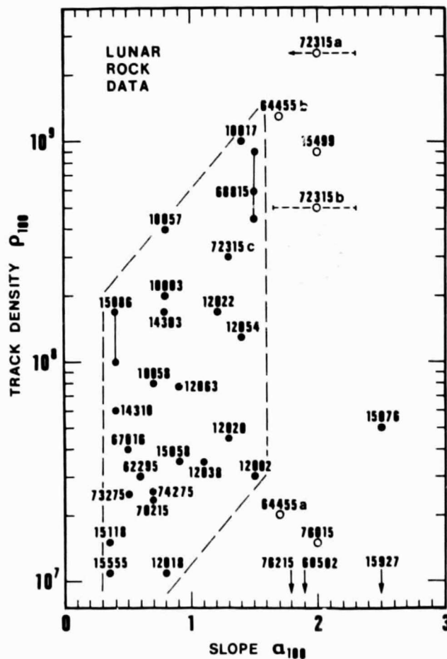
Fig. 5. Measured track density at 100 \mu\text{m} plotted against the negative exponent of the depth profile at 100 \mu\text{m} for 31 rocks reported in 21 papers. References are given in Table 1. Open circles refer to special samples chosen to yield the track production profile.
