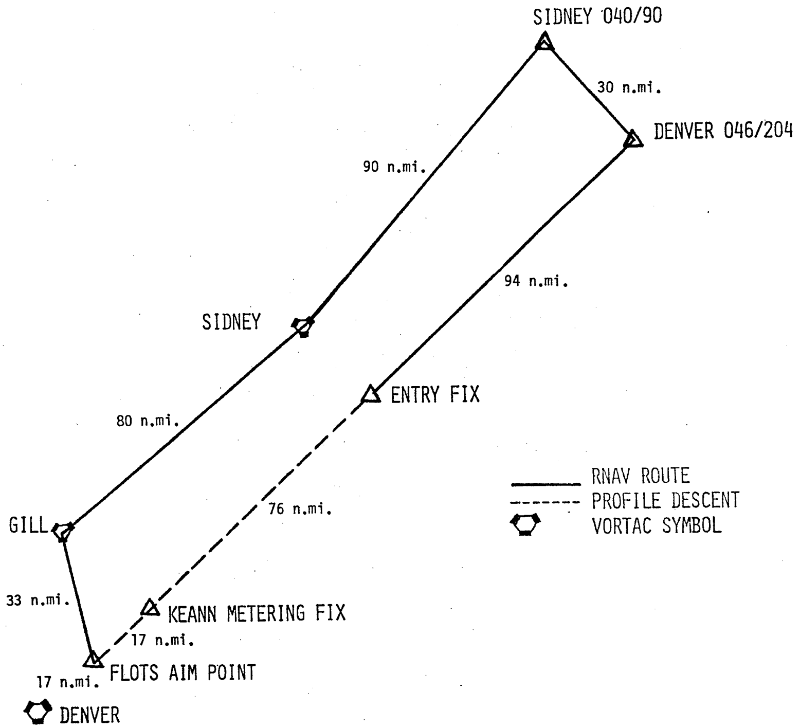
Figure 5. - LFM/PD flight test path.
