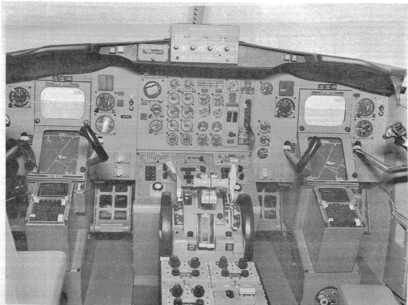
Figure 1. - Research flight deck instrument panel.
