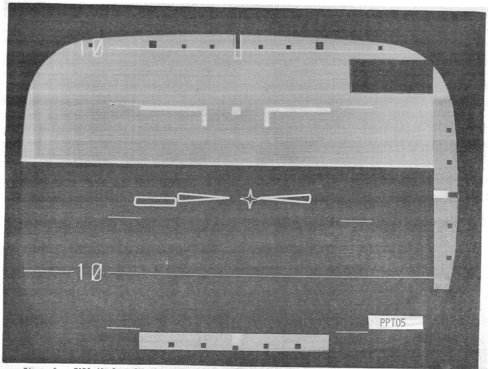
Figure 2. - EADI display with the course deviation indicators and the star and wedges guidance symbology.
