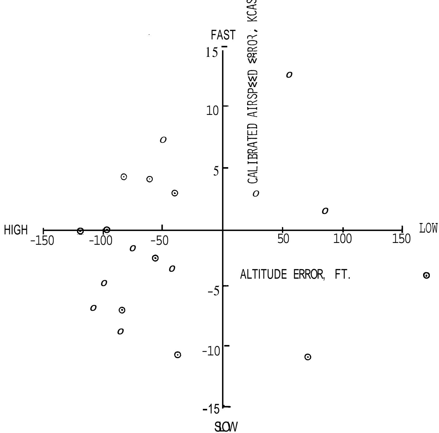
Figure 6. - Calibrated airspeed and altitude errors at the metering fix waypoint.
