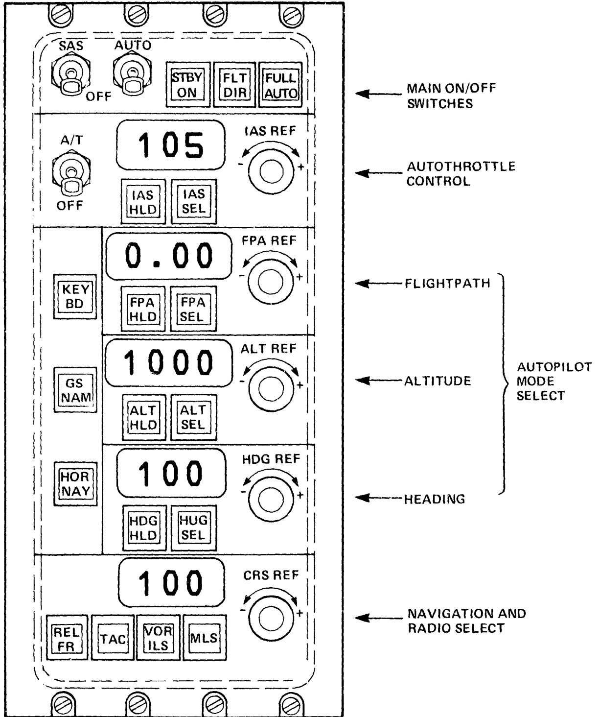
Figure 1.- STOLAND mode-select panel.
