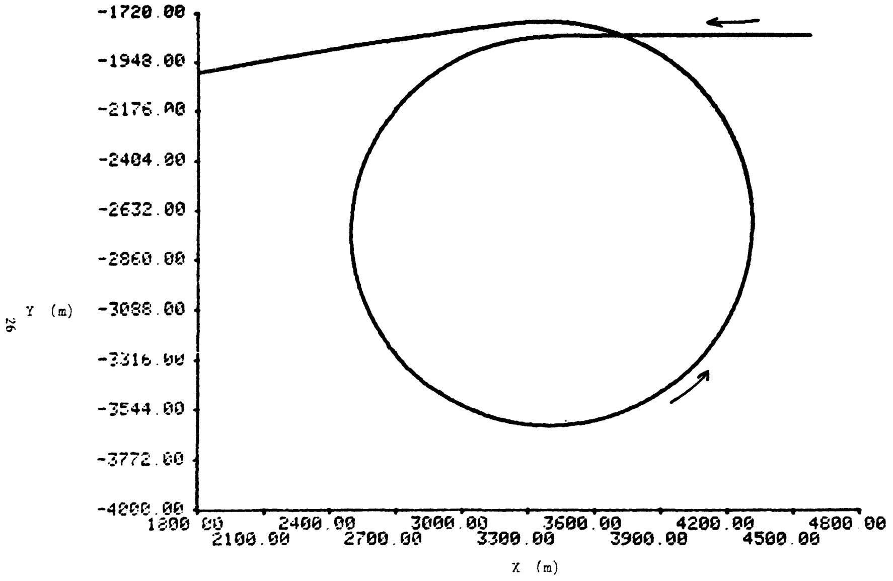
(b) X-Y trajectory flown: TAFOS ATC off.
