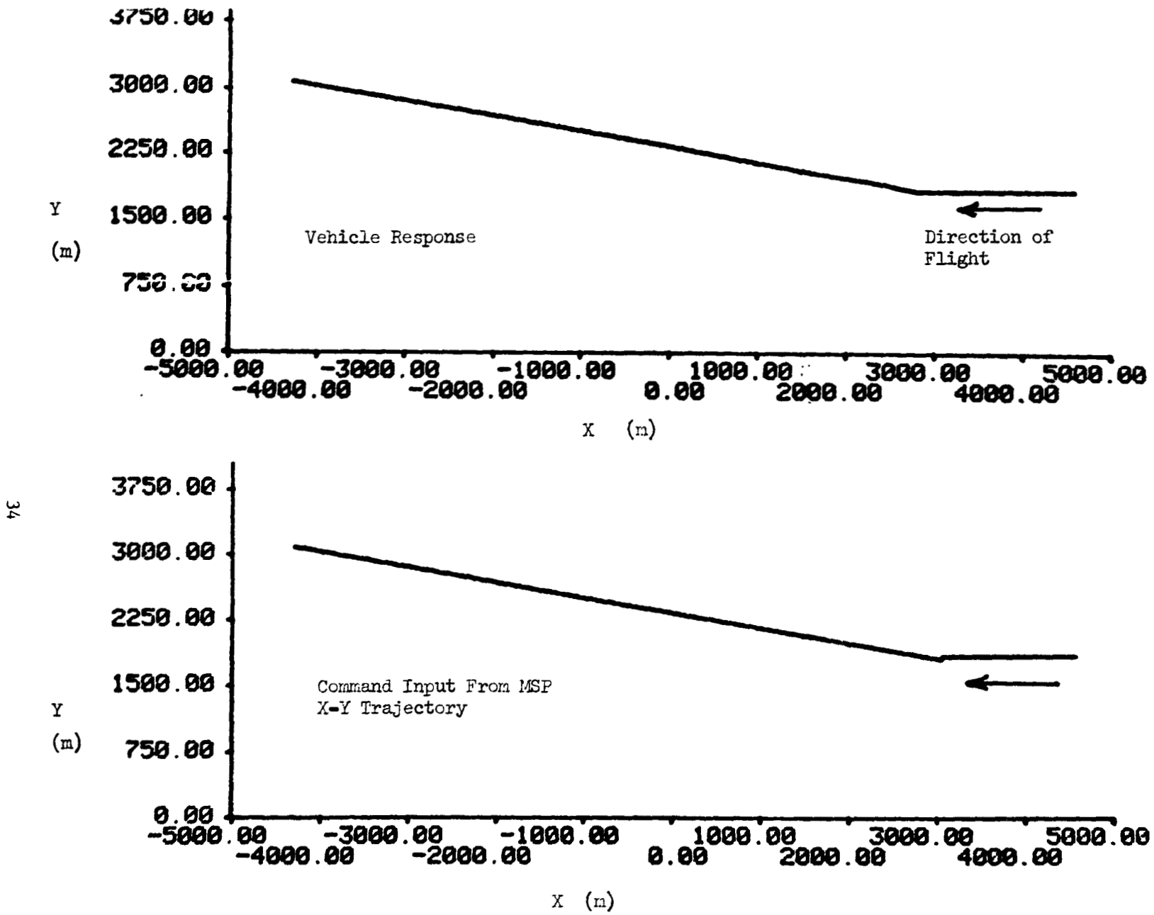
(a) Small heading on command, \psi = 180^\circ to 190^\circ .
