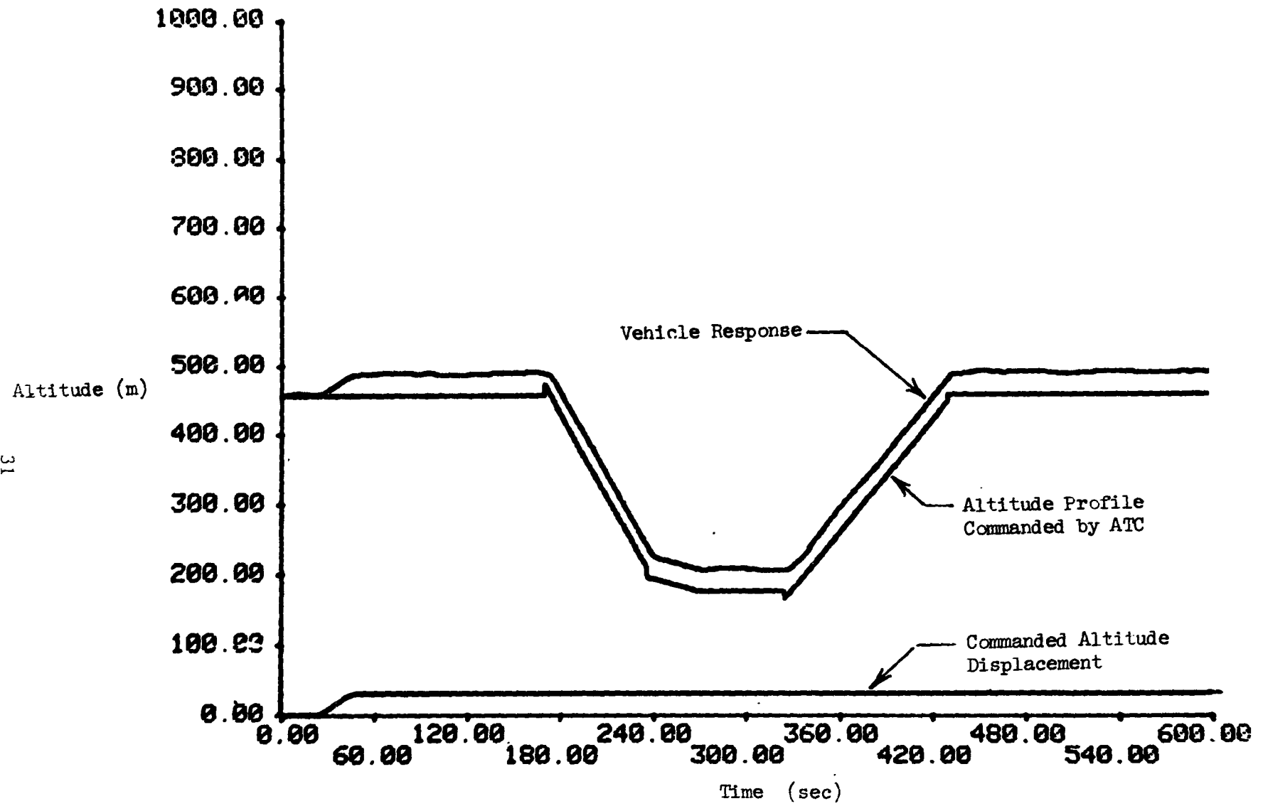
(b) Altitude plots. Figure 10.- Concluded.
