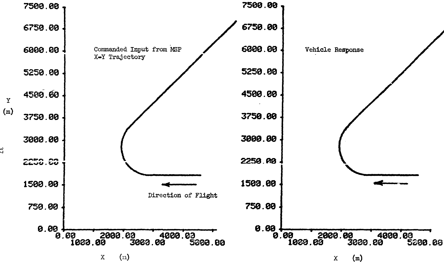
(d) Commanded heading change, large angle, \psi = 180^\circ to 315^\circ .
