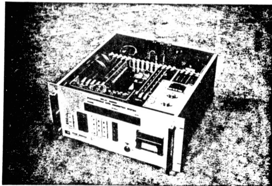
Figure 1. Existing solar heating and control subsystem was implemented in a solar energy data acquisition system.
