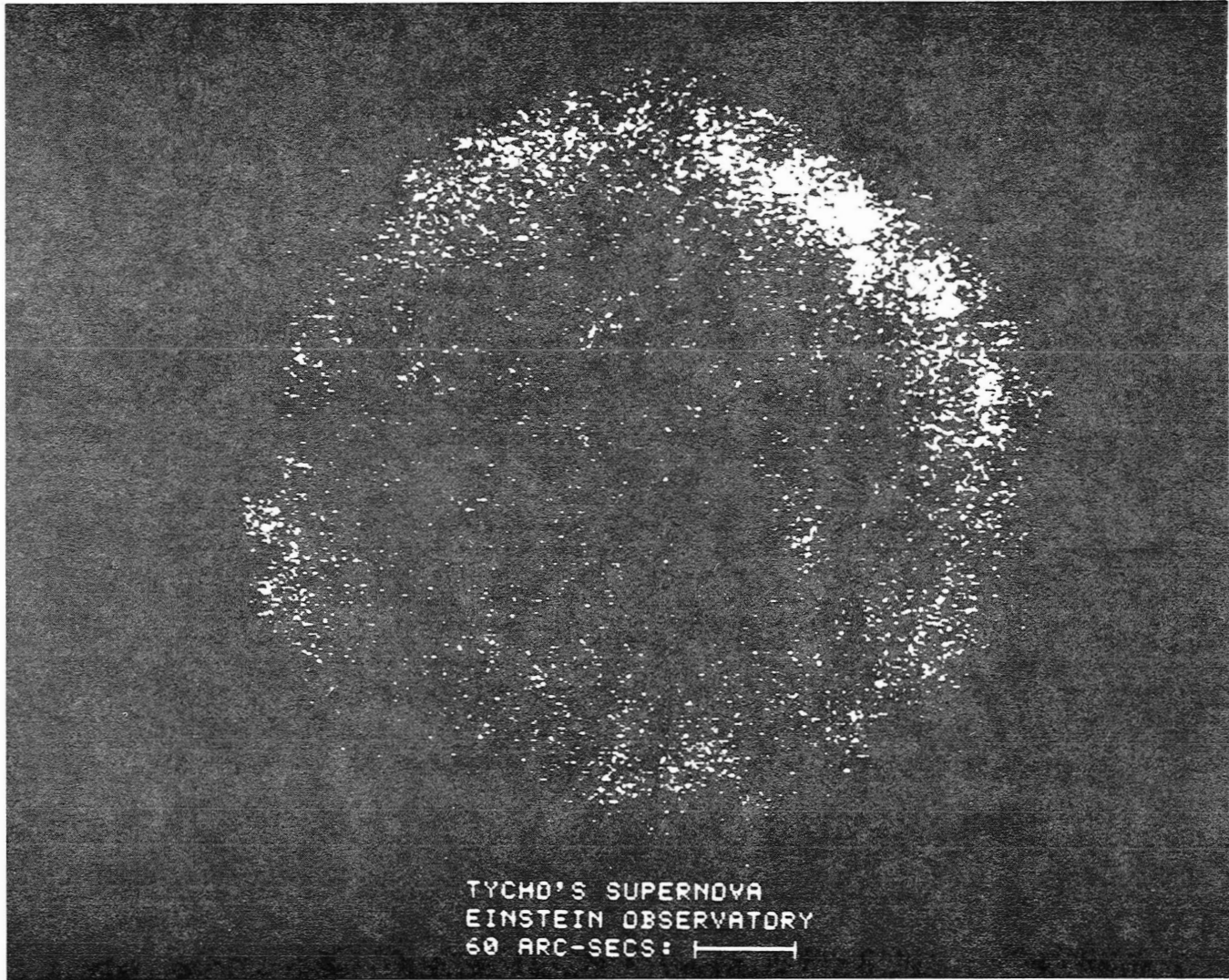
Figure 3. HRI picture of Tycho SNR. Exposure approximately 4 \times 10^4 sec.
