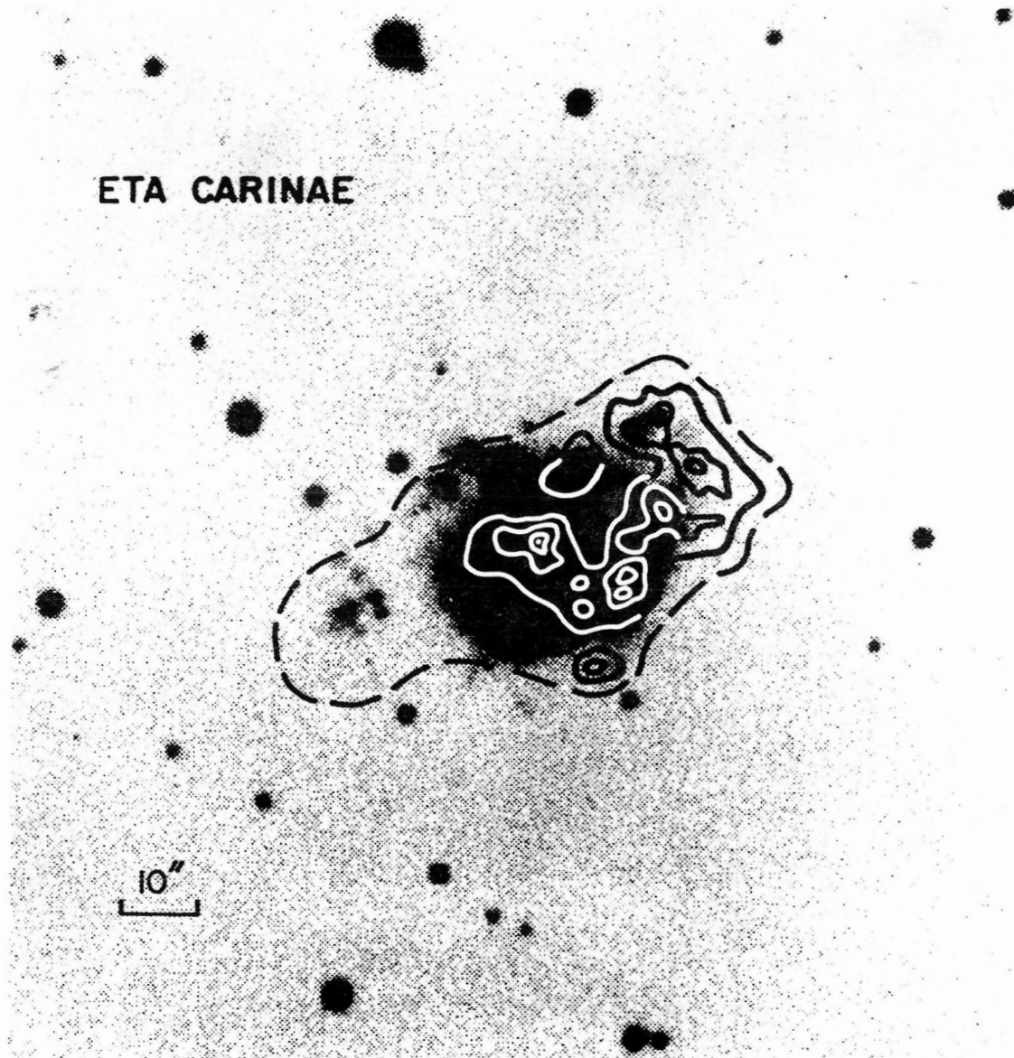
Figure 13. Contours of constant X-ray emission overlaid on an optical photograph of Eta Carinae taken from Walborn (1976).
