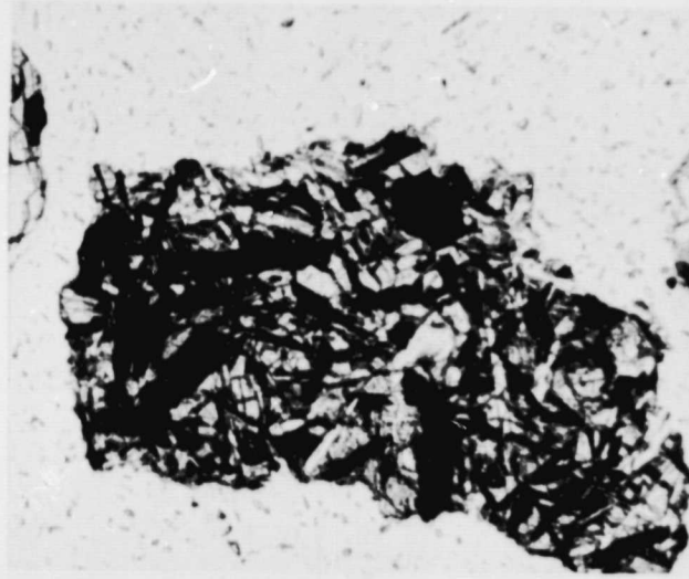
BASALT FRAGMENT TRANSMITTED LIGHT
