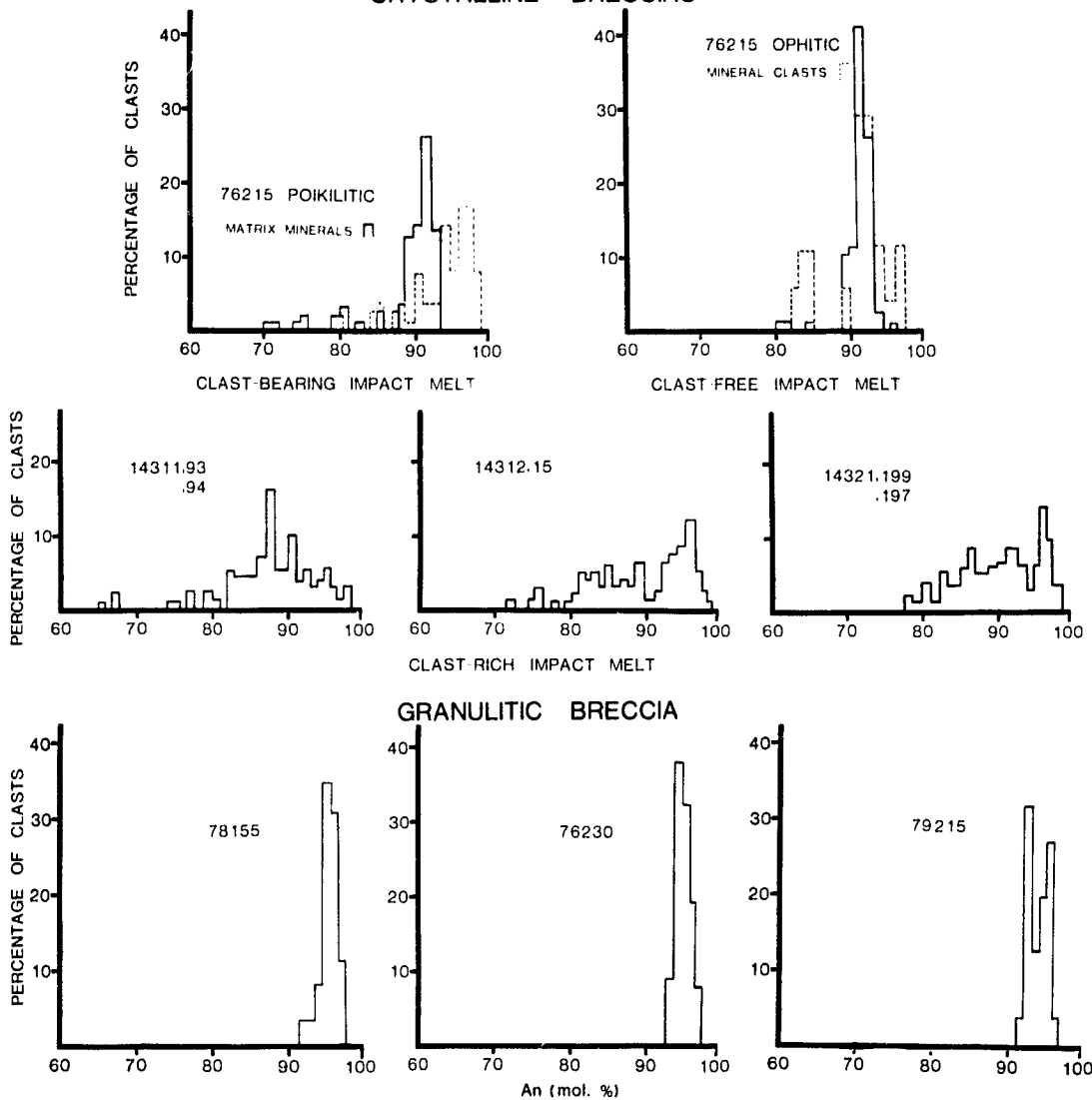
FIGURE 8. COMPOSITIONS OF PLAGIOCIASE GRAINS IN FRAGMENTAL, CRYSTALLINE AND GRANULITIC BRECCIAS. DATA FROM: SIMONDS (1975); SIMONDS et al. (1977); BICKEL et al. (1976); BICKEL (1977).
