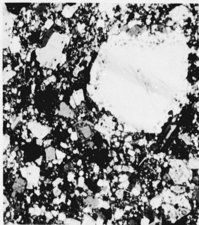
Figure 76315b. Micro-poikilitic matrix in 76315; reflected light. Dark-grey plagioclase; lt-grey, pyroxene; white, ilmenite.
