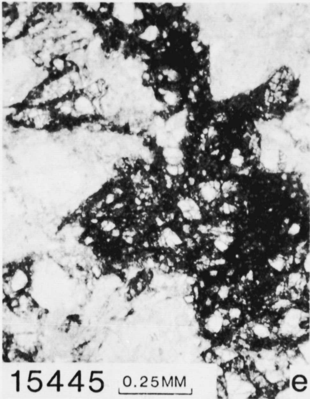
Figure 15445e. Brecciated norite clast; transmitted light.
