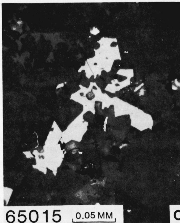
Figure 65015c. Poikilitic ilmenite (white) in 65015; reflected light; color key same as in (b).
