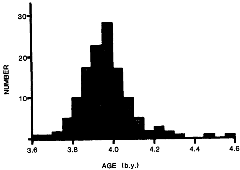
Figure 18. Distribution of highland ages as determined from ^{87}\text{Rb}/^{87}\text{Sr} isochrons and the ^{39}\text{Ar}-^{40}\text{Ar} plateaus, using data from the literature. Some ages in the 3.6-3.8 range may be younger igneous mare rocks transported to the highlands by distant impacts. A few ages >4.2 b.y. appear to have survived the intense rate heavy bombardment. Adapted from Wetherill (1975).
