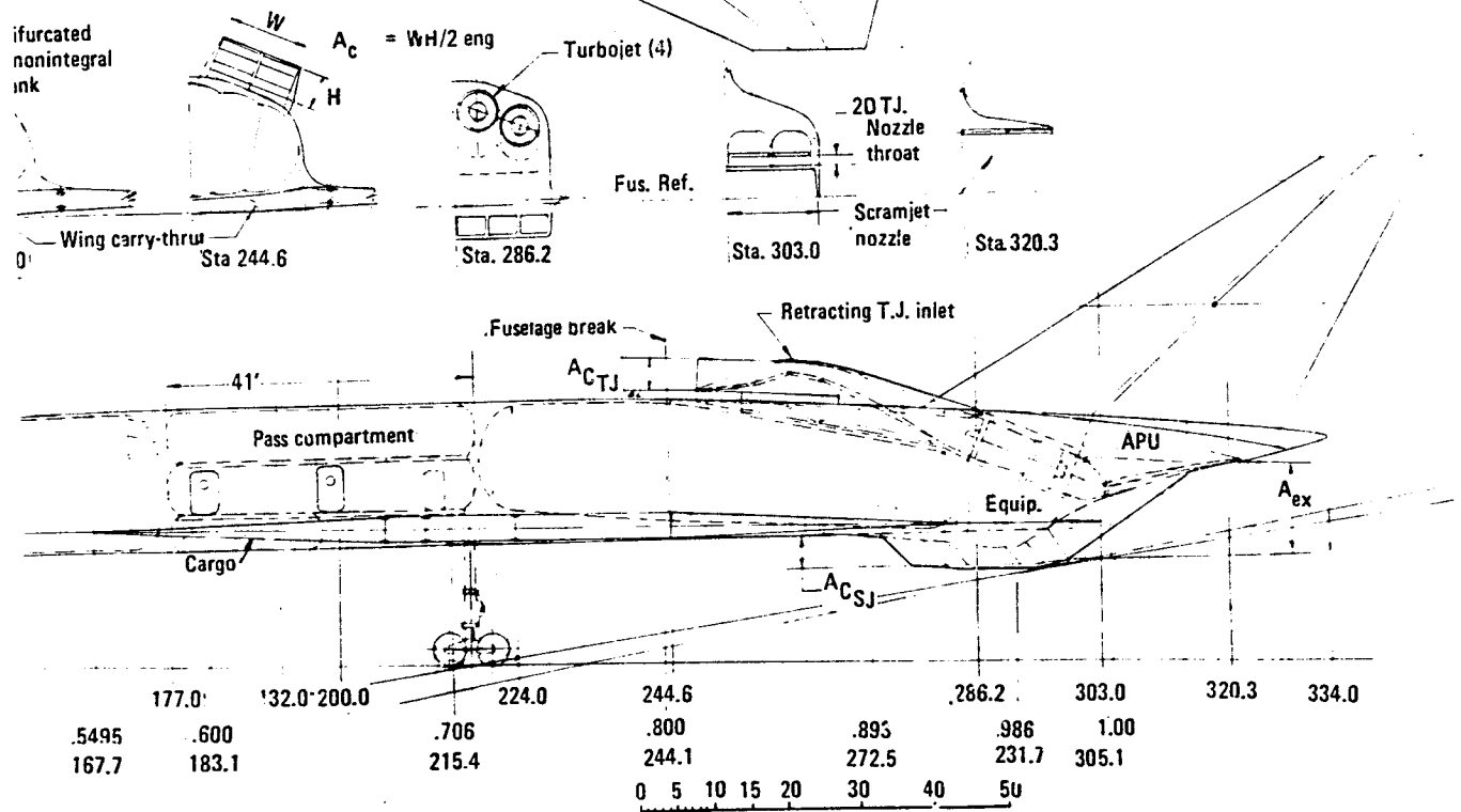
Figure 4. - HYCAT-2 general arrangement
