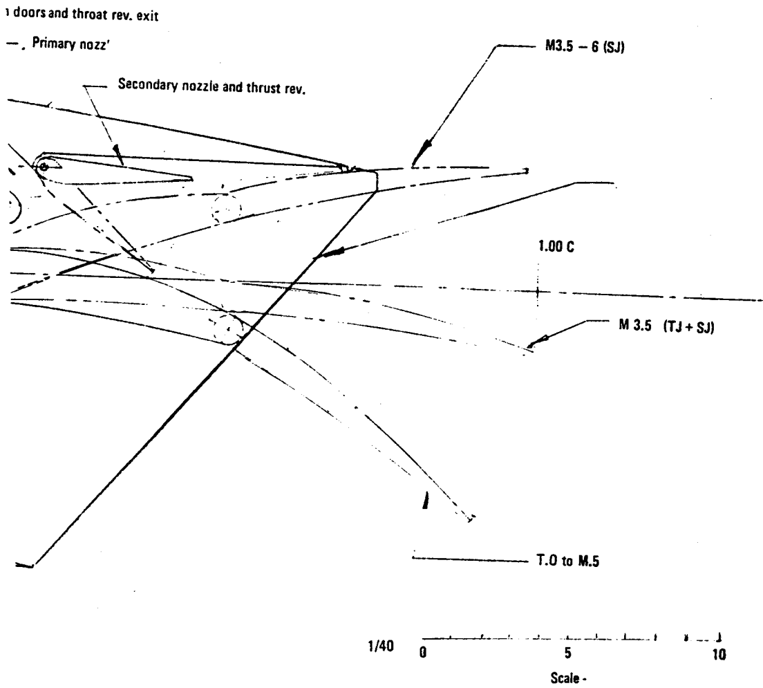
Figure 9. HYCAT-4 propulsion installation.
