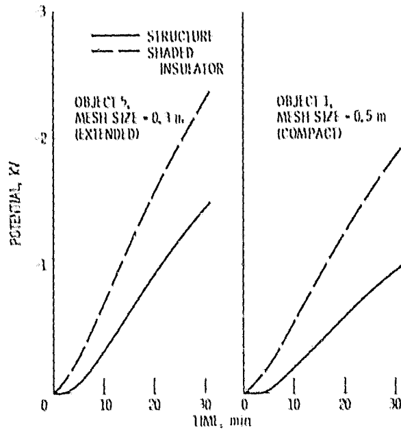
Figure 13. - Effect of geometry type on charging response.
