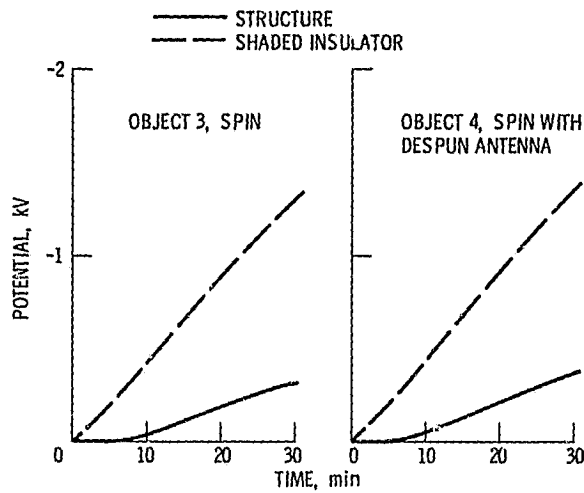
Figure 11. - Effect of despun antenna on charging response. Sun 1, 0, 0.
