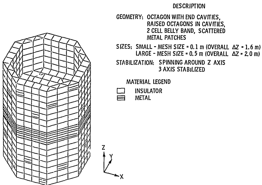
Figure 3. - Object 1 (ATS-5 model object)
