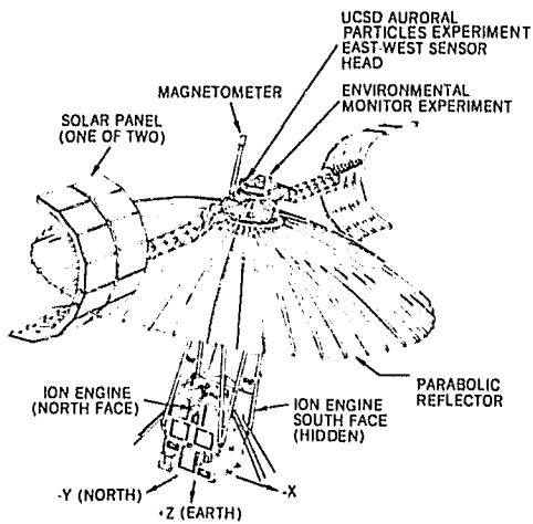
Figure 2. - ATS-6 orbital configuration.
