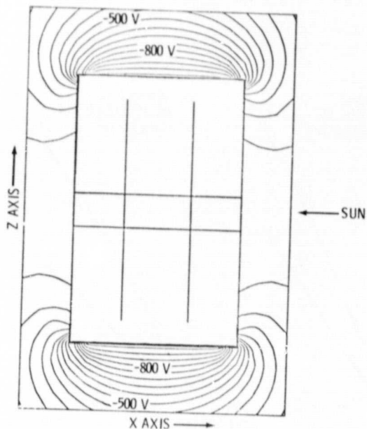
Figure 15. - Potential contours after 21 minutes of charging.
