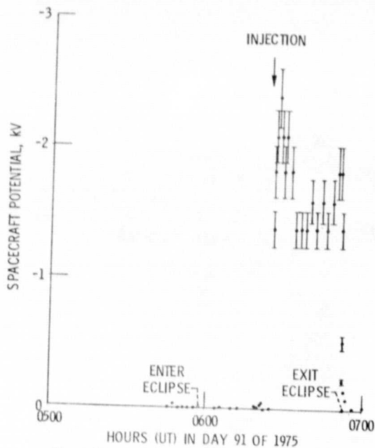
Figure 17. - ATS-6 potential: response to injection during eclipse.
