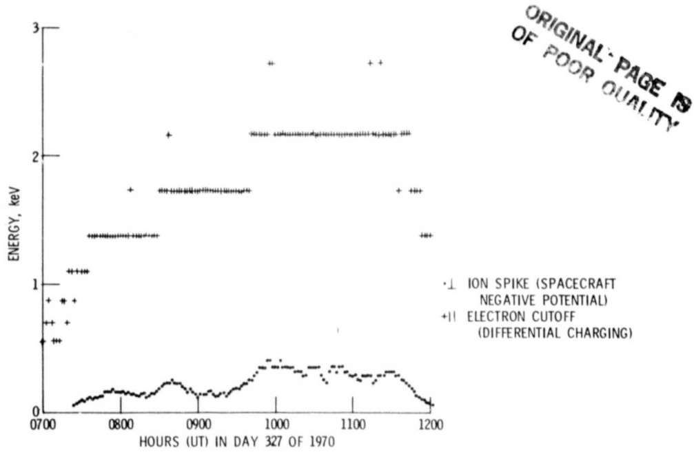
Figure 22. - ATS-5 data: charging in sunlight.
