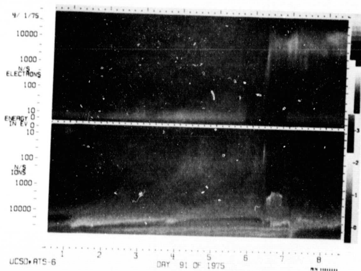
Figure 16. - ATS-6 spectrogram, day 91 of 1975: injection during eclipse.
