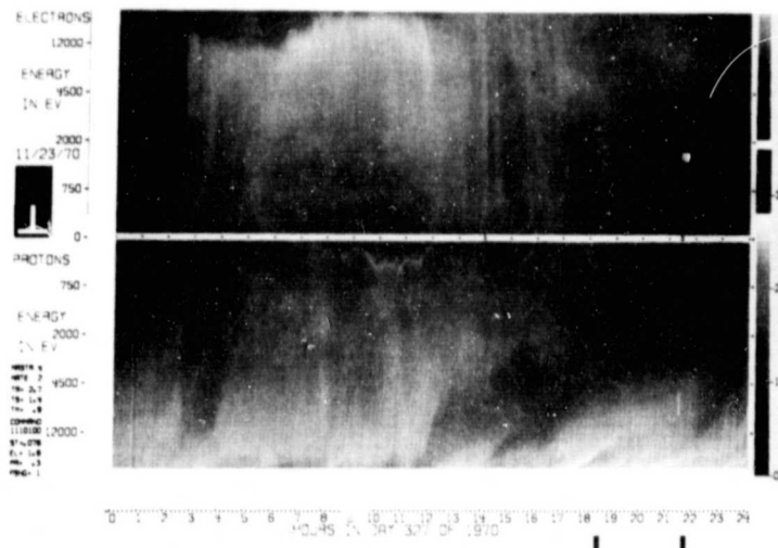
Figure 21. - ATS-5 daylight charging data, perpendicular detector.
