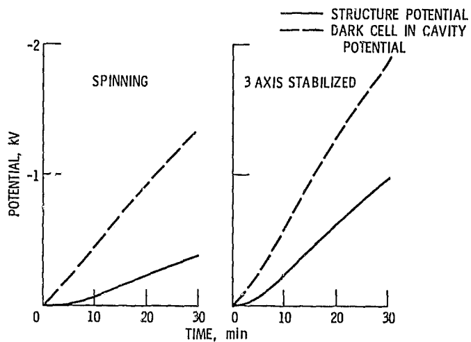
Figure 8. - NASCAP predictions: sunlight charging; effect of stabilization type. CS-79-4381
