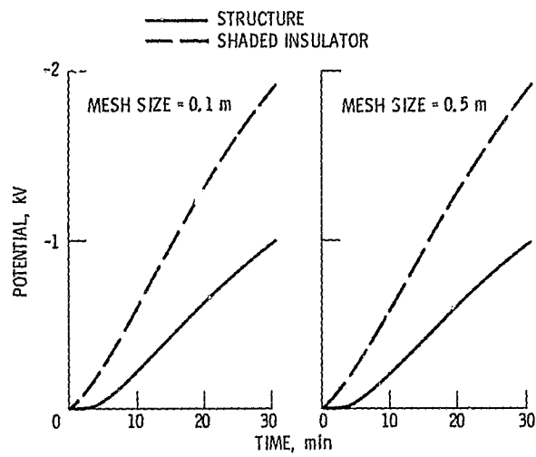
Figure 12. - Effect of size on charging response. Object 1, 3 axis stabilized. Sun at 1, 0, 0.
