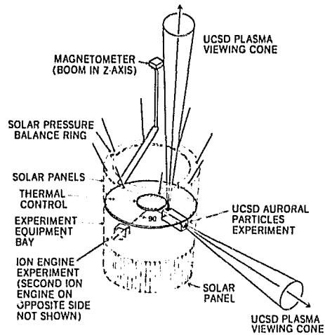
Figure 1. - ATS-5 orbital configuration.
