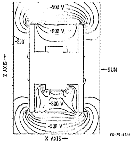
Figure 14. - Potential contours after 20 minutes of charging.
