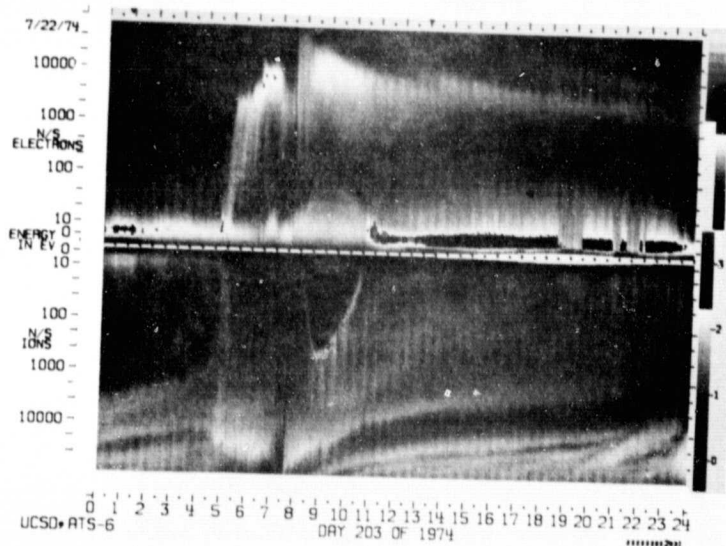
Figure 18. - ATS-6 spectrogram: daylight charging.
