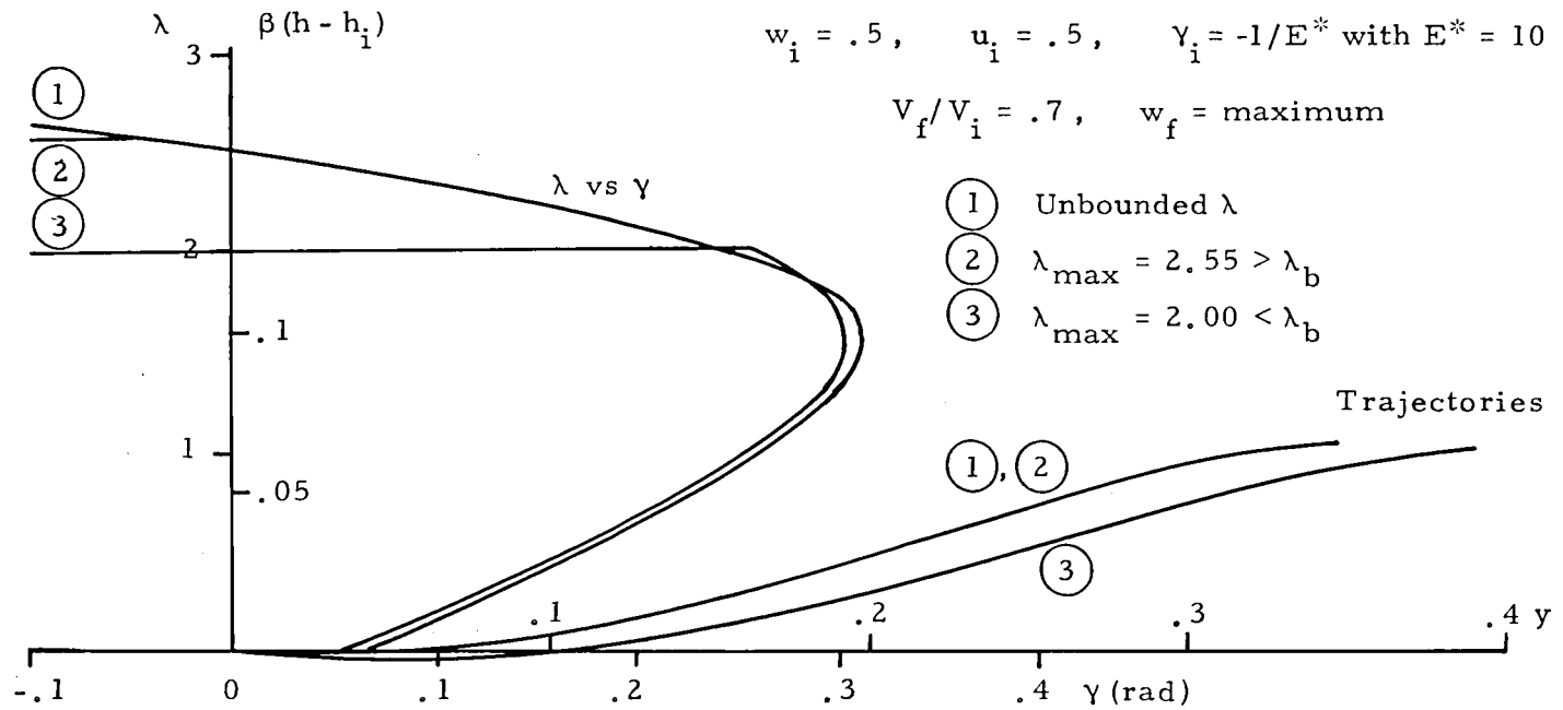
Figure 8. - Pull-Up Maneuver with Bounded \lambda ; Trajectories in the Physical Space \beta(h - h_i) vs y , and Variation of the Optimum Bounded Lift Control.
