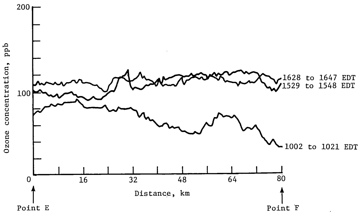
Figure 17.- Ozone data for leg E → F at 560-m altitude on July 21, 1978.
