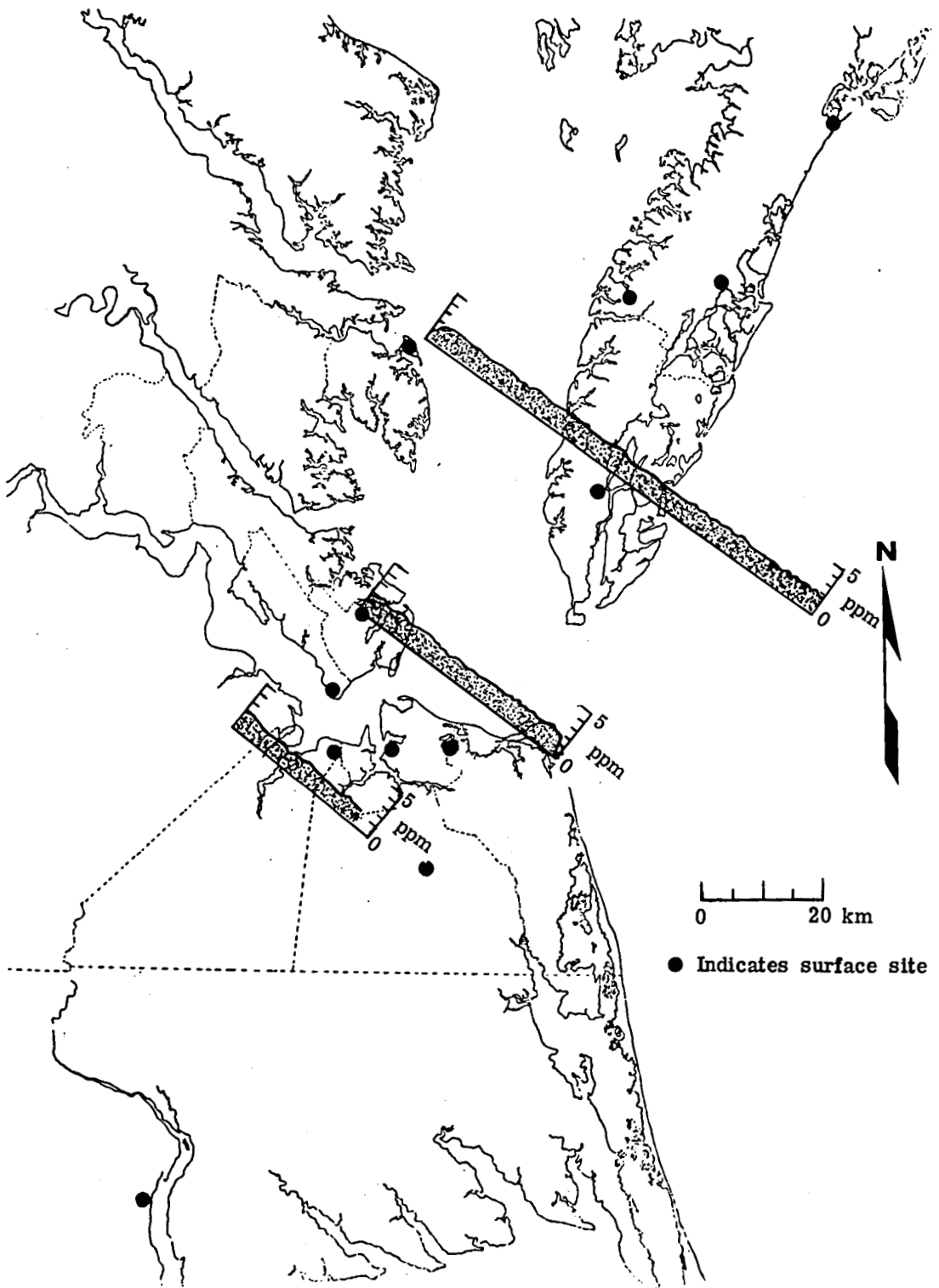
Figure 24.- Methane data on morning of July 27, 1978.
