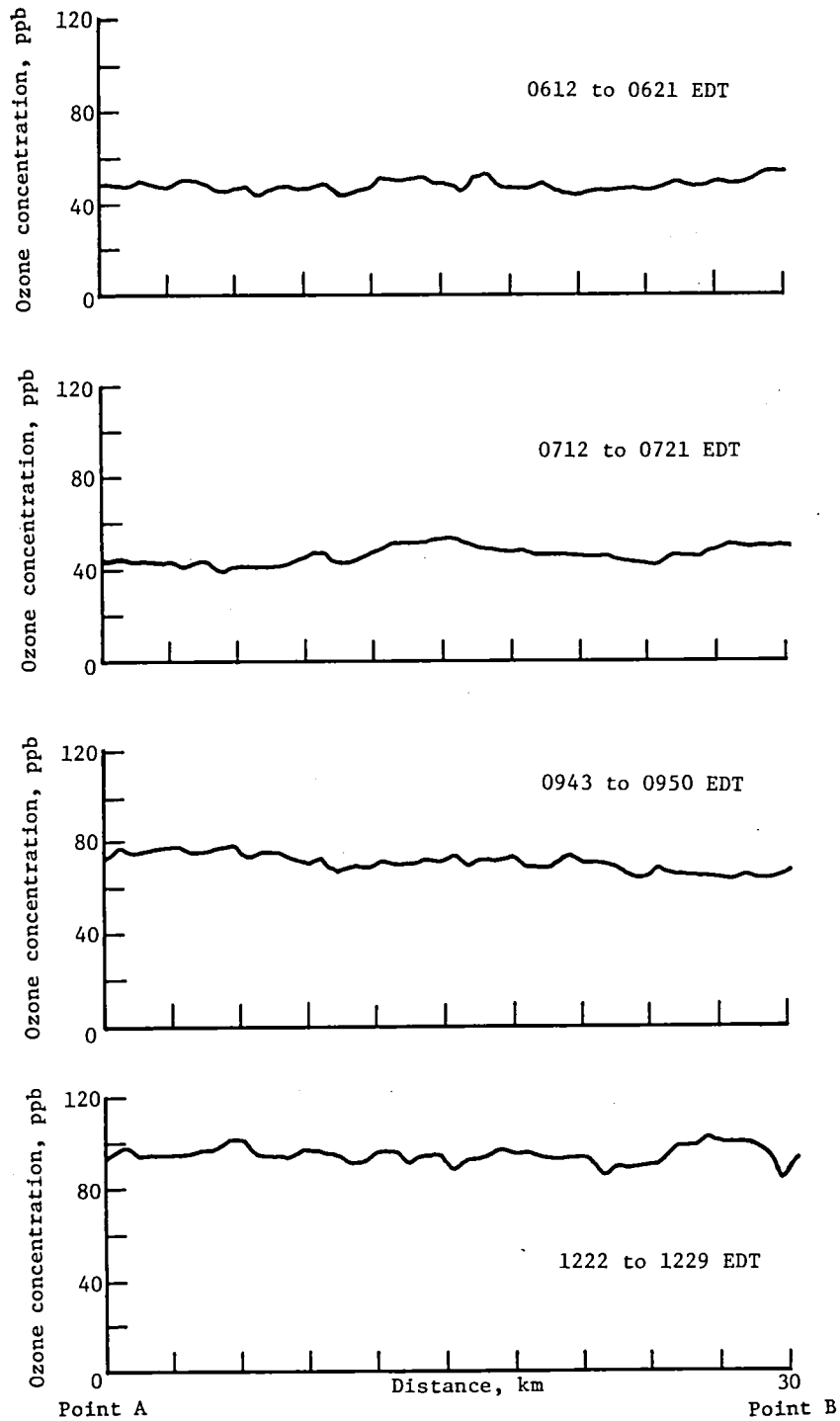
Figure 19.- Ozone concentration on leg A → B for photochemical oxidant box experiment on July 24, 1978.
