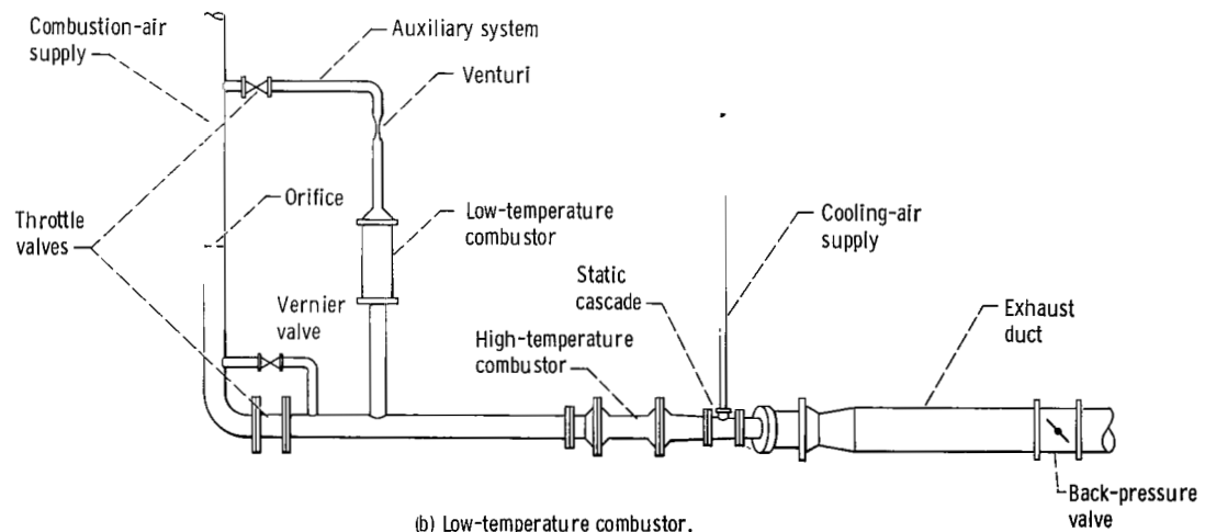
Figure 1. - Cascade facility.
