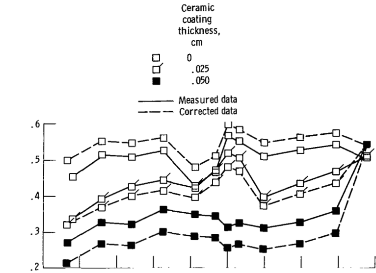
(a) High gas Reynolds number; turbulent flow (CTOL takeoff conditions, case C).
