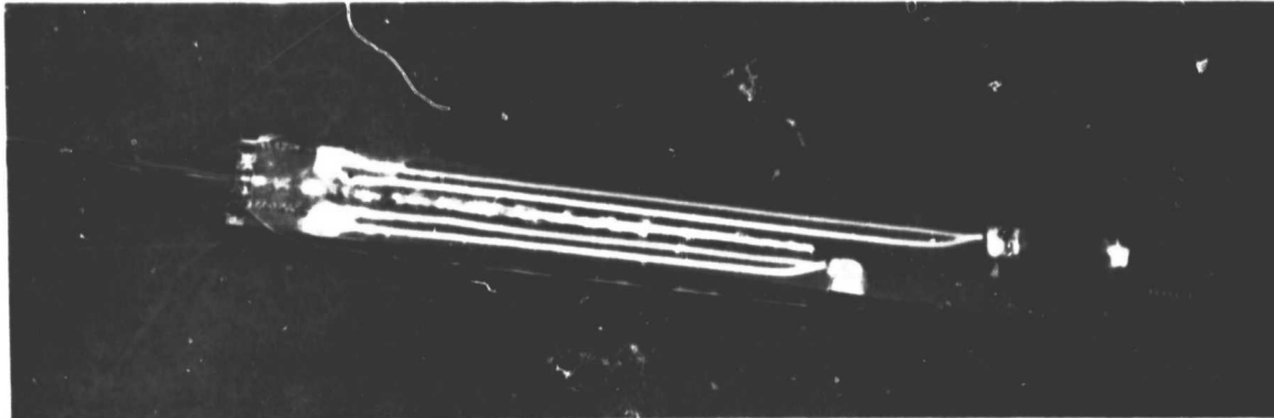
Figure 8 Simulated Turbine Blade 4R 1 Instrumented with Two Thin Film Temperature Sensor Systems and Five Reference Wire Thermocouples - Two of the thermocouples are buried in the central groove.
