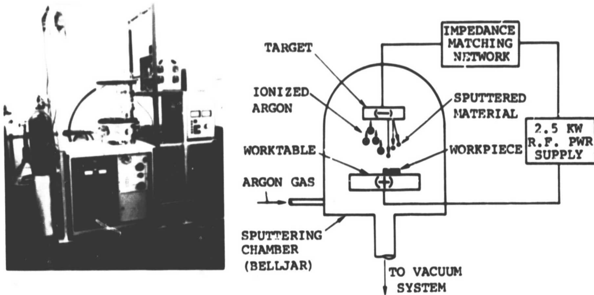
Figure 2 Sputtering Apparatus
