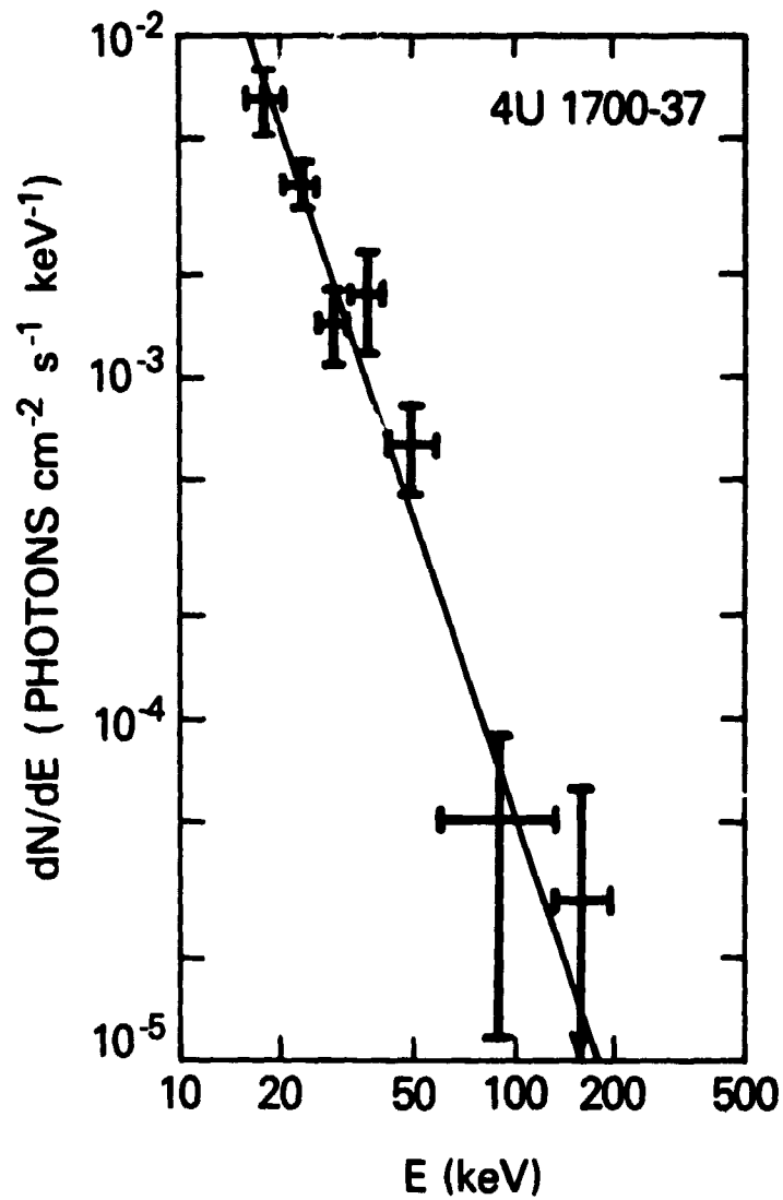
Figure 3. The photon-number spectrum of 4U1700-37 observed 1978 September 1 to 11 outside of eclipse. The straight line is the power law given in Equation (1) in the text which acceptably represents the data. The error bars represent \pm one standard deviation uncertainties derived from the statistics alone.
