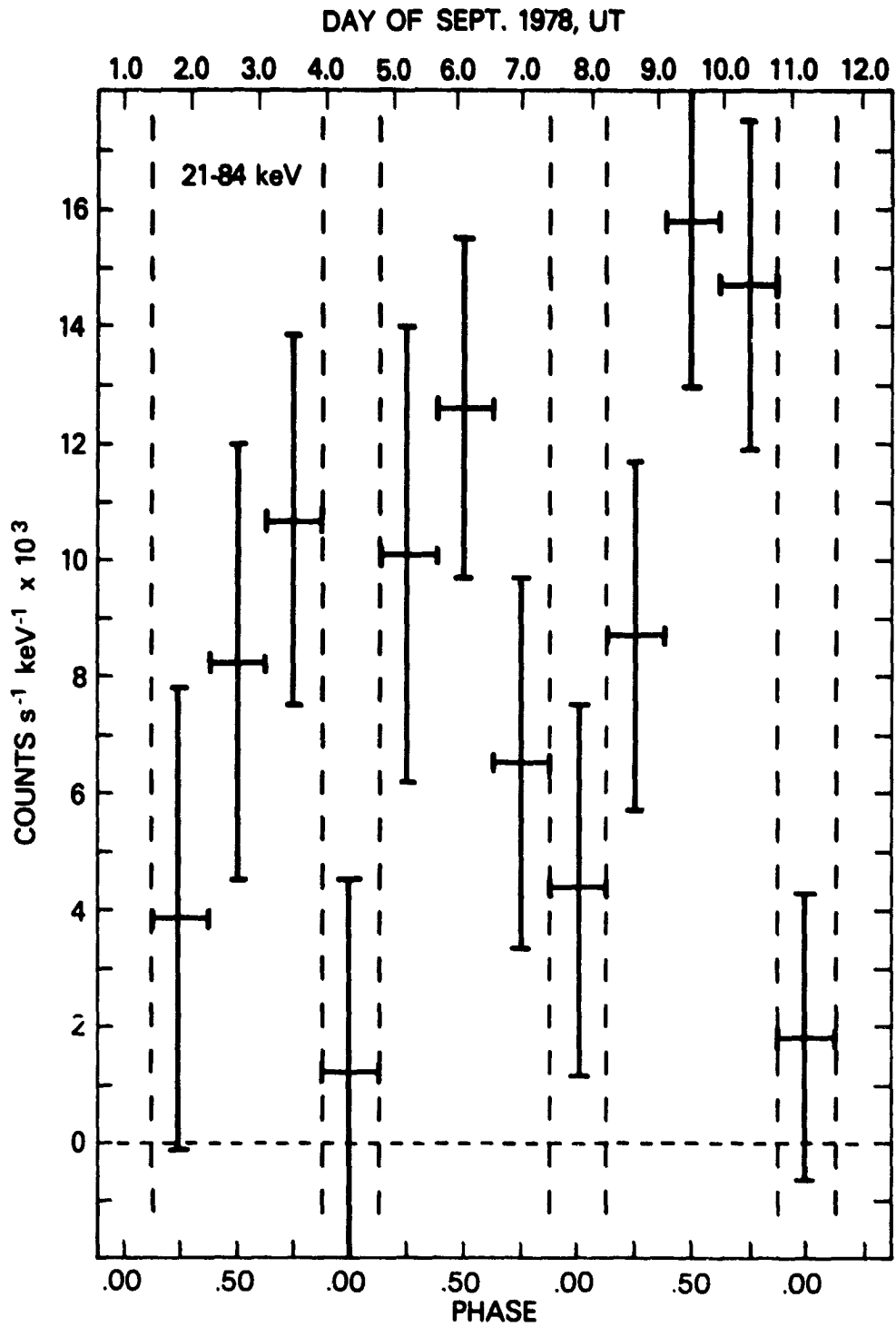
Figure 1. The 21 to 84 keV counting rate observed from 4U1700-37, 1978 September 1 to 11. Orbital phase is calculated from the ephemeris given in the text. Eclipses occur in low-energy x-rays between phases 0.875 and 0.125; these intervals are demarcated by the vertical dashed lines. The error bars represent \pm one standard deviation uncertainties derived from the statistics alone.
