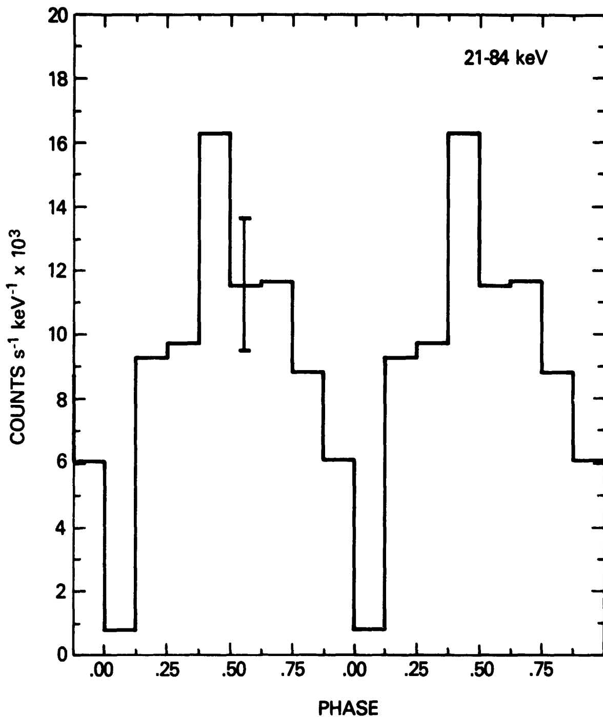
Figure 2. The data included in Figure 1, folded modulo the orbital period of 4U1700-37. Eclipses in low energy x-rays occur centered on phase 0.0. All phase bins have \pm one standard deviation uncertainties derived from the statistics alone similar to the error bar shown. The same data points are repeated twice for clarity.
