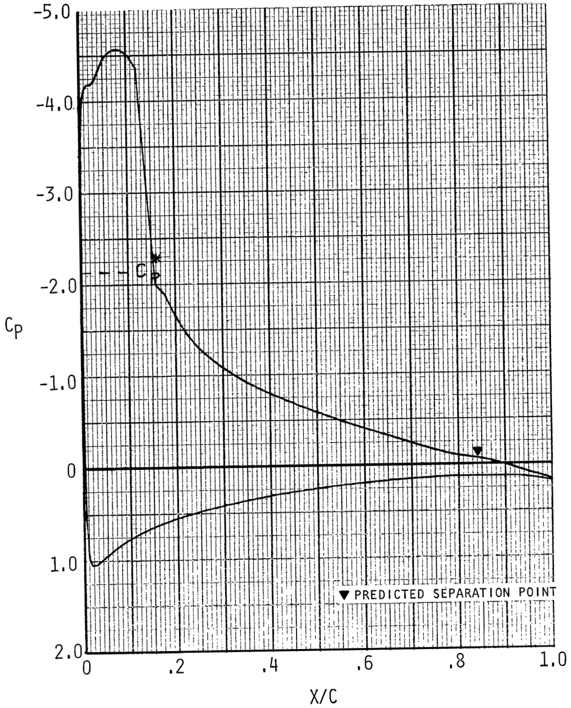
c. M = 0.50 , C_{\ell} = 1.5 , R_N = 5 \times 10^6 Figure 26. - Continued.
