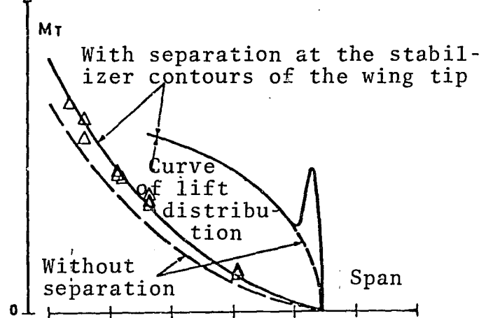
FIG. 38 Structural Loading Movement of Wing Flexure
