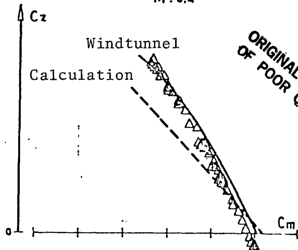
FIG. 16 Static Longitudinal Stability
