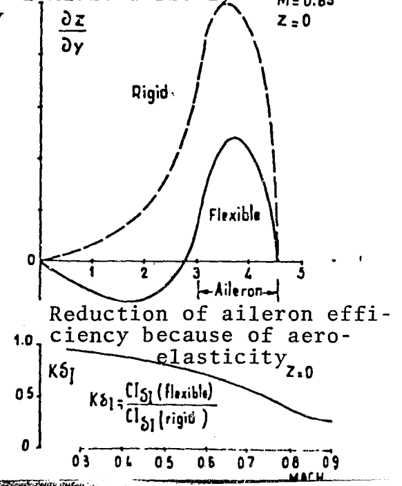
FIG. 5. Lift Distribution Due to Aileron Deflection (comparison between a rigid and a flexible airfoil) M=0.85 Z=0
