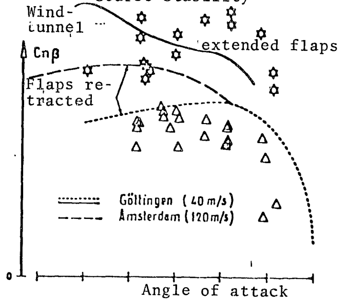
FIG. 28 Course Stability
