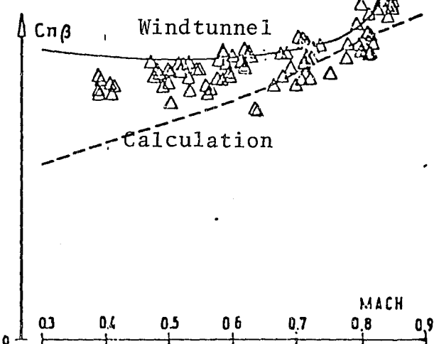
FIG. 22 Course Stability
