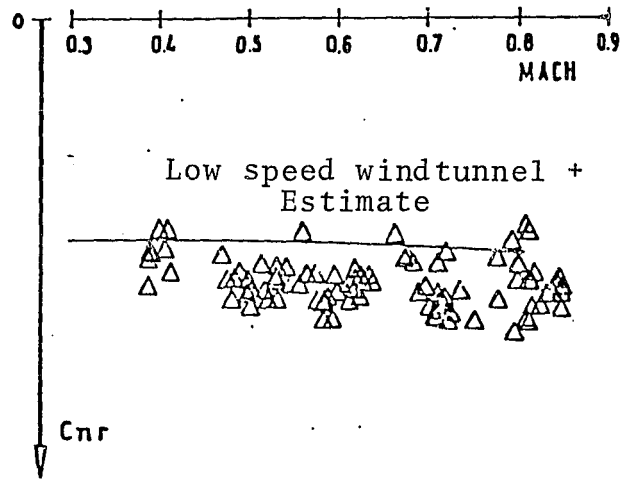
FIG. 20 Yaw Damping
