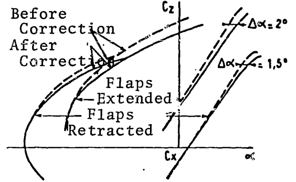
FIG. 4. Example of Interactions with the Windtunnel Walls
