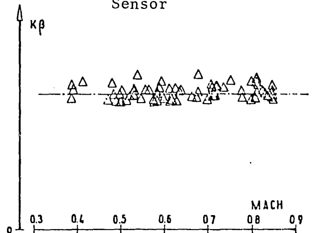
FIG. 34 Calibration of Side Slip Sensor
