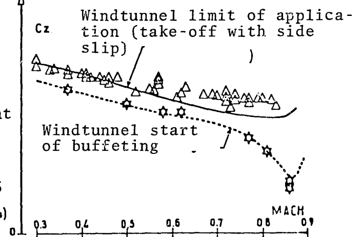
FIG. 40 Boundaries of Buffeting and of Application
