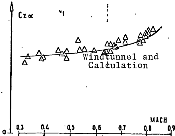
FIG. 11 Lift
