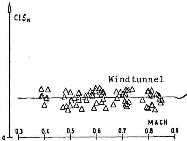
FIG. 31 Roll Due to Rudder
