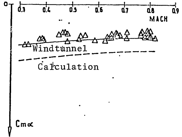
FIG. 12 Static Stability
