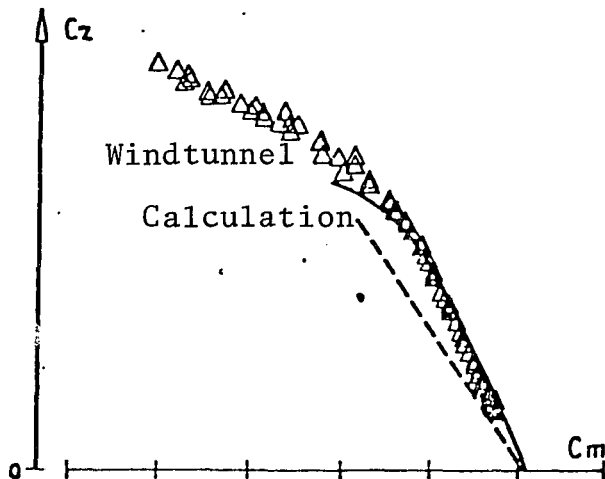
FIG. 15 Static Longitudinal Stability
