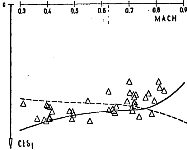
FIG. 29 Aileron Efficiency
