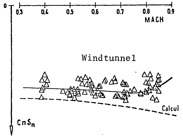
FIG. 32 Rudder Efficiency
