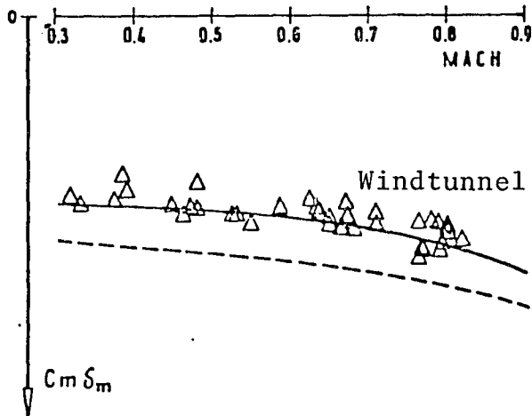
FIG. 33 Elevator Efficiency
