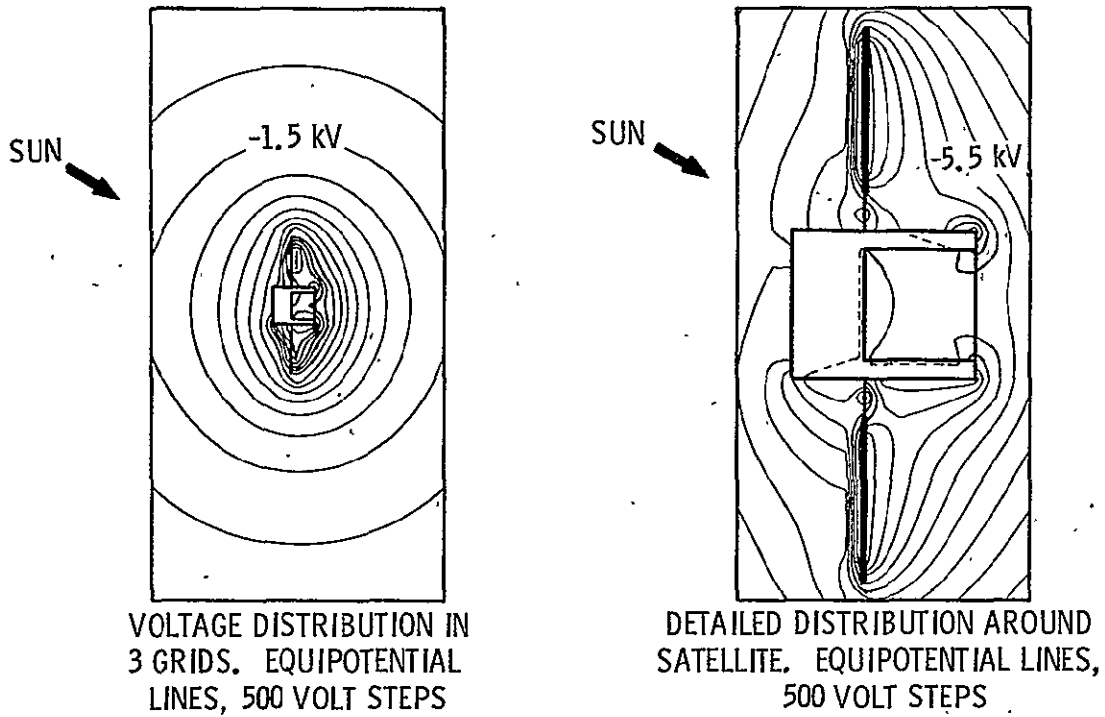
Figure 8. - Voltage distributions around satellite. Severe substorm charging for 30 minutes ( T_e = 8 keV; T_p = 16 keV; n_e = n_p = 2.0 \text{ cm}^{-3} ).
