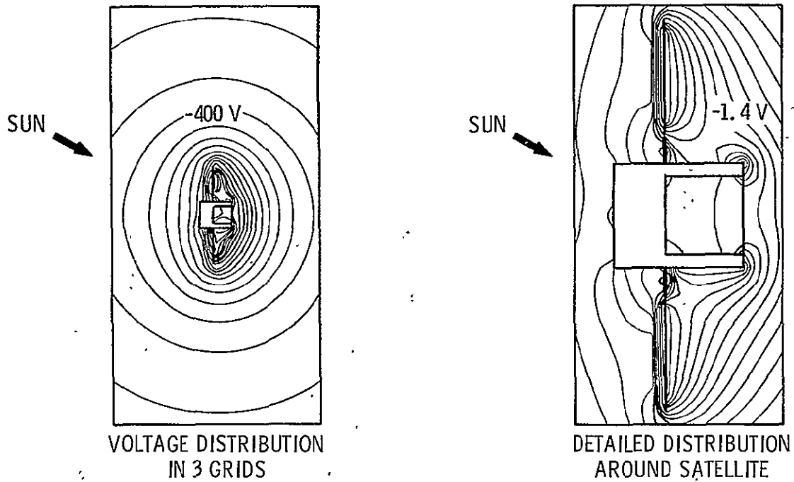
Figure 5. - Voltage distributions around satellite in moderate substorm charging for 20 minutes ( T_e = 3 keV; T_p = 6 keV; n_e = n_p = 1.0 cm 2 ): Equipotential lines at 100 volt steps.
