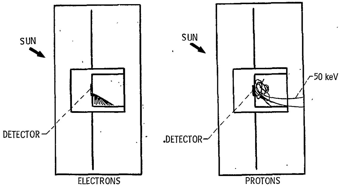
Figure 9a. - Charged particle trajectories incident on mirror. Severe substorm charging. Particle energies: 1 eV to 50 keV.
