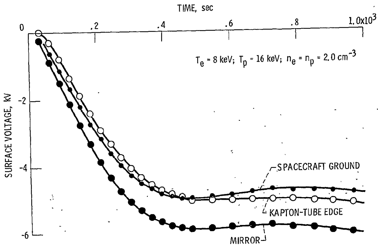
Figure 11. - Charging characteristics of satellite. Severe substorm charging (solar arrays rotated 90°).
