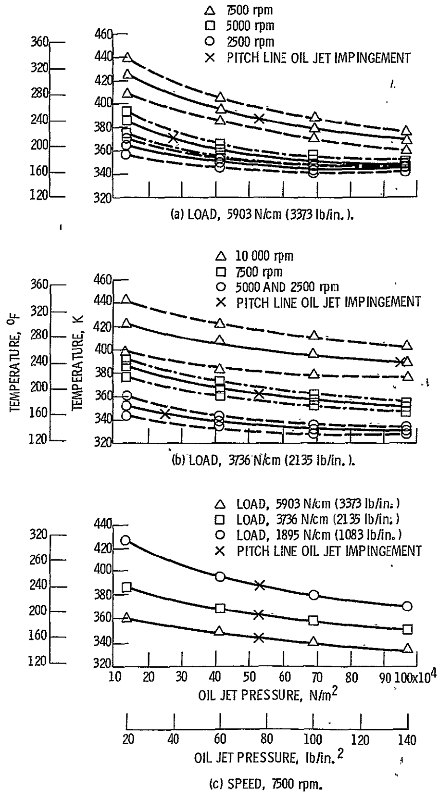
Figure 8. - I. R. microscope measurements of gear surface temperature versus oil jet pressure, inlet oil temperature 308 K (95 ^{\circ} F), oil jet diameter 0.04 cm (0.016 in.).
