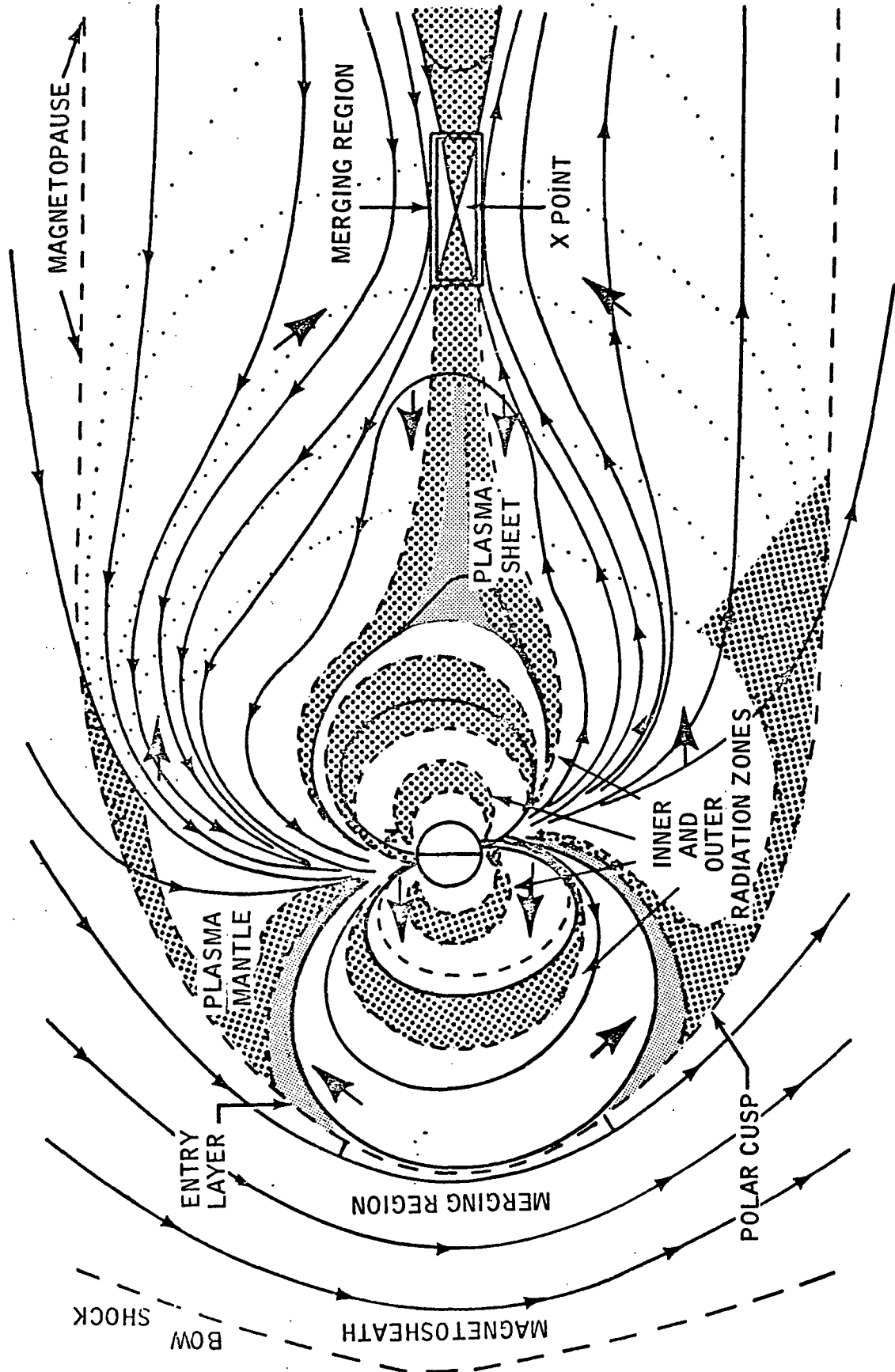
EARTH'S MAGNETOSPHERE AND SOLAR WIND INTERACTION NOTE: CONVECTIVE PLASMA FLOW . . . . .
