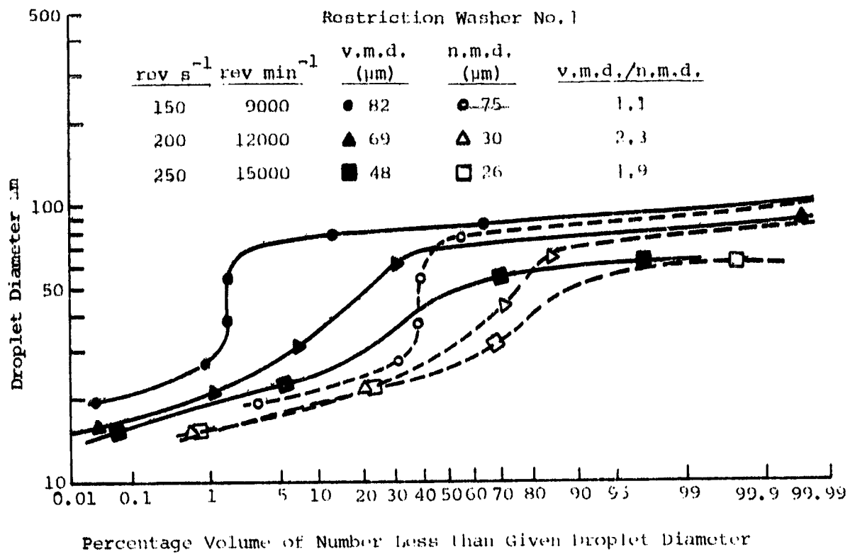
Figure 2.13 Droplet distribution using a rotary atomizer and restriction washer #1.
