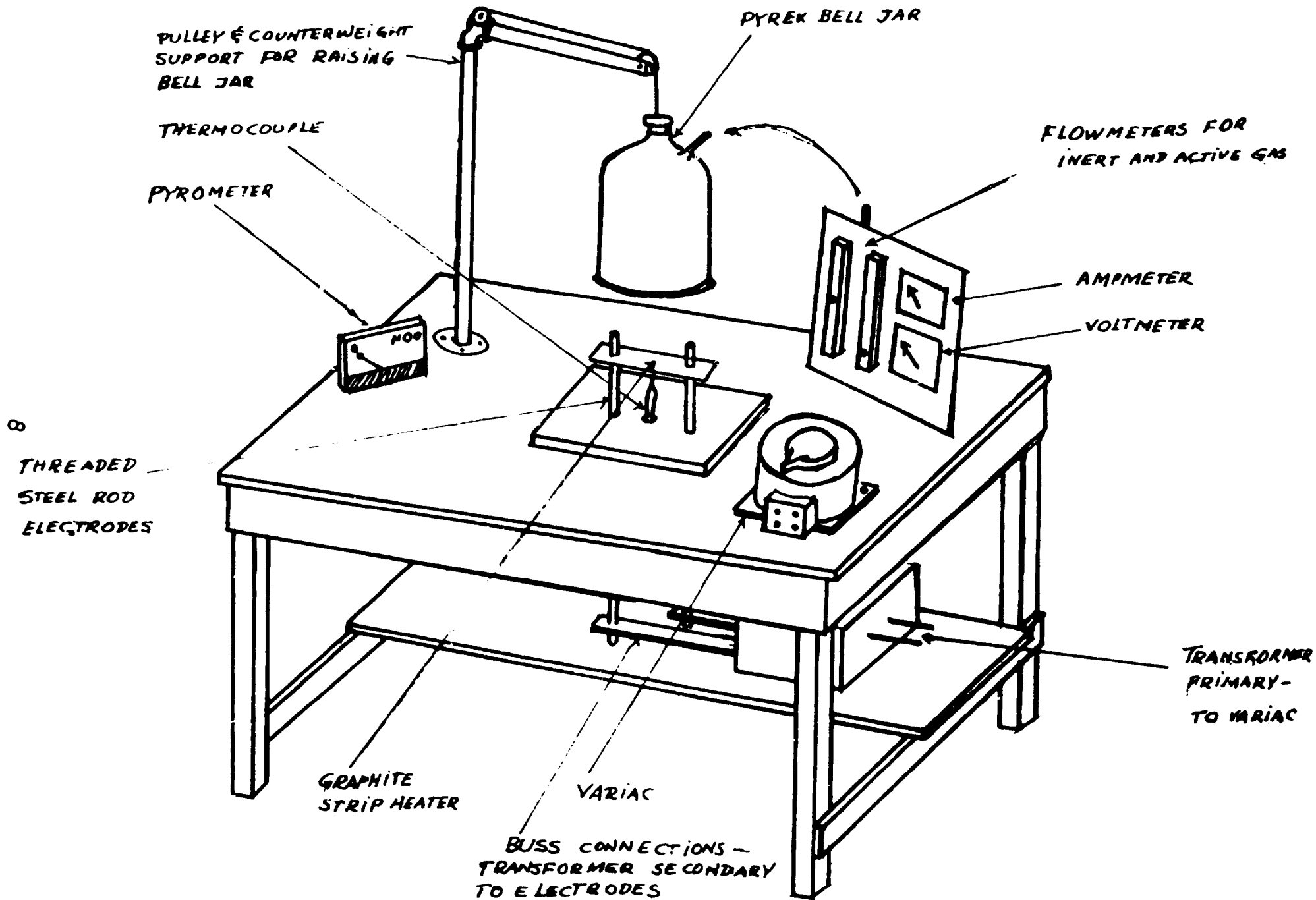
CONTROLLED ATMOSPHERE EXPERIMENTAL STRIP HEATER
