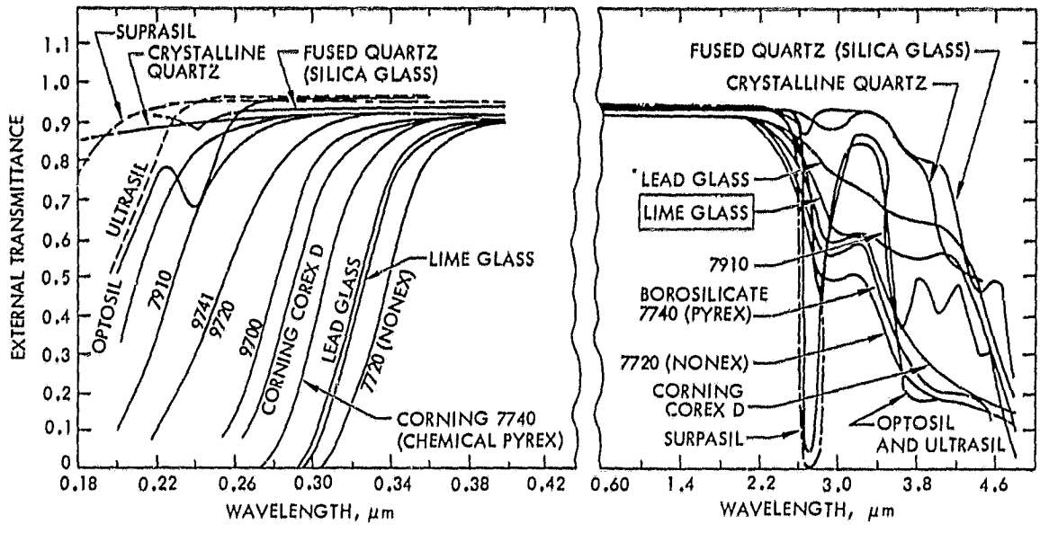
Figure 16. The External Transmittance of Several Samples of Corning and Amersil Glasses (Ref. 8)
