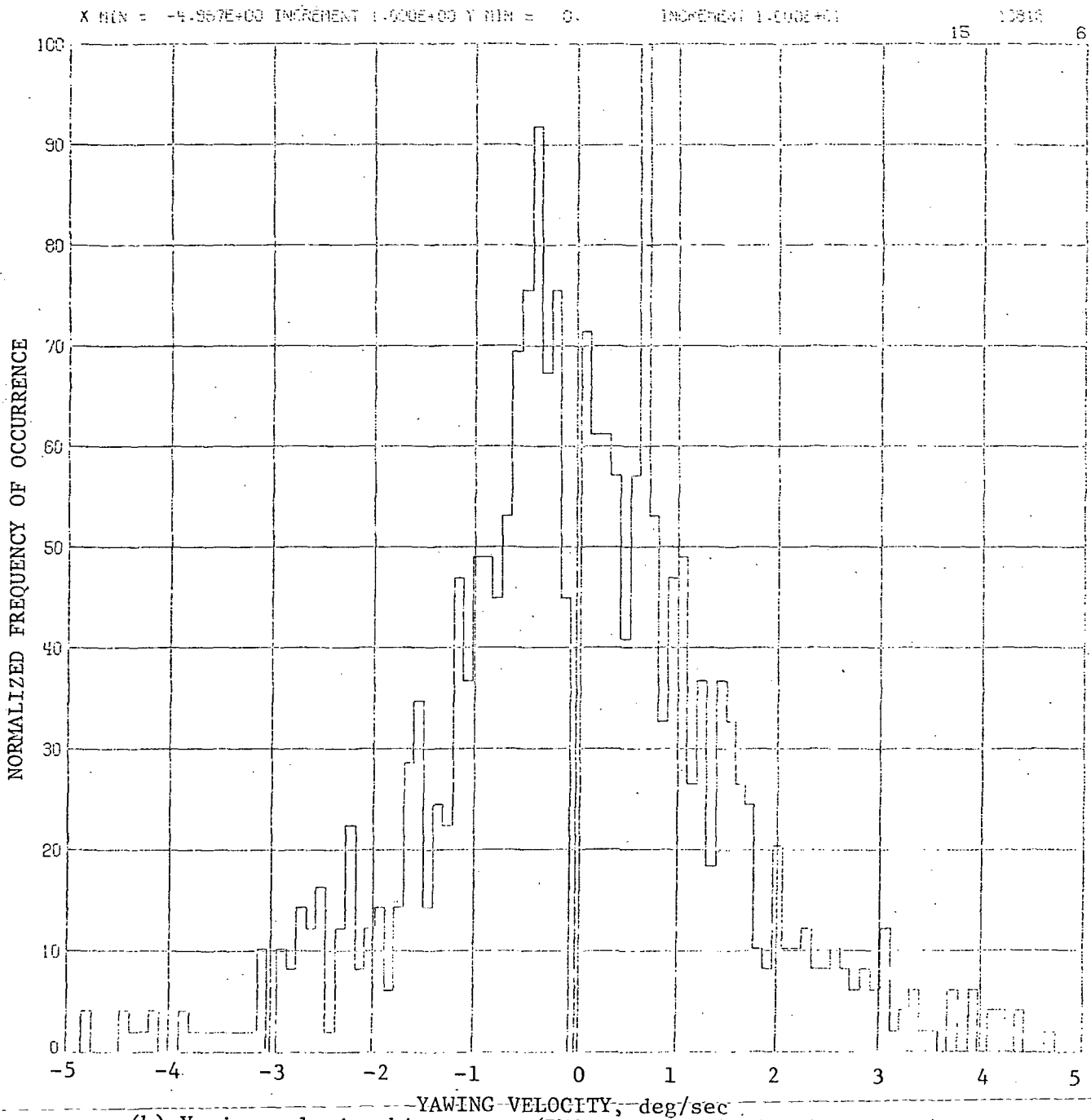
(b) Yawing velocity histograms (RMS yawing velocity 1.247 deg/sec)
