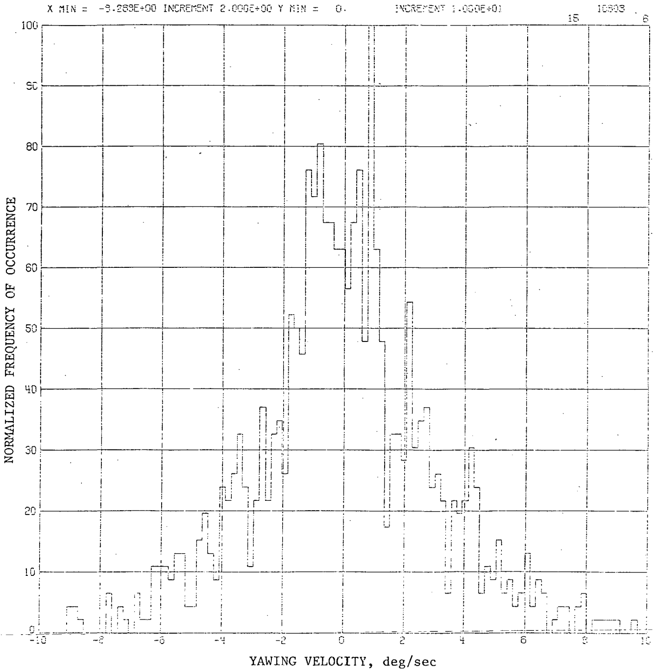
(b) Yawing velocity histograms (RMS yawing velocity 2.997 deg/sec)
