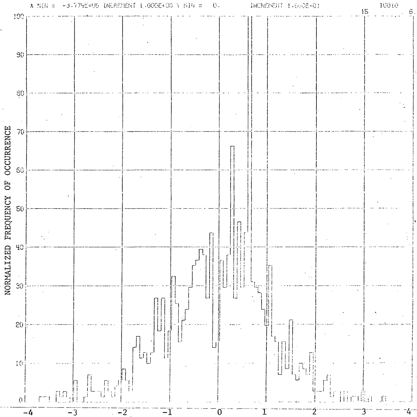
(b) Yawing velocity histograms (RMS yawing velocity 0.976 deg/sec)
