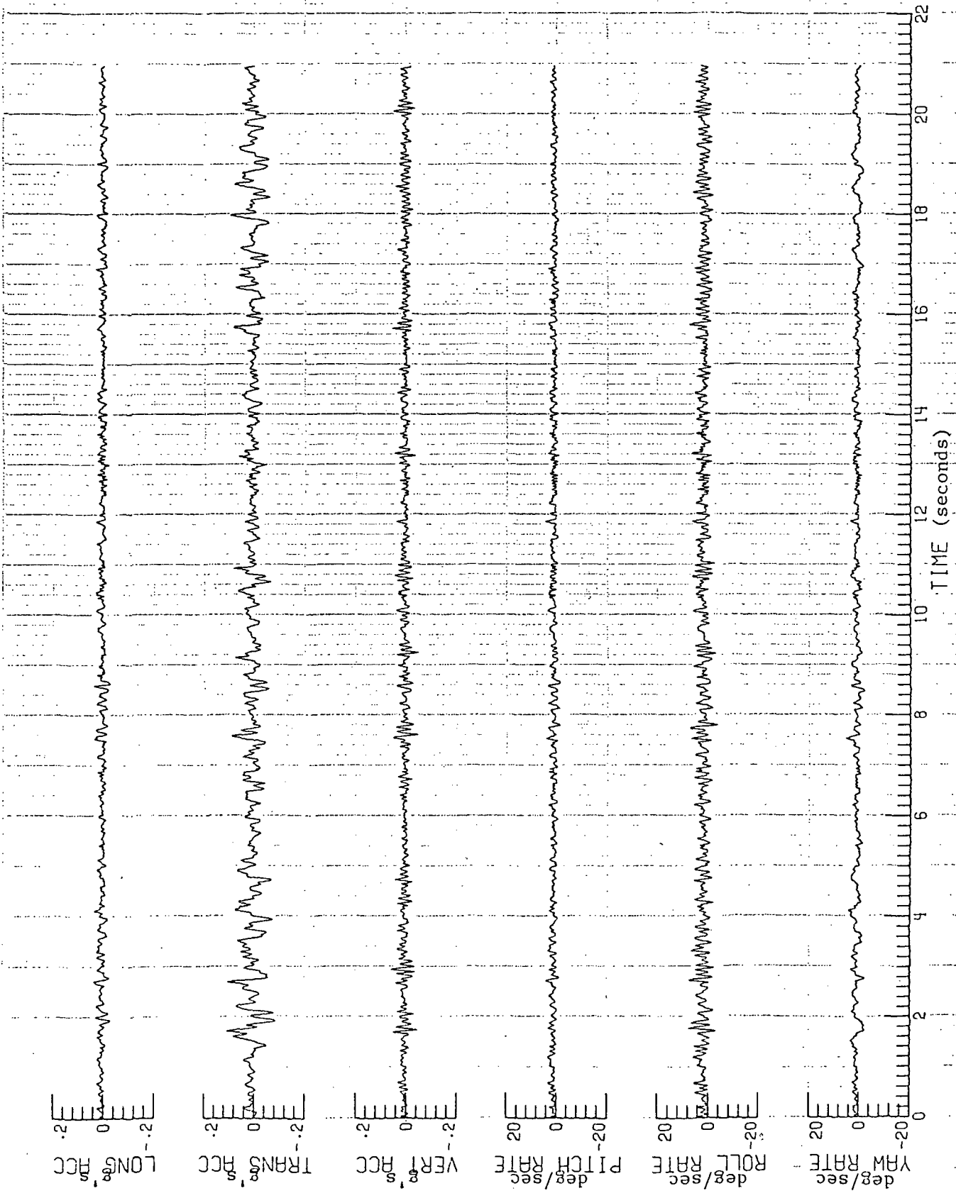
(a) Time histories (RMS yawing velocity 1.064 deg/sec)
