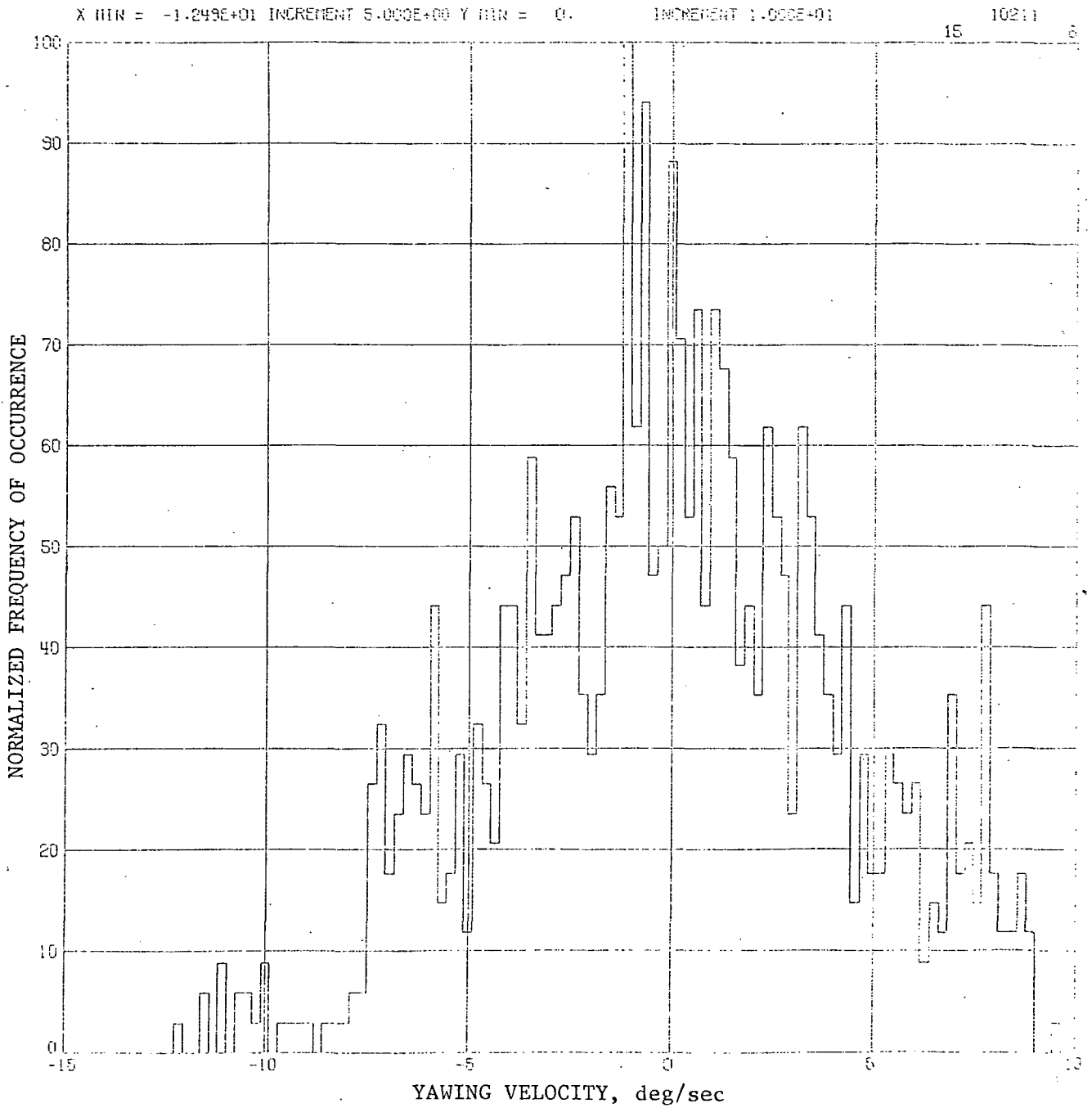
(b) Yawing velocity histogram (RMS yawing velocity 4.525 deg/sec)
