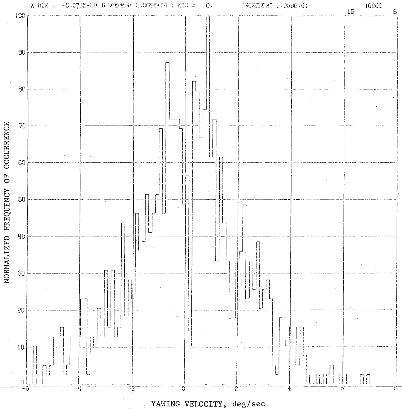
(b) Yawing velocity histograms (RMS yawing velocity 2.058 deg/sec)
