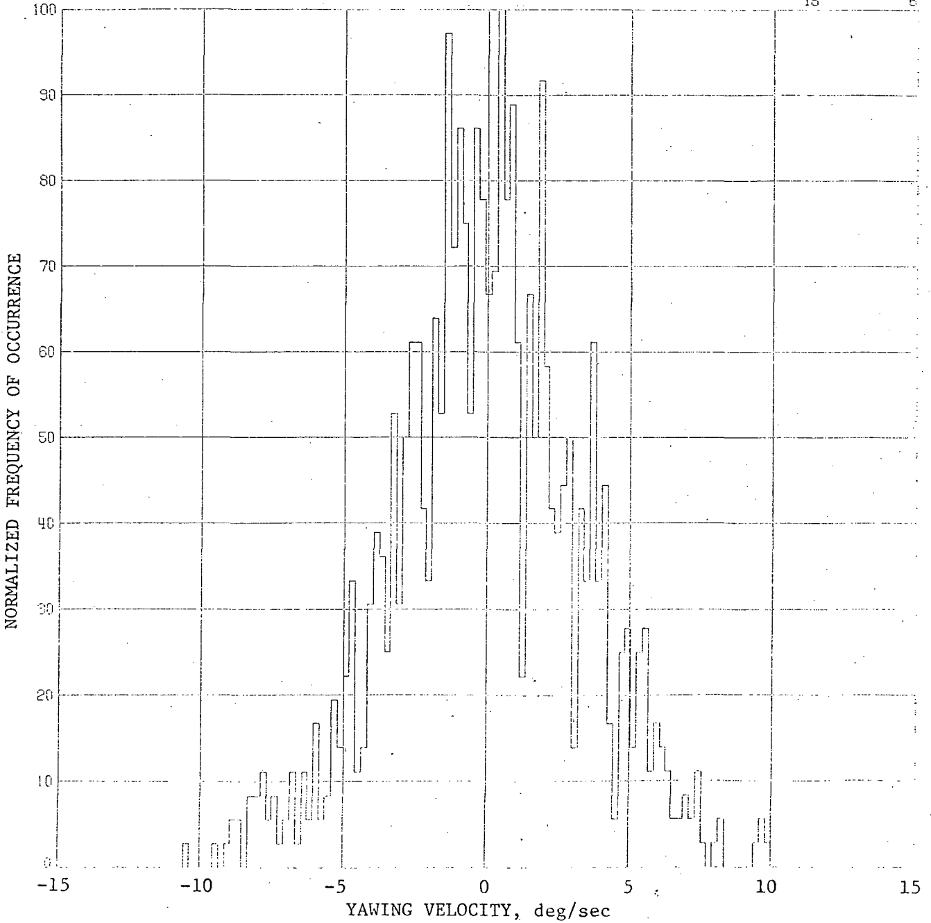
(b) Yawing velocity histograms (RMS yawing velocity 3.097 deg/sec)
