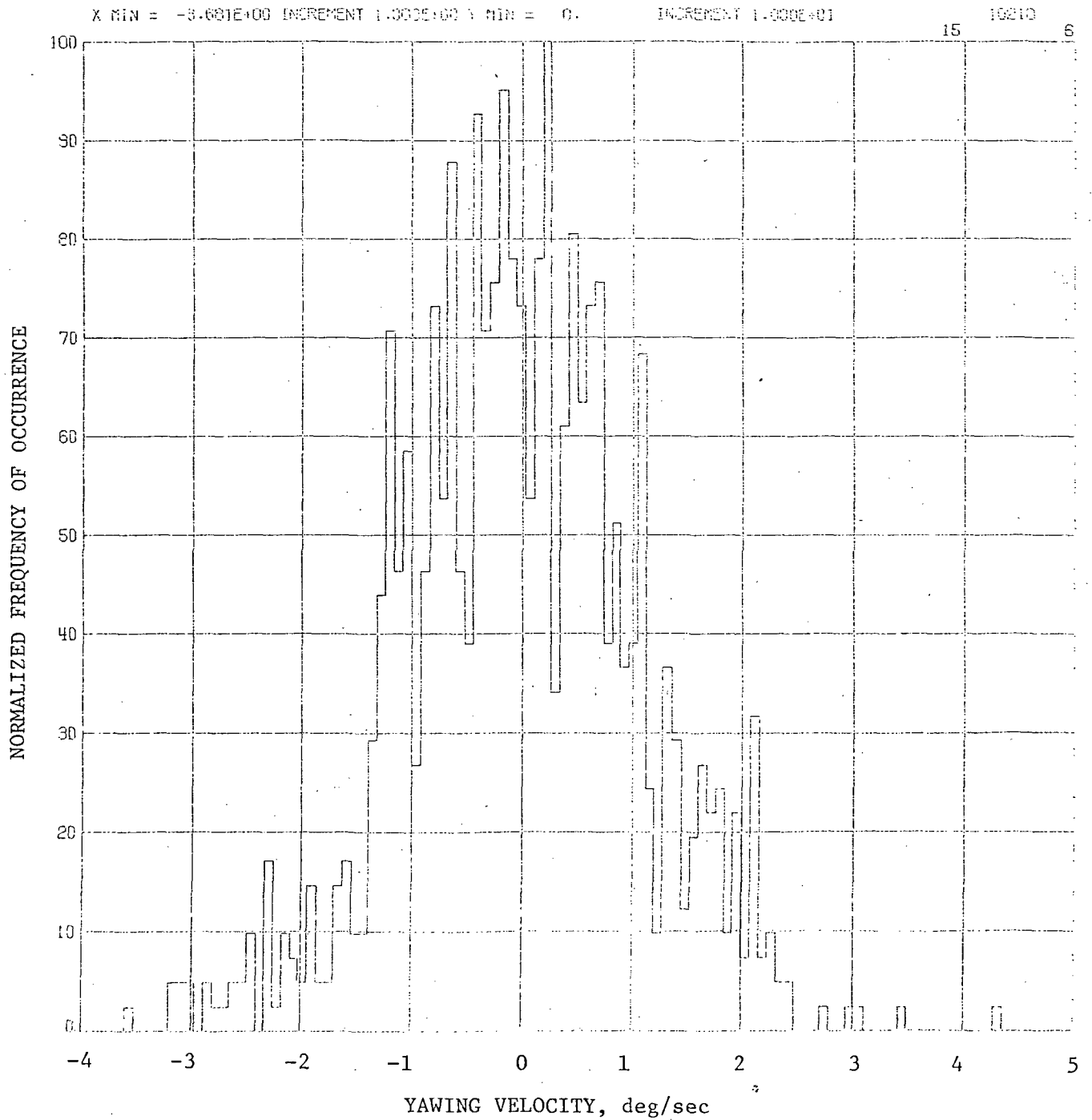
(b) Yawing velocity histograms (RMS yawing velocity 1.064 deg/sec)
