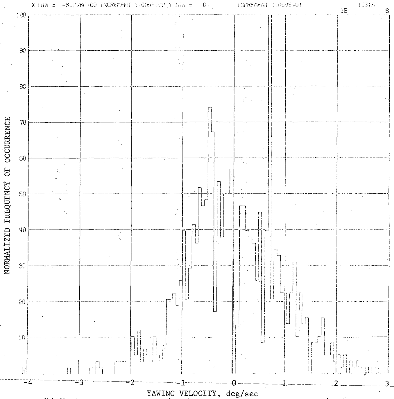
(b) Yawing velocity histograms (RMS yawing velocity 0.662 deg/sec)
