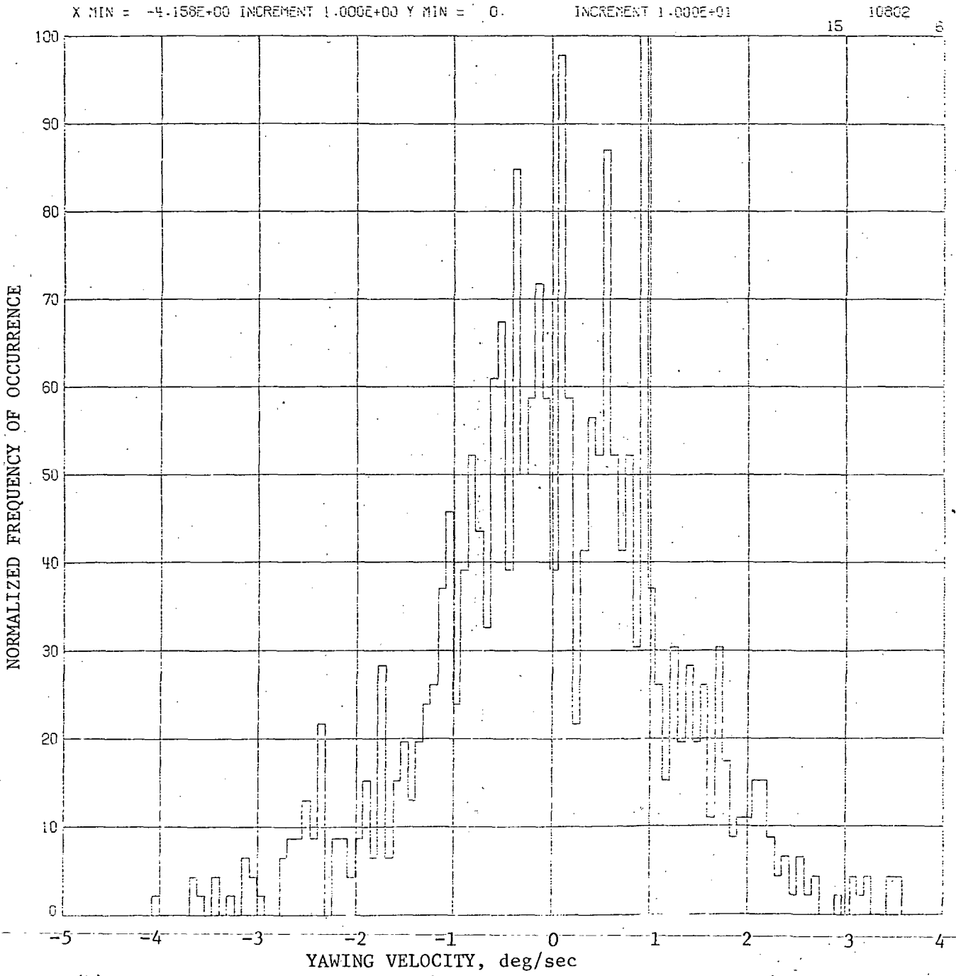
(b) Yawing velocity histograms (RMS yawing velocity 1.134 deg/sec)
