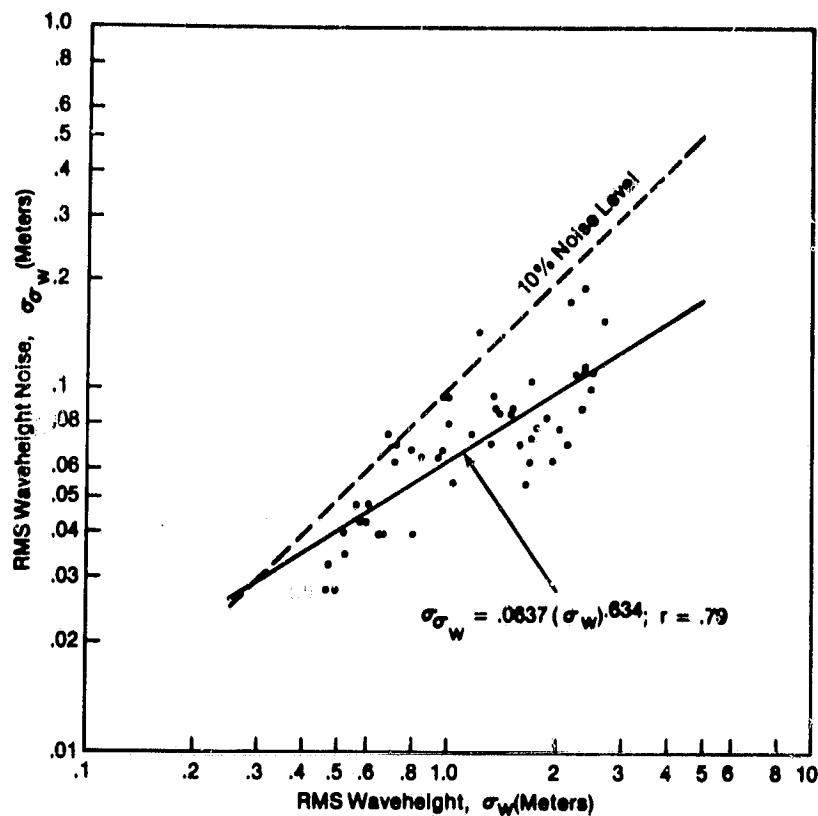
Figure 18. Significant wave height measurement noise level.
