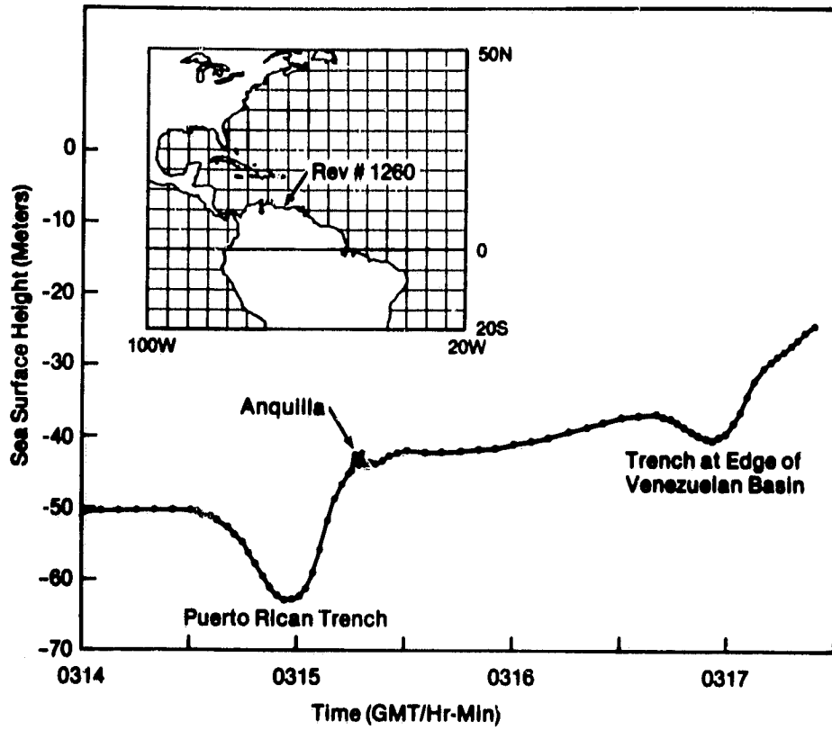
Figure 13. Sea surface height over trench type features.
