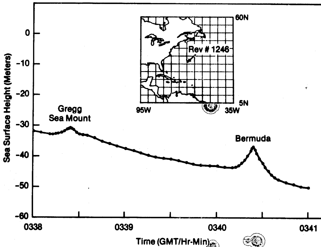
Figure 14. Sea surface height over sea mount type features.
