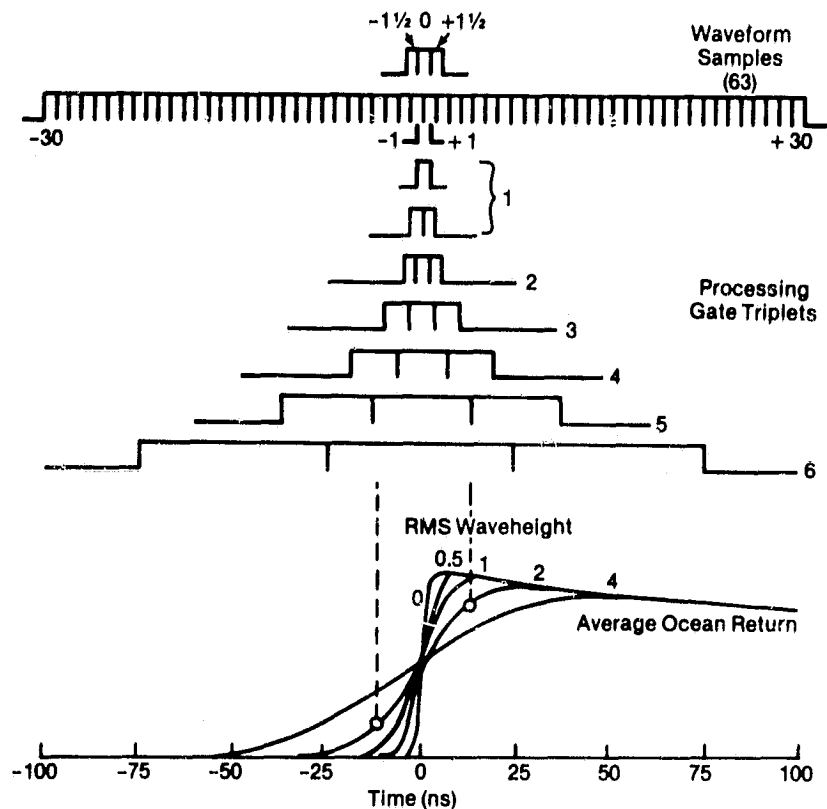
Figure 5. Formation of processing gates from waveform samples (ref. 8).
