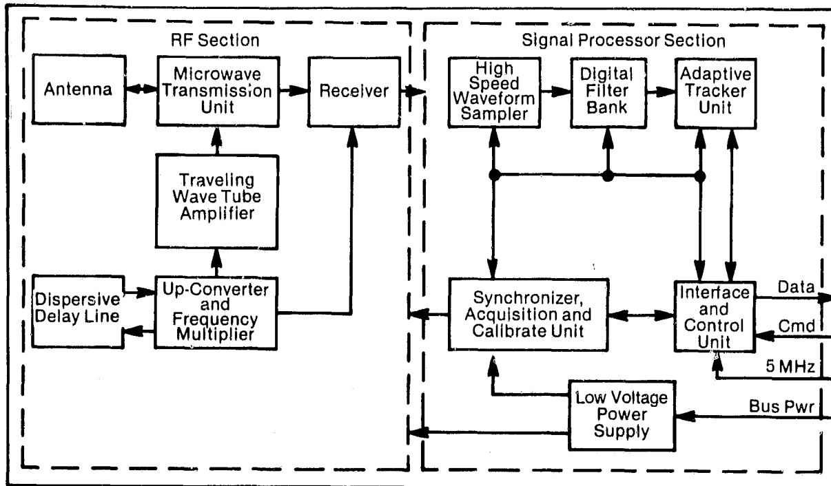
Figure 2. SEASAT-1 Radar Altimeter major functional elements (ref. 8).
