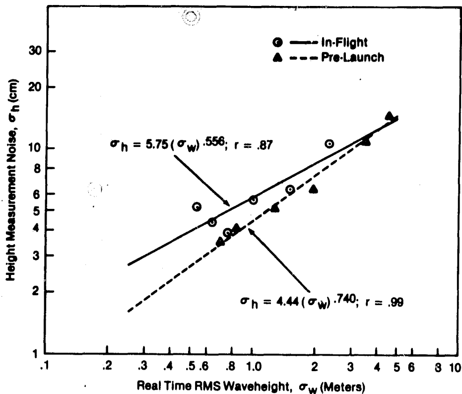
Figure 12. Height measurement performance (one second smoothing).
