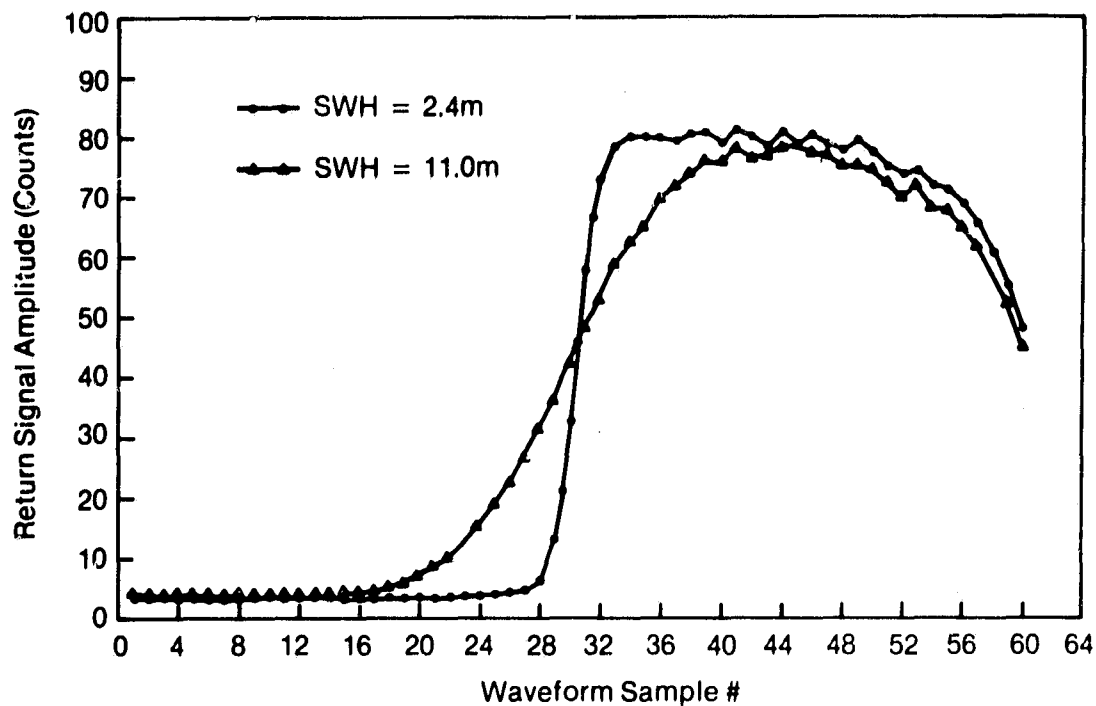
Figure 19. Return pulse shape as a function of SWH.
