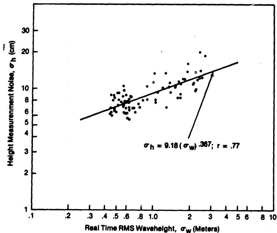
Figure 11. Height measurement performance (no smoothing).
