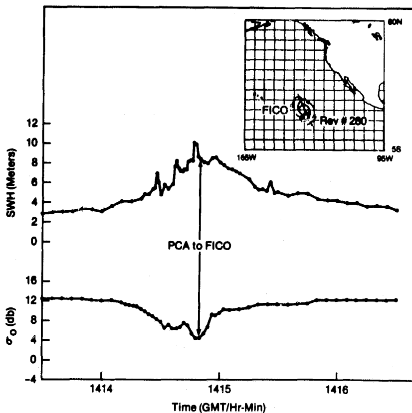
Figure 20. Altimeter measurements over Hurricane Fico.
