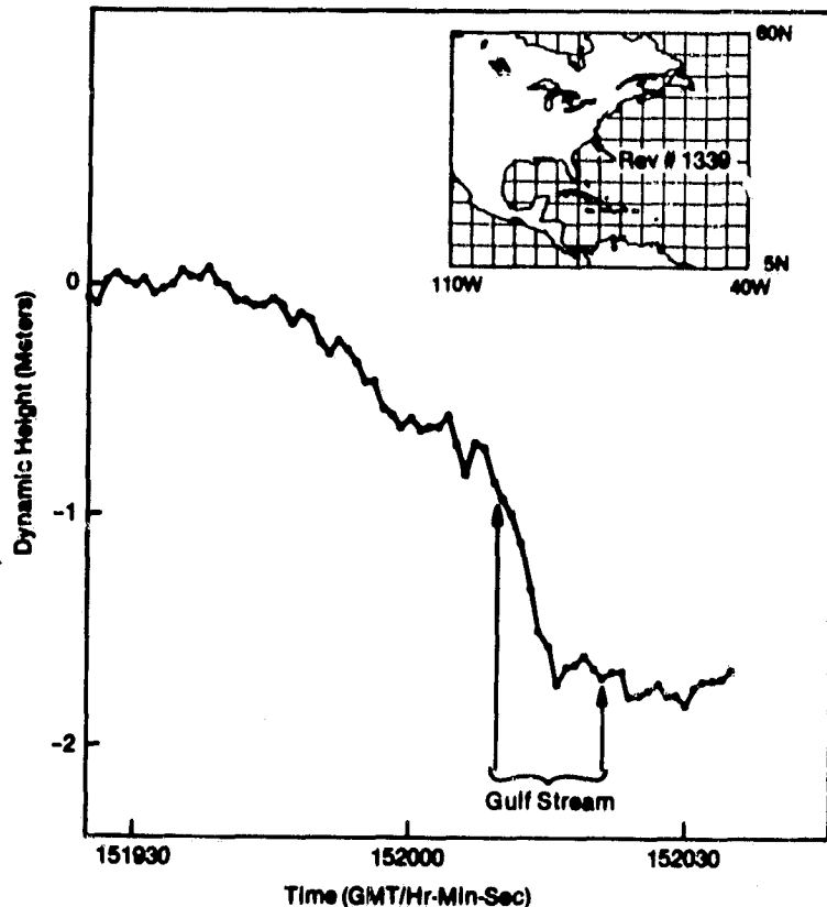
Figure 15. Dynamic height over Gulf Stream (ref. 14).
