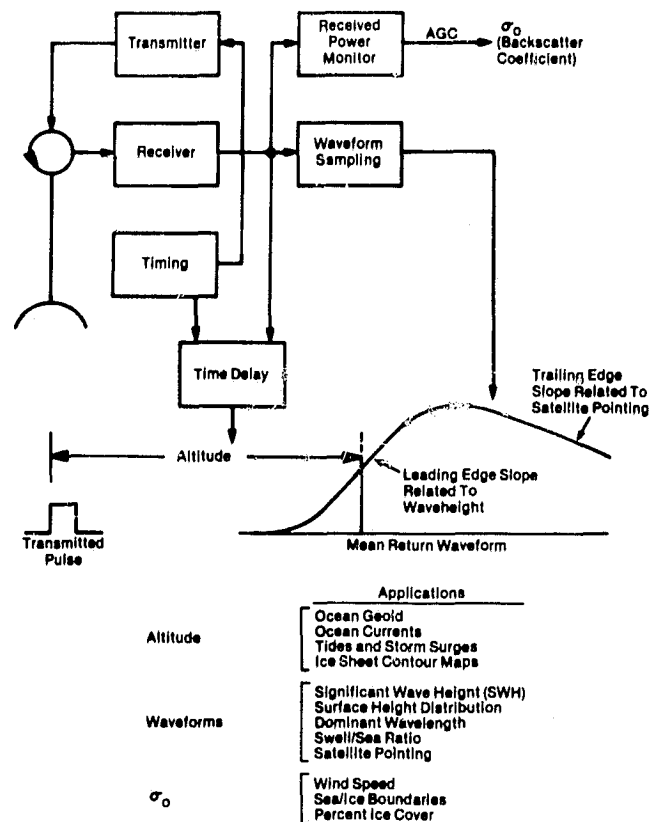
Figure 1. Block diagram depicting satellite altimetry concept and potential applications (ref. 3).
