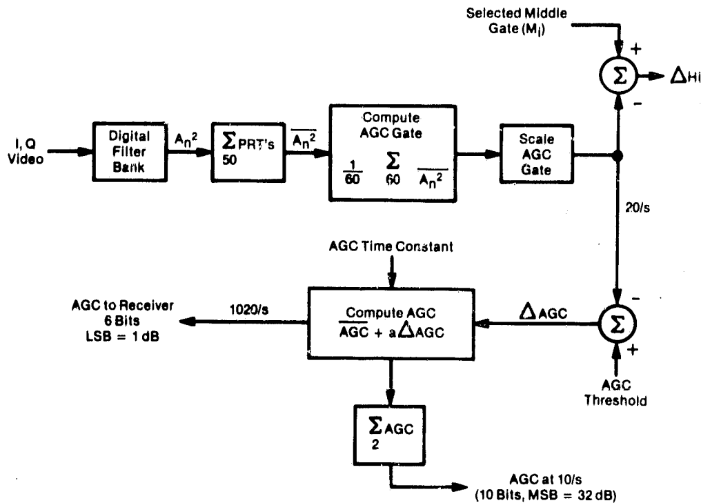
Figure 3. AGC processing flow (ref. 8).
