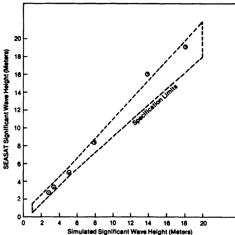
Figure 17. Significant wave height measurement performance (pre-launch).
