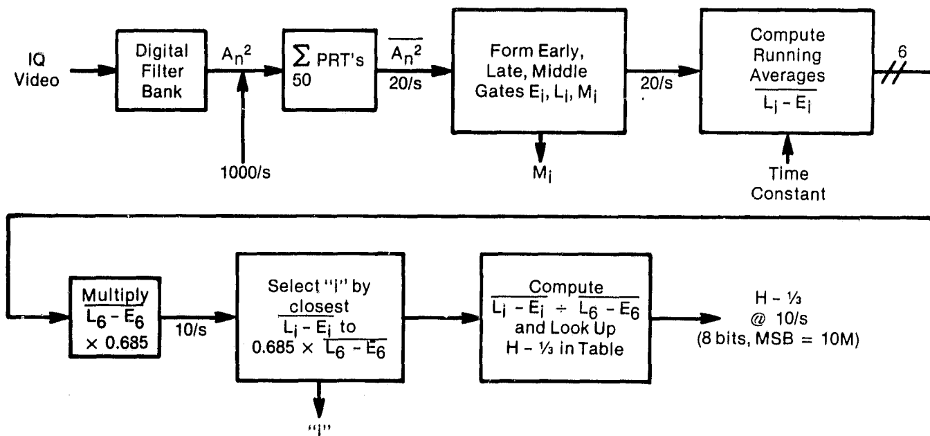
Figure 7. Wave height processing flow (ref. 8).
