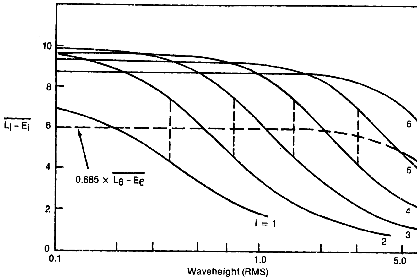
Figure 6. Wave height estimation (ref. 8).
