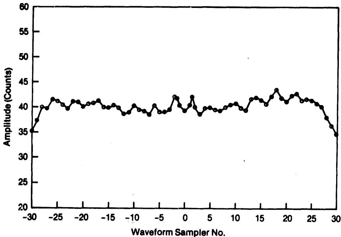
Figure 22. Calibrate mode II waveform calibration data.
