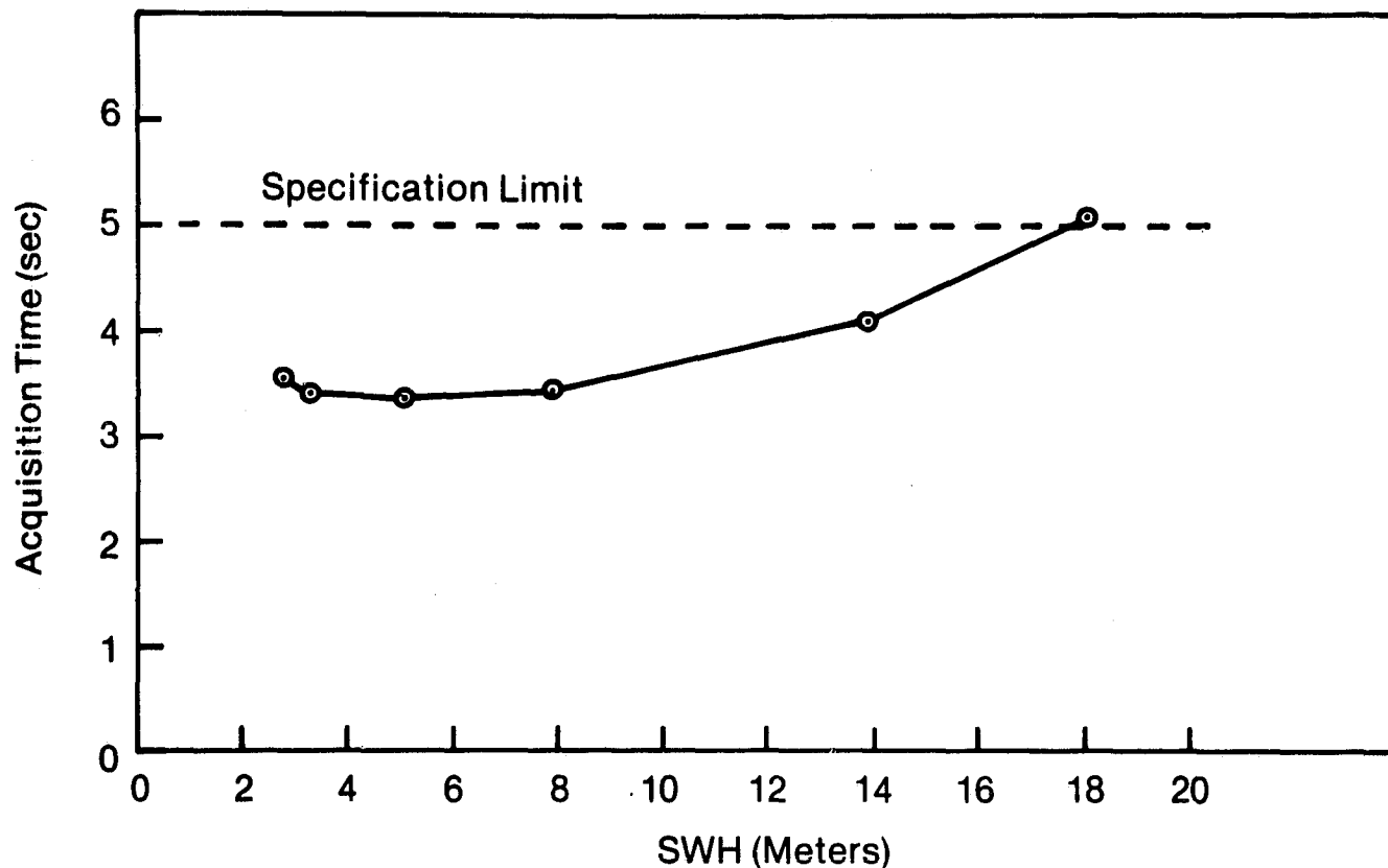
Figure 23. Acquisition time performance (pre-launch).
