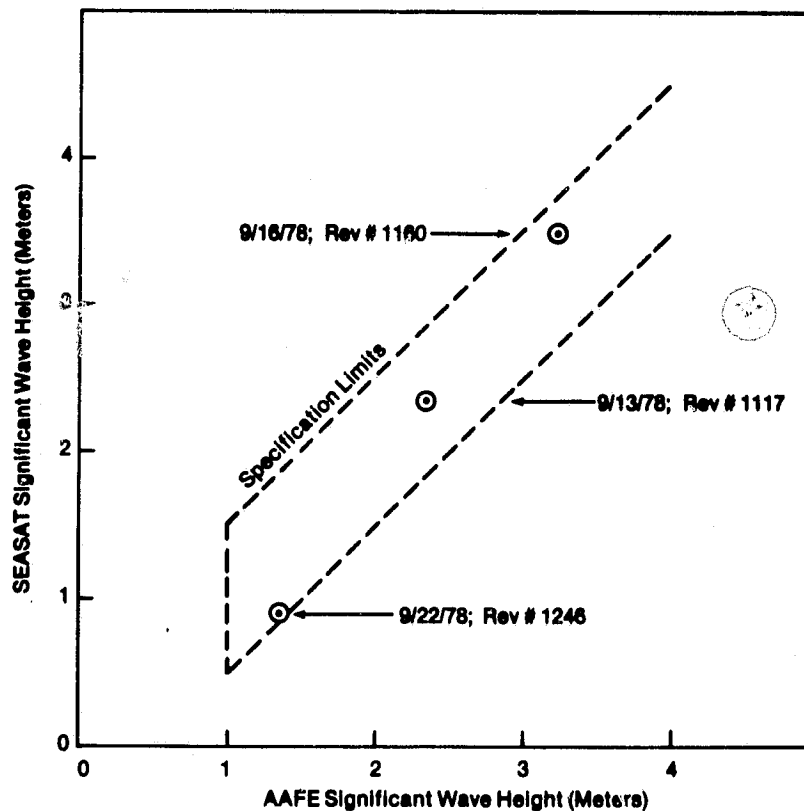
Figure 16. Significant wave height measurement performance at low SWH (< 4 m).
