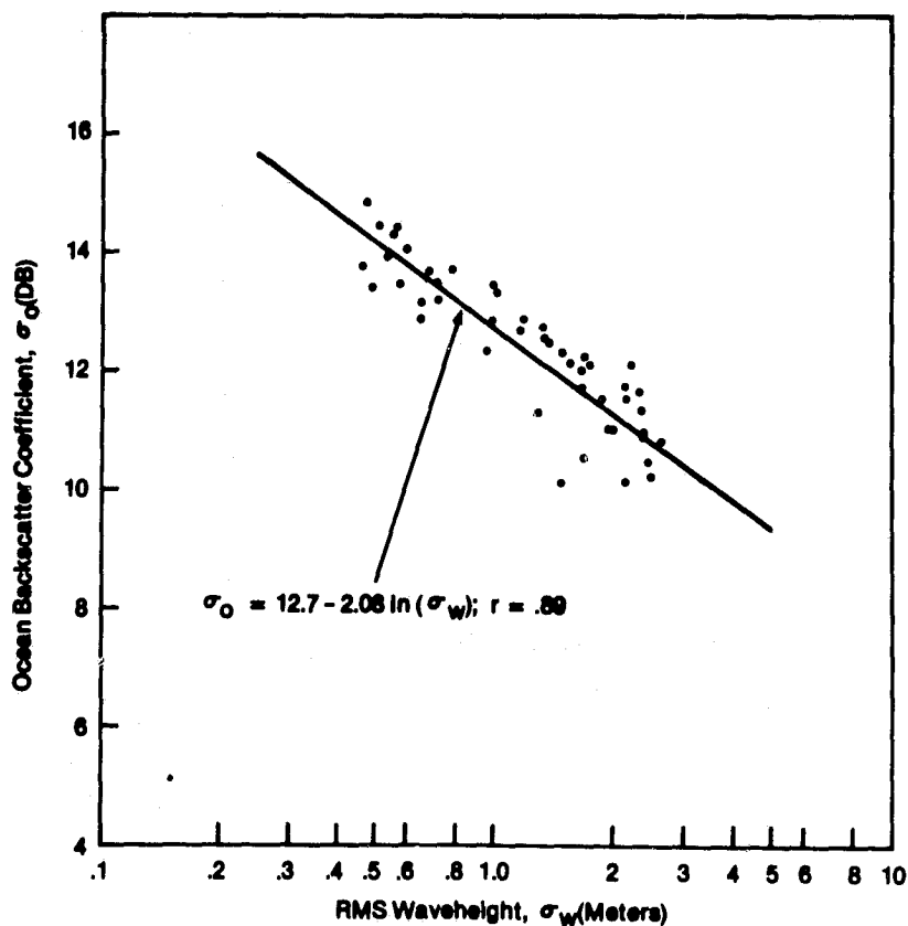
Figure 21. Ocean backscatter coefficient ( \sigma_0 ) measurement performance.
