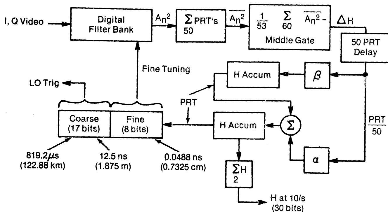
Figure 4. Height processing flow (ref. 8).
